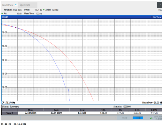
Band4-10MHz-16QAM-20175-50RB#0
