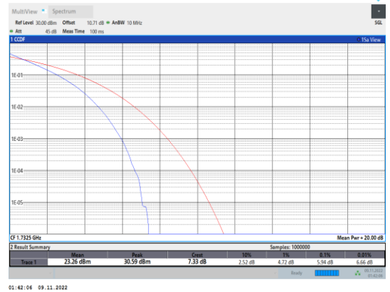
Band4-10MHz-QPSK-20175-50RB#0
