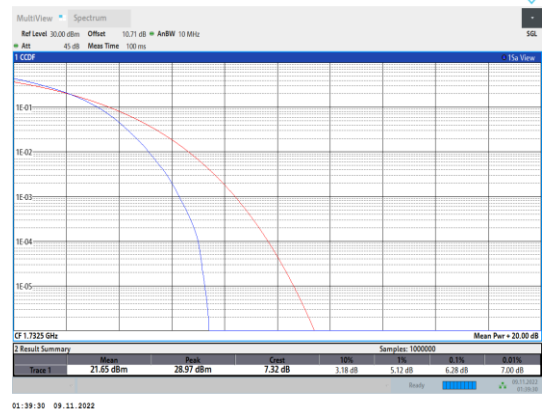
Band4-15MHz-16QAM-20175-75RB#0
