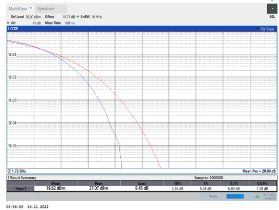
Band4-20MHz-64QAM-20050-100RB#0
