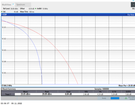
Band5-5MHz-QPSK-20625-25RB#0
