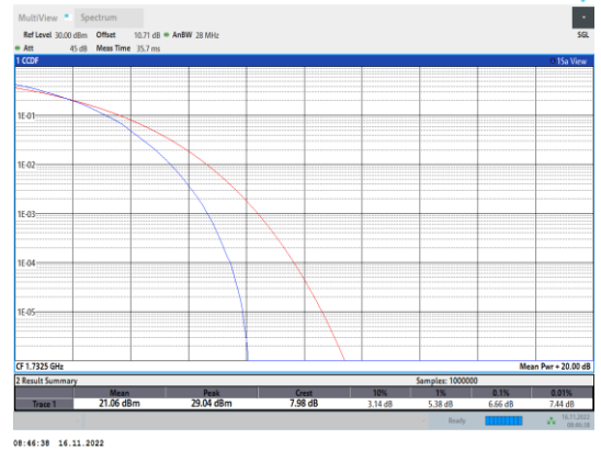
Band4-3MHz-64QAM-20175-15RB#0
