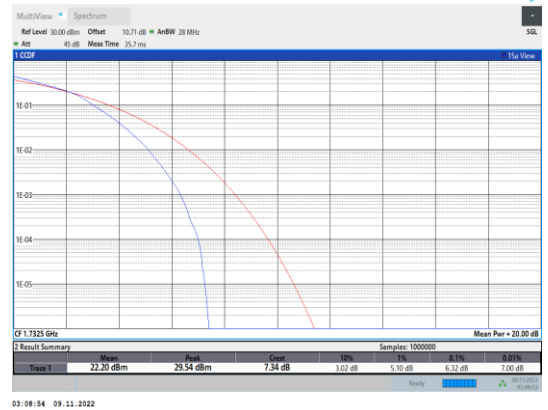
Band4-1.4MHz-16QAM-20175-6RB#0
