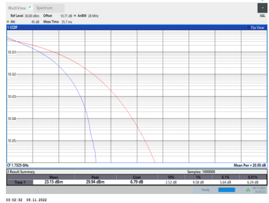
Band4-3MHz-QPSK-20175-15RB#0
