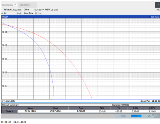
Band4-1.4MHz-QPSK-20175-6RB#0
