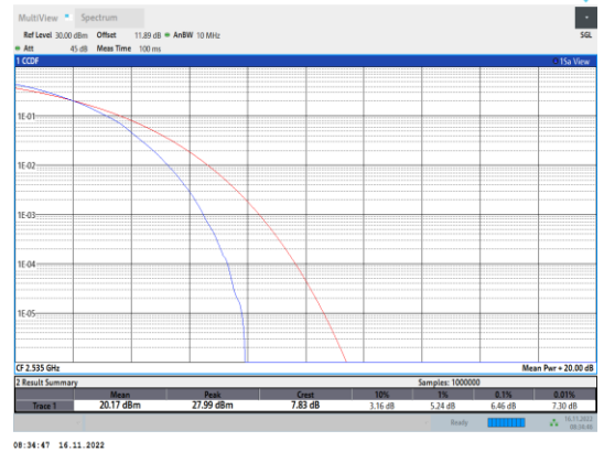
Band7-10MHz-64QAM-21100-50RB#0
