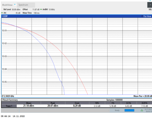
Band7-5MHz-64QAM-20775-25RB#0
