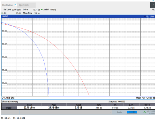
Band4-15MHz-QPSK-20025-75RB#0
