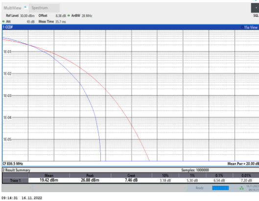
Band5-1.4MHz-64QAM-20525-6RB#0
