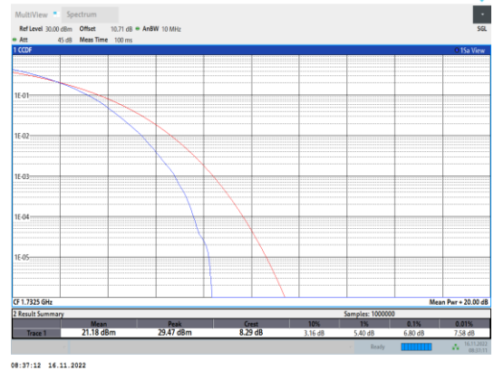
Band4-10MHz-64QAM-20175-50RB#0
