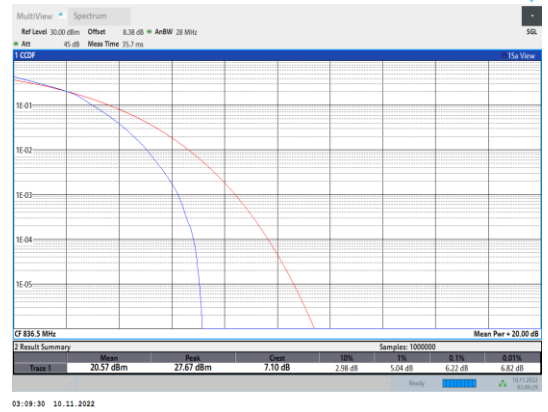
Band5-1.4MHz-16QAM-20525-6RB#0
