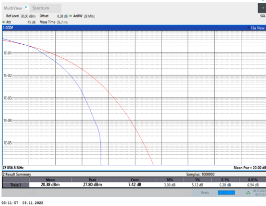
Band5-3MHz-16QAM-20525-15RB#0
