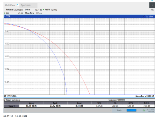
Band4-20MHz-64QAM-20175-100RB#0
