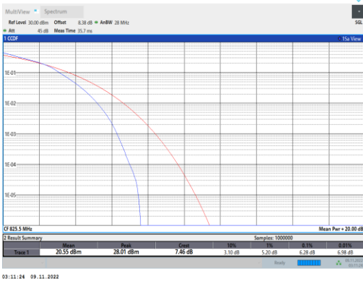
Band5-3MHz-16QAM-20415-15RB#0
