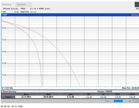
Band4-1.4MHz-QPSK-19957-6RB#0
