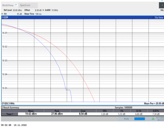
Band5-5MHz-64QAM-20425-25RB#0
