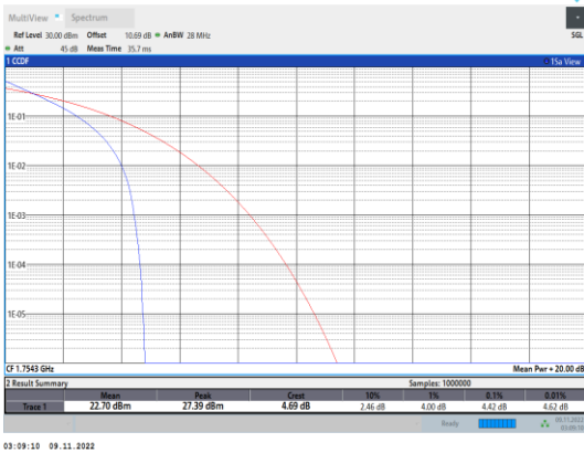
Band4-1.4MHz-QPSK-20393-6RB#0
