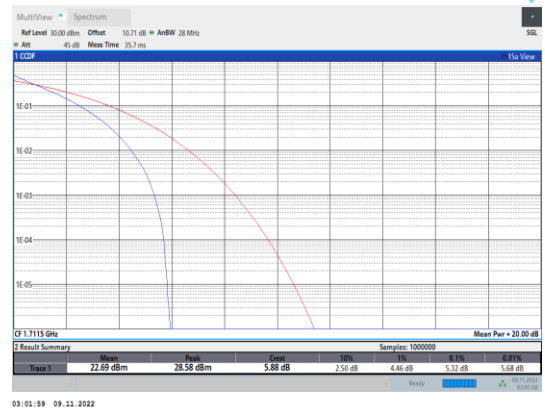
Band4-3MHz-QPSK-19965-15RB#0
