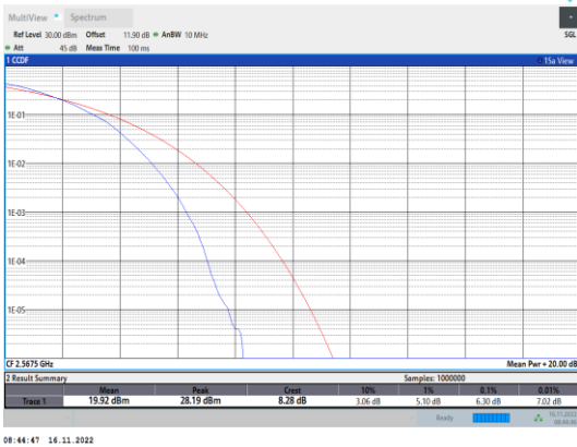
Band7-5MHz-64QAM-21425-25RB#0
