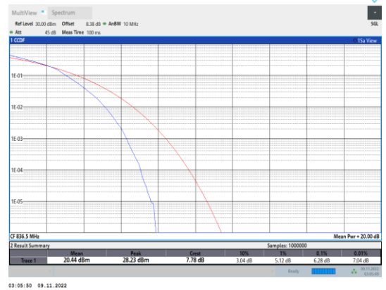
Band5-5MHz-16QAM-20525-25RB#0
