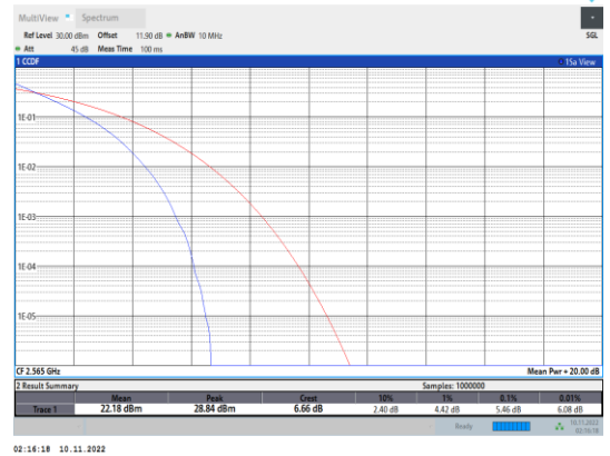
Band7-10MHz-QPSK-21400-50RB#0
