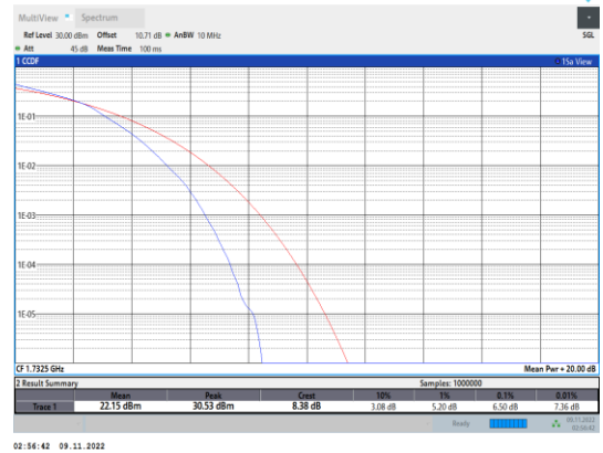
Band4-5MHz-16QAM-20175-25RB#0
