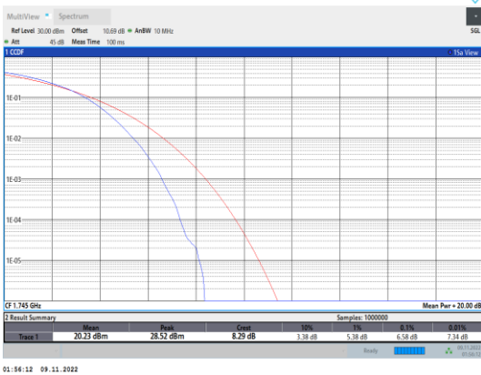
Band4-20MHz-16QAM-20300-100RB#0
