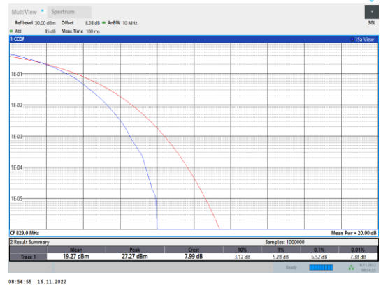
Band5-10MHz-64QAM-20450-50RB#0
