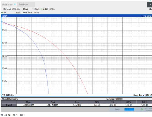
Band7-5MHz-QPSK-21425-25RB#0
