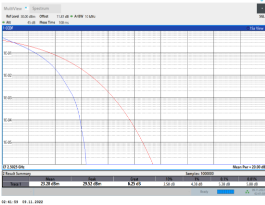
Band7-5MHz-QPSK-20775-25RB#0
