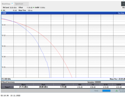
Band7-10MHz-16QAM-21400-50RB#0
