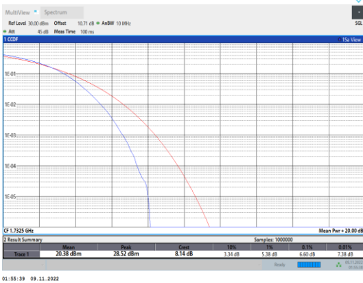
Band4-20MHz-16QAM-20175-100RB#0
