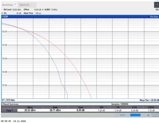
Band4-15MHz-64QAM-20325-75RB#0
