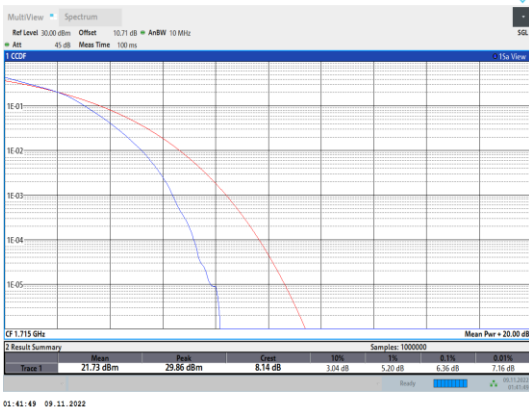
Band4-10MHz-16QAM-20000-50RB#0
