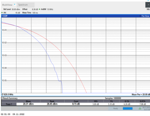
Band5-10MHz-16QAM-20450-50RB#0
