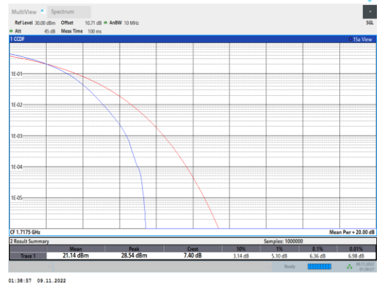
Band4-15MHz-16QAM-20025-75RB#0
