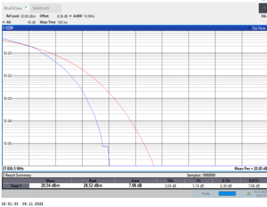
Band5-10MHz-16QAM-20525-50RB#0
