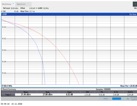
Band5-1.4MHz-QPSK-20525-6RB#0
