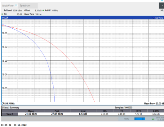
Band5-5MHz-QPSK-20525-25RB#0
