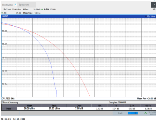
Band4-5MHz-64QAM-20375-25RB#0
