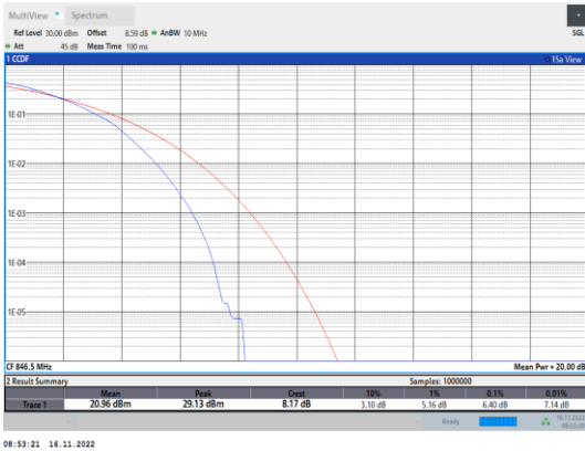
Band5-5MHz-64QAM-20625-25RB#0
