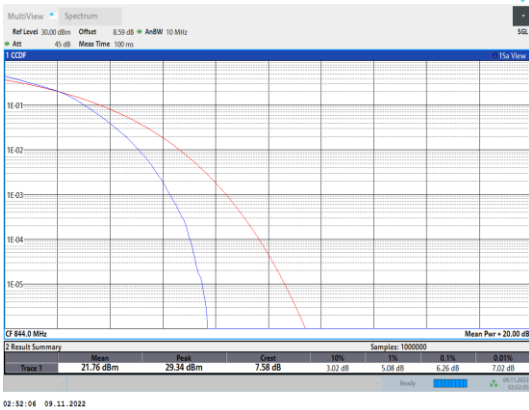
Band5-10MHz-16QAM-20600-50RB#0
