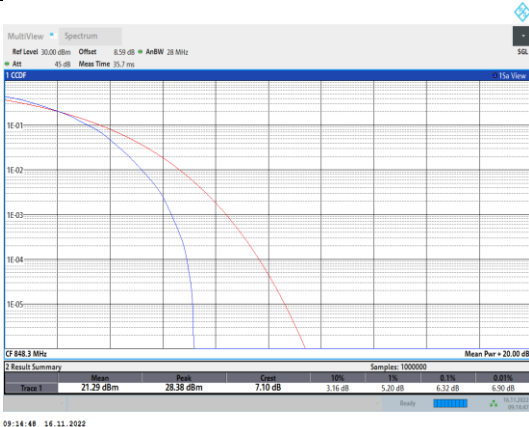
Band5-1.4MHz-64QAM-20643-6RB#0
