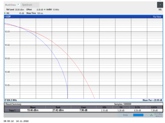
Band5-10MHz-64QAM-20525-50RB#0
