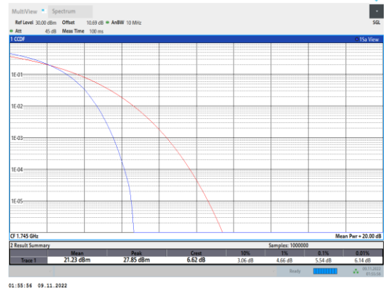
Band4-20MHz-QPSK-20300-100RB#0
