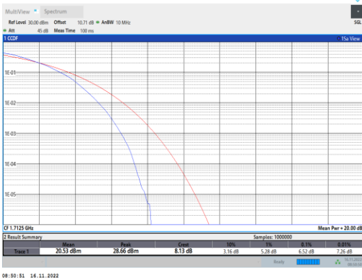
Band4-5MHz-64QAM-19975-25RB#0
