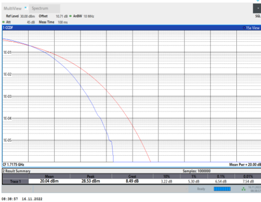
Band4-15MHz-64QAM-20025-75RB#0
