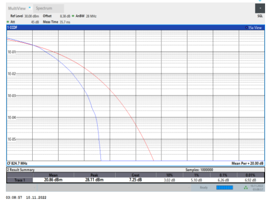
Band5-1.4MHz-16QAM-20407-6RB#0
