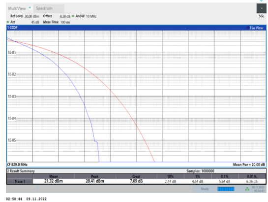
Band5-10MHz-QPSK-20450-50RB#0
