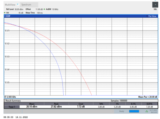
Band7-10MHz-64QAM-21400-50RB#0
