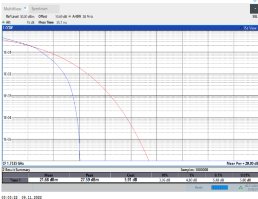
Band4-3MHz-16QAM-20385-15RB#0
