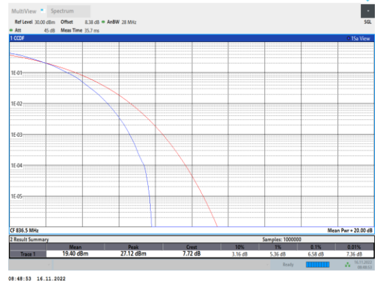
Band5-3MHz-64QAM-20525-15RB#0
