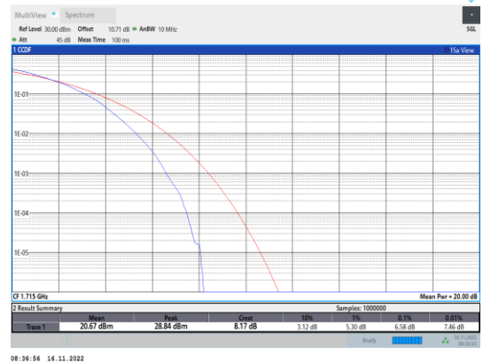
Band4-10MHz-64QAM-20000-50RB#0
