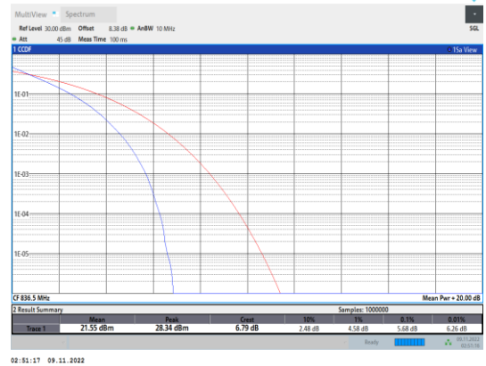
Band5-10MHz-QPSK-20525-50RB#0
