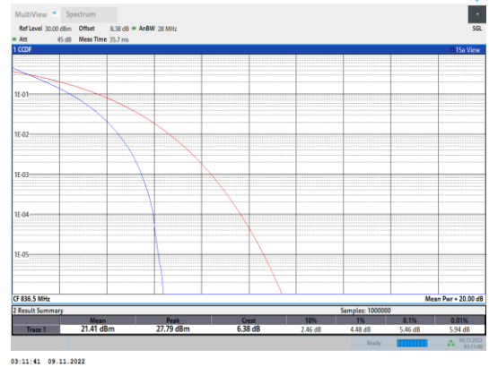
Band5-3MHz-QPSK-20525-15RB#0
