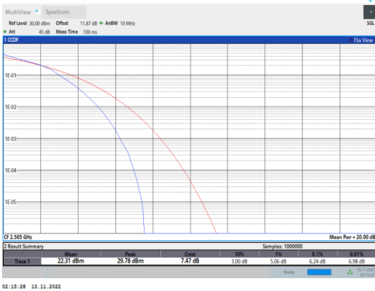
Band7-10MHz-16QAM-20800-50RB#0
