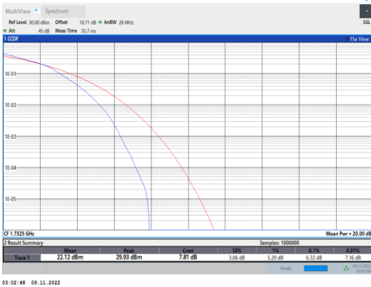
Band4-3MHz-16QAM-20175-15RB#0
