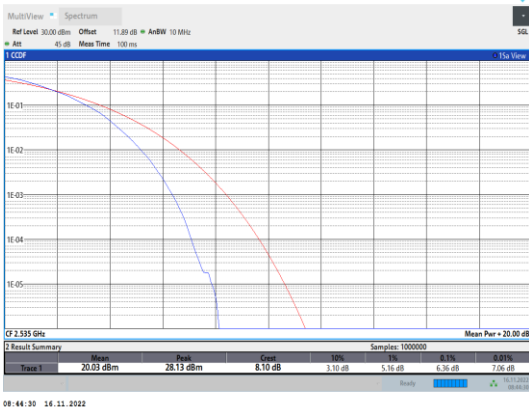
Band7-5MHz-64QAM-21100-25RB#0
