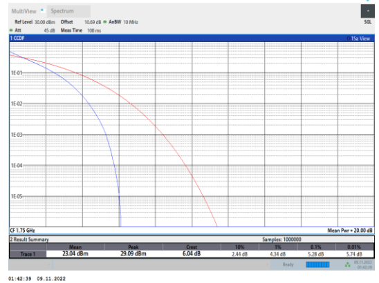
Band4-10MHz-QPSK-20350-50RB#0
