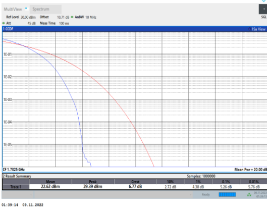
Band4-15MHz-QPSK-20175-75RB#0
