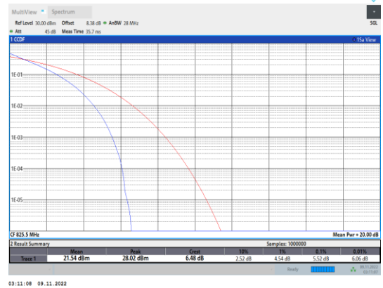
Band5-3MHz-QPSK-20415-15RB#0
