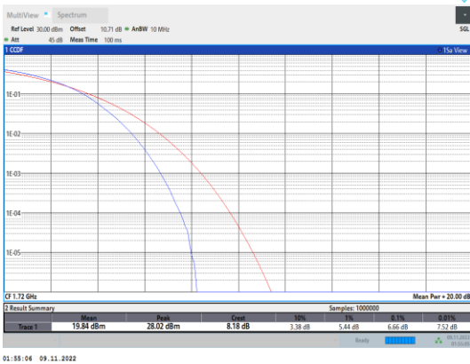
Band4-20MHz-16QAM-20050-100RB#0
