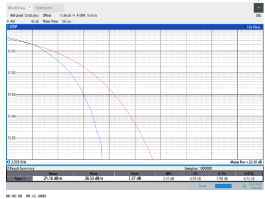
Band7-5MHz-16QAM-21100-25RB#0
