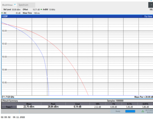
Band4-5MHz-QPSK-19975-25RB#0
