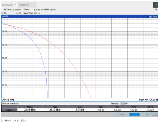
Band5-1.4MHz-QPSK-20643-6RB#0
