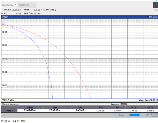
Band5-5MHz-QPSK-20425-25RB#0
