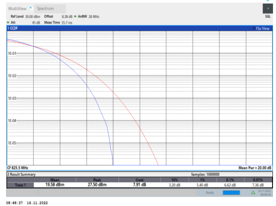
Band5-3MHz-64QAM-20415-15RB#0
