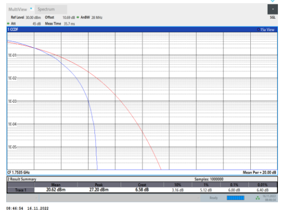
Band4-3MHz-64QAM-20385-15RB#0
