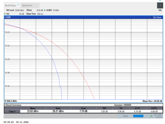
Band5-5MHz-16QAM-20625-25RB#0
