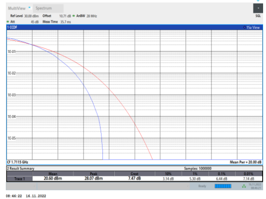
Band4-3MHz-64QAM-19965-15RB#0
