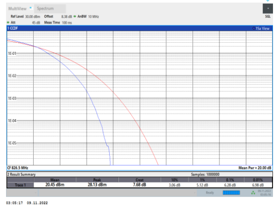
Band5-5MHz-16QAM-20425-25RB#0
