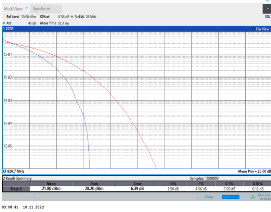
Band5-1.4MHz-QPSK-20407-6RB#0
