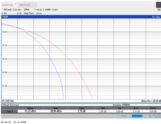
Band7-10MHz-16QAM-21100-50RB#0
