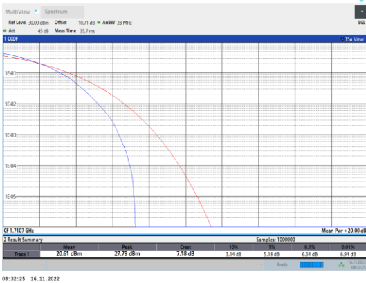
Band4-1.4MHz-64QAM-19957-6RB#0
