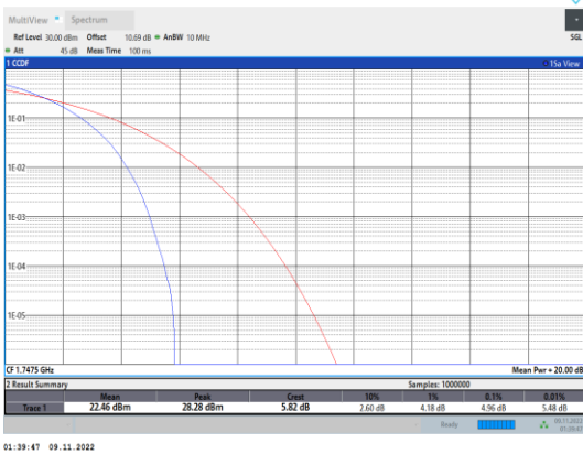
Band4-15MHz-QPSK-20325-75RB#0
