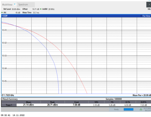
Band4-1.4MHz-64QAM-20175-6RB#0
