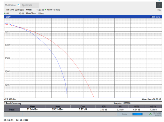
Band7-10MHz-64QAM-20800-50RB#0
