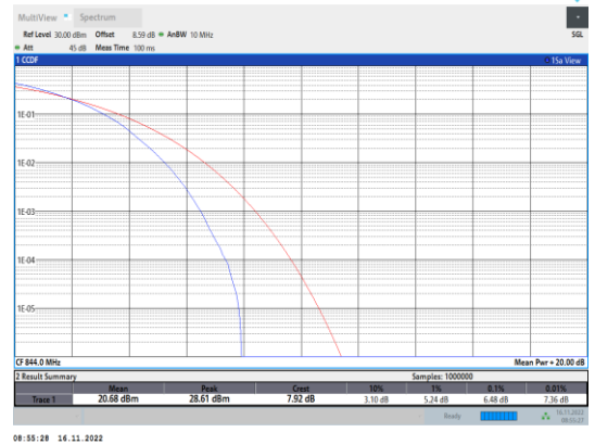
Band5-10MHz-64QAM-20600-50RB#0
