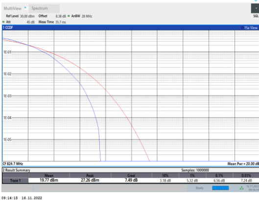
Band5-1.4MHz-64QAM-20407-6RB#0
