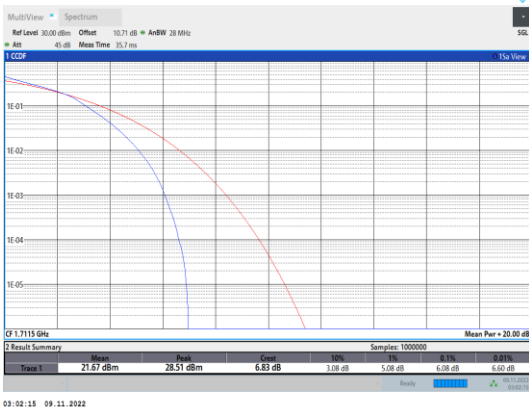
Band4-3MHz-16QAM-19965-15RB#0
