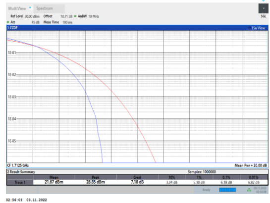
Band4-5MHz-16QAM-19975-25RB#0
