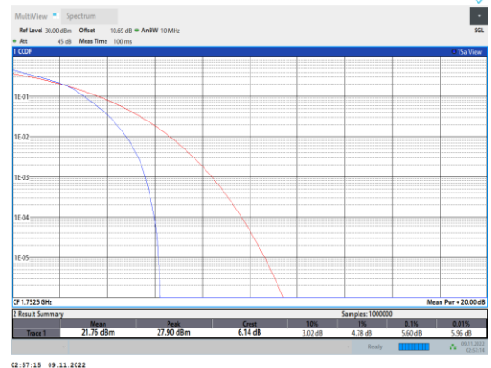
Band4-5MHz-16QAM-20375-25RB#0
