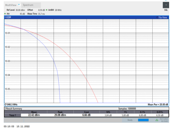
Band5-1.4MHz-16QAM-20643-6RB#0
