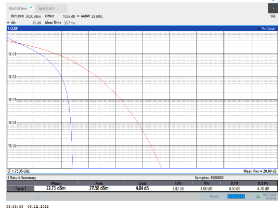
Band4-3MHz-QPSK-20385-15RB#0
