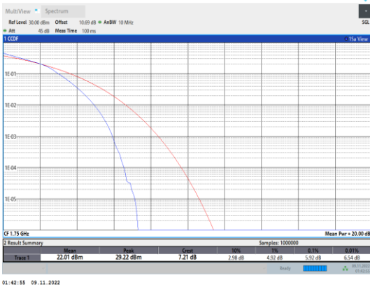
Band4-10MHz-16QAM-20350-50RB#0
