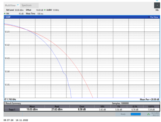
Band4-20MHz-64QAM-20300-100RB#0
