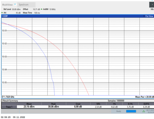
Band4-5MHz-QPSK-20175-25RB#0
