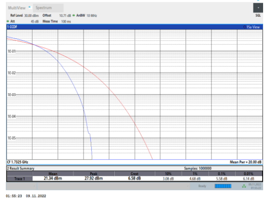
Band4-20MHz-QPSK-20175-100RB#0
