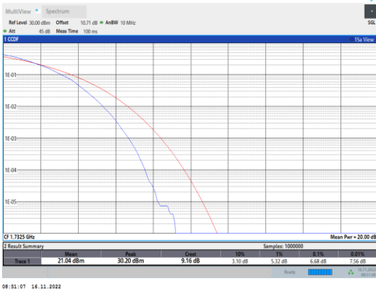
Band4-5MHz-64QAM-20175-25RB#0
