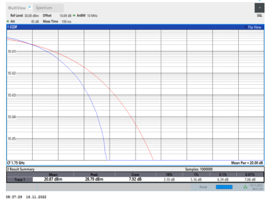
Band4-10MHz-64QAM-20350-50RB#0
