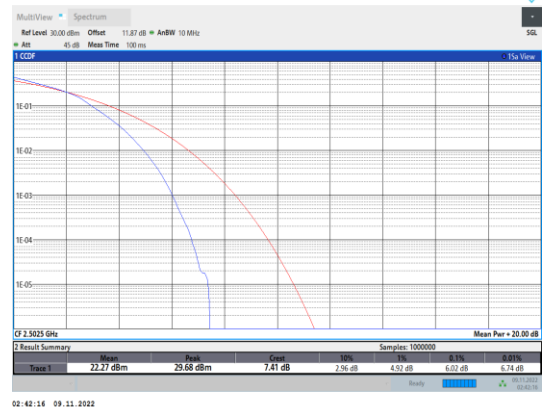
Band7-5MHz-16QAM-20775-25RB#0
