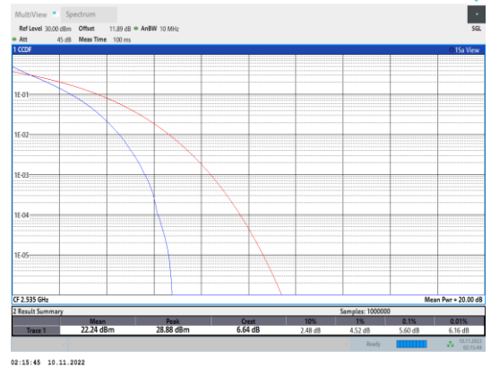
Band7-10MHz-QPSK-21100-50RB#0
