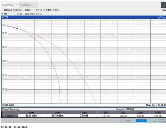
Band5-3MHz-16QAM-20635-15RB#0
