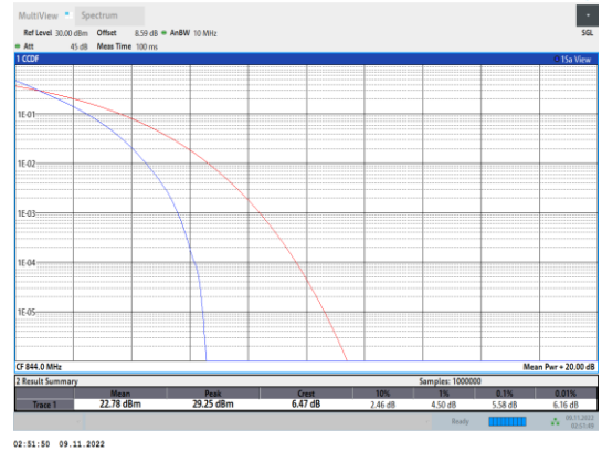
Band5-10MHz-QPSK-20600-50RB#0
