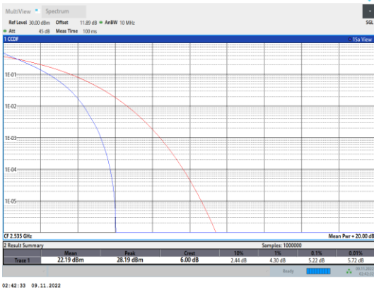
Band7-5MHz-QPSK-21100-25RB#0
