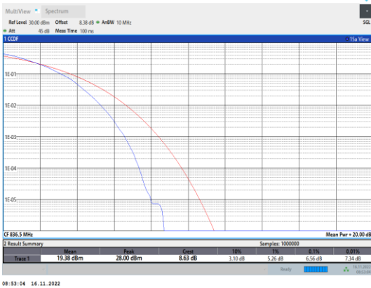
Band5-5MHz-64QAM-20525-25RB#0
