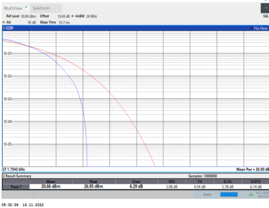
Band4-1.4MHz-64QAM-20393-6RB#0
