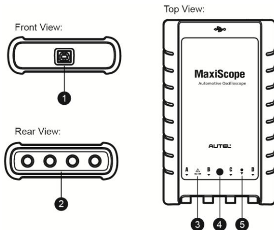
Figure 16-3 Front, Rear, and Top View
