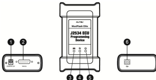
Figure 2-6 J2534 ECU Programming Device – for MaxiSys MS908S Pro
