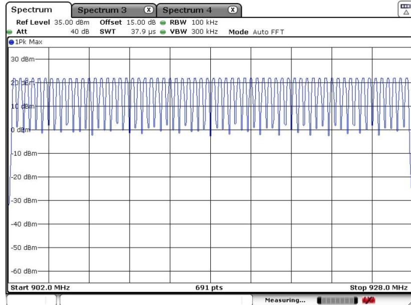
Number of Hopping Channel Plot (Data Rate 150kbps)
