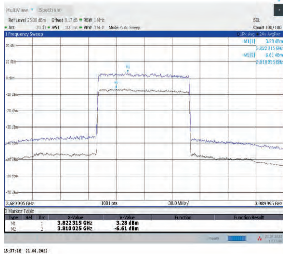
1-N77-3700-3980--30-100-M-1-DFT-256QAM-Outer_Full-270@0-Ant1-9.89-100%-0.00-9.89-PASS-≤13
