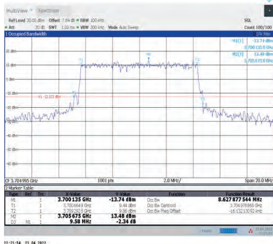
1-N77-3700-3980--30-10-L-1-DFT-QPSK-Outter_Full -24@0-Ant1-8.628-9.580-≤10-PASS
