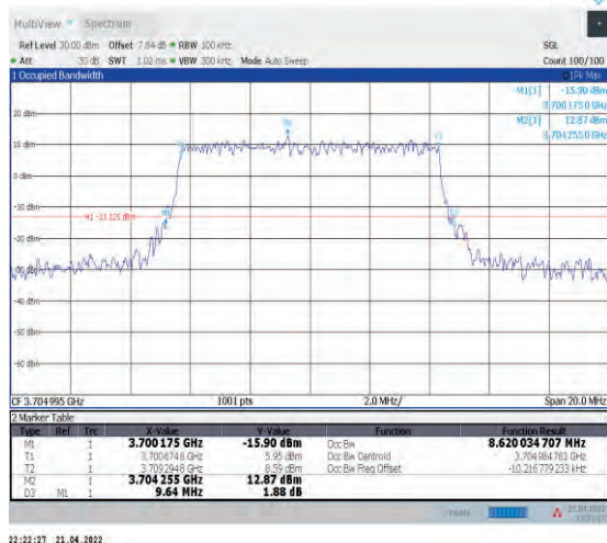
1-N77-3700-3980--30-10-L-3-DFT-16QAM-Outter_Full -24@0-Ant1-8.62-9.640-≤10-PASS
