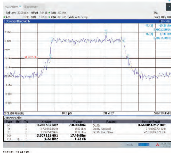
1-N77-3700-3980--30-10-L-2-DFT-PI2BPSK-Outter_Full -24@0-Ant1-8.569-9.220-≤10-PASS
