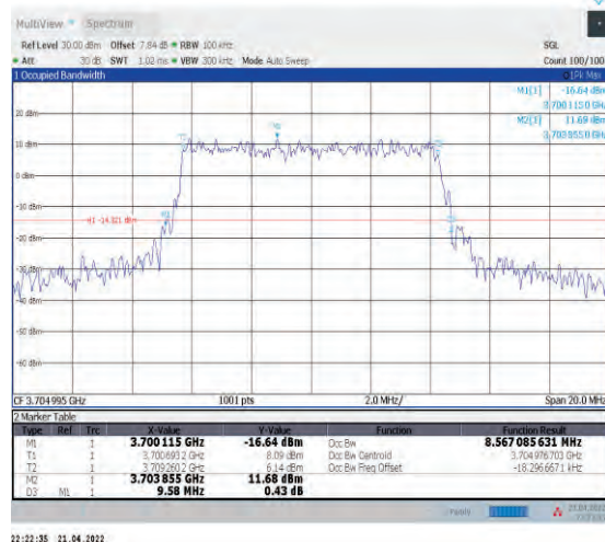
1-N77-3700-3980--30-10-L-4-DFT-64QAM-Outter_Full -24@0-Ant1-8.567-9.580-≤10-PASS
