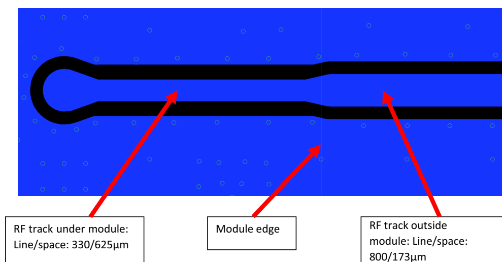
Figure 19: Routing Detail
