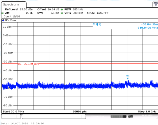
11N40MIMO-Ant1-2452-30~1000-PASS
