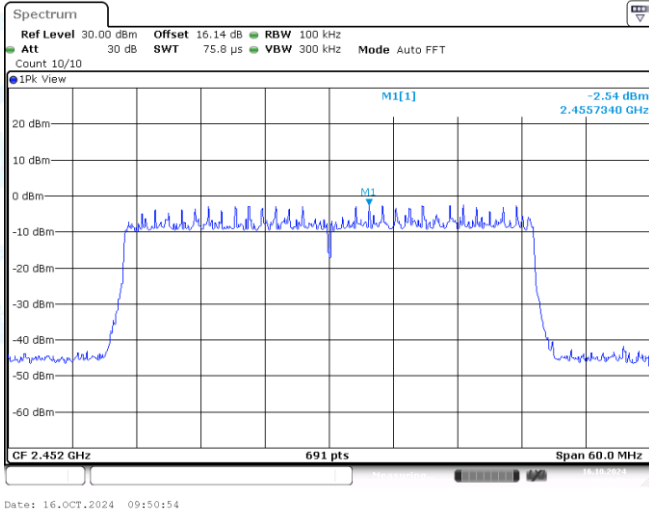
11AX40MIMO-Ant1-2452-0~Reference-PASS
