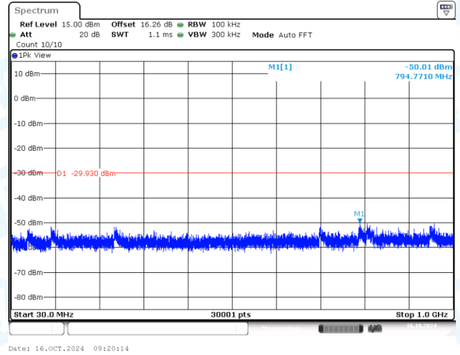
11AX20MIMO-Ant2-2412-30~1000-PASS
