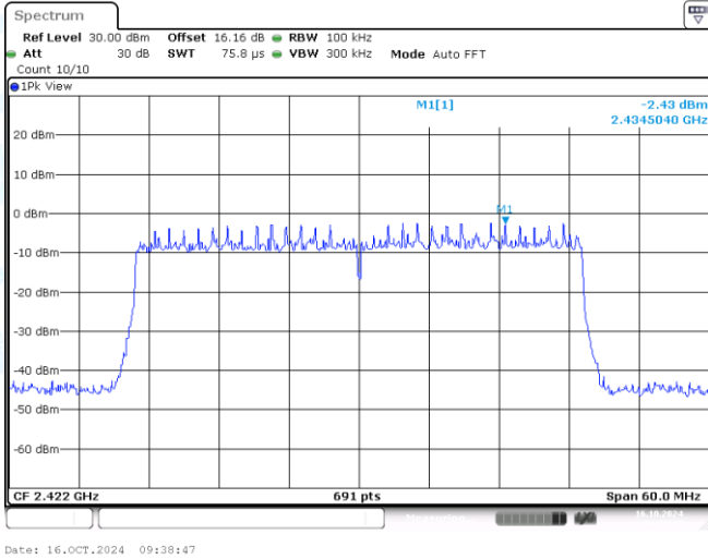
11AX40MIMO-Ant1-2422-0~Reference-PASS
