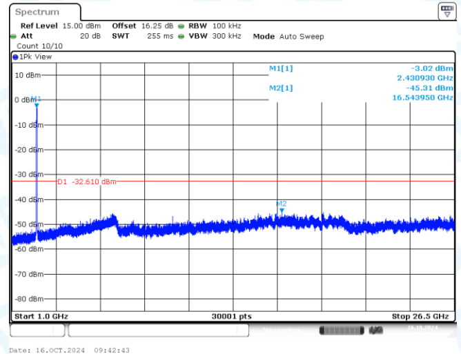
11AX40MIMO-Ant2-2422-1000~26500-PASS
