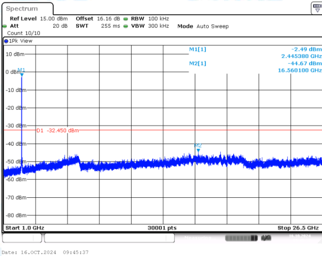
11AX40MIMO-Ant1-2437-1000~26500-PASS
