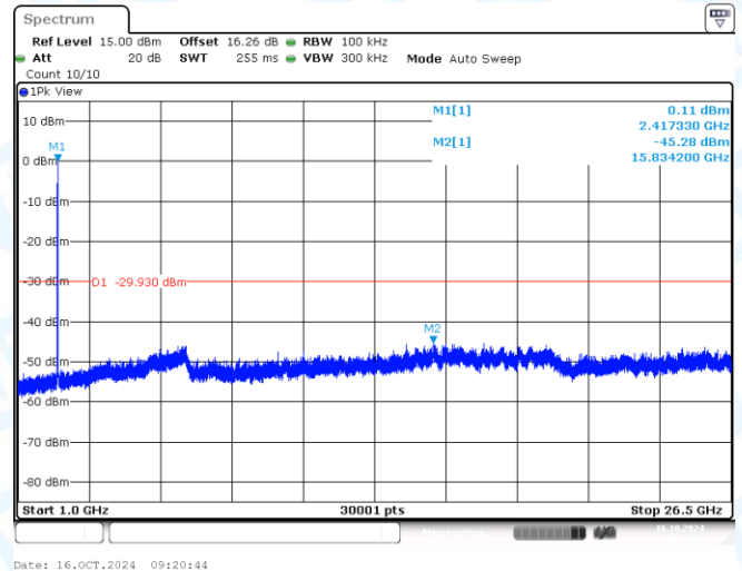
11AX20MIMO-Ant2-2412-1000~26500-PASS
