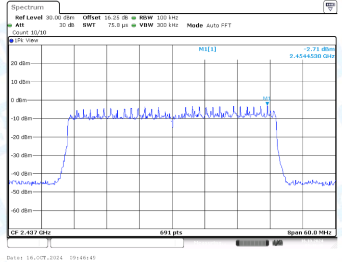
11AX40MIMO-Ant2-2437-0~Reference-PASS
