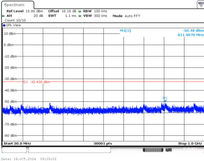
11AX40MIMO-Ant1-2422-30~1000-PASS
