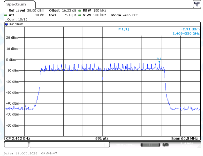
11AX40MIMO-Ant2-2452-0~Reference-PASS
