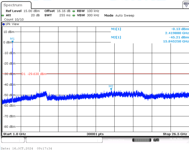
11AX20MIMO-Ant1-2412-1000~26500-PASS
