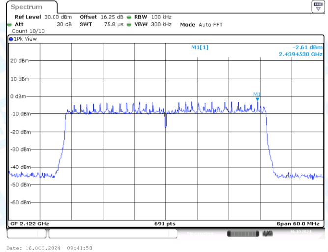
11AX40MIMO-Ant2-2422-0~Reference-PASS
