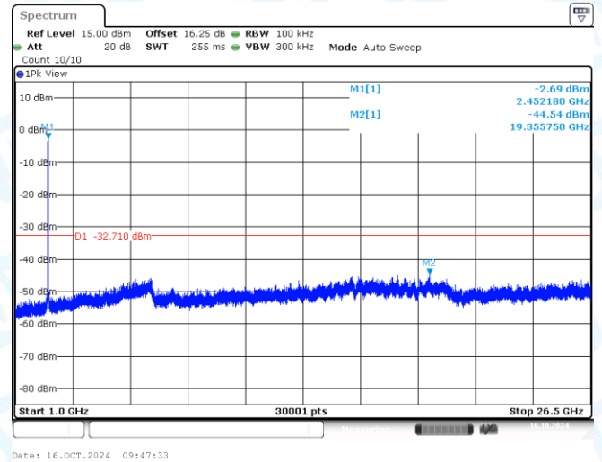
11AX40MIMO-Ant2-2437-1000~26500-PASS
