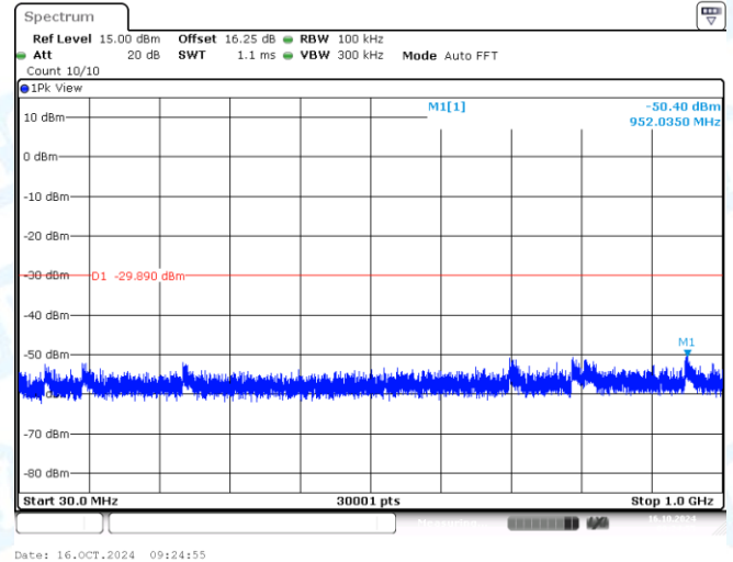
11AX20MIMO-Ant2-2437-30~1000-PASS
