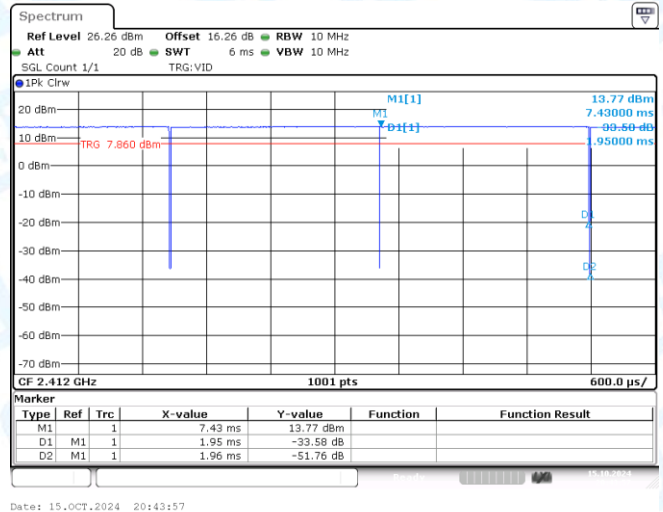
NTNV-11B-CDD-Ant2-2412
