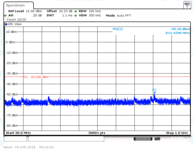
11N40MIMO-Ant2-2452-30~1000-PASS
