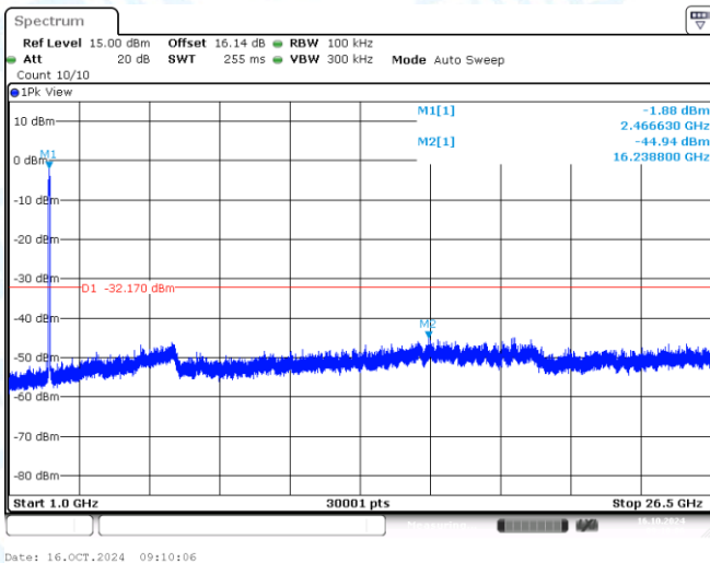
11N40MIMO-Ant1-2452-1000~26500-PASS
