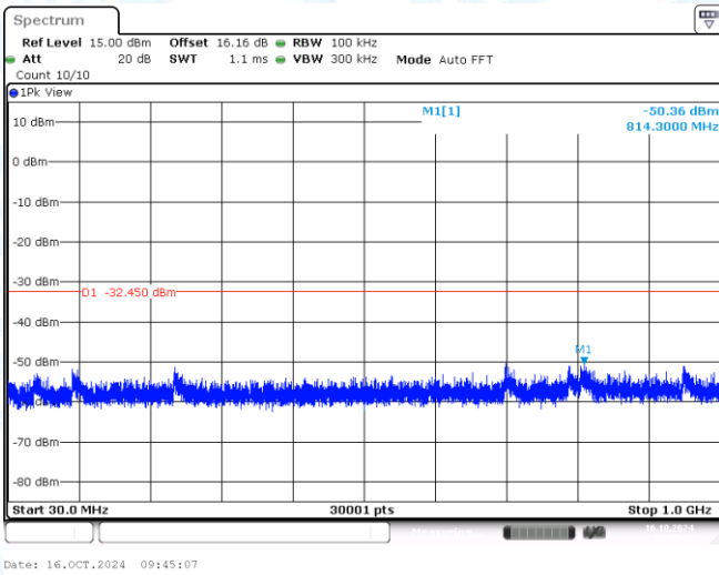
11AX40MIMO-Ant1-2437-30~1000-PASS
