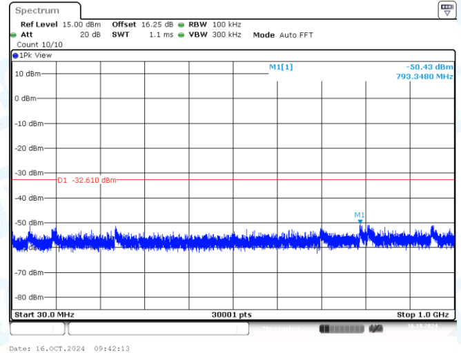
11AX40MIMO-Ant2-2422-30~1000-PASS
