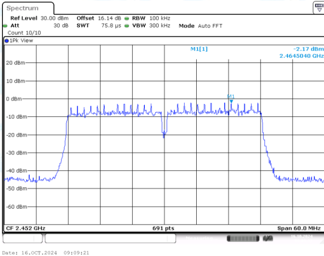
11N40MIMO-Ant1-2452-0~Reference-PASS
