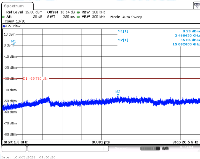
11AX20MIMO-Ant1-2462-1000~26500-PASS
