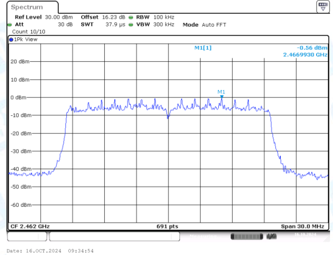
11AX20MIMO-Ant2-2462-0~Reference-PASS
