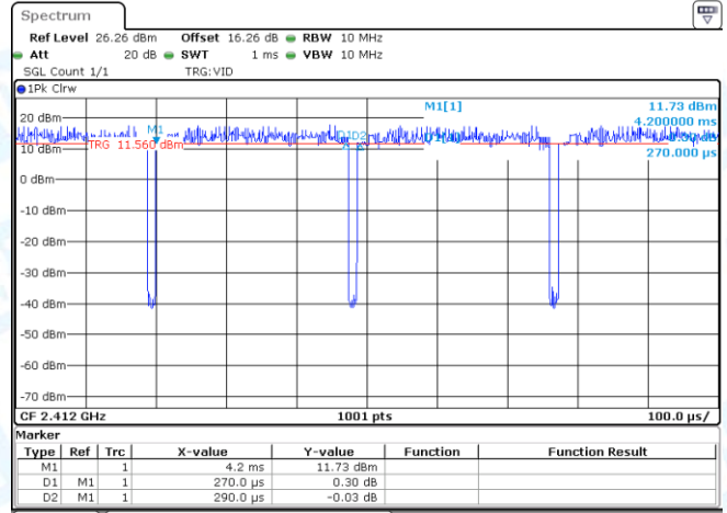
NTNV-11AX20MIMO-Ant2-2412
