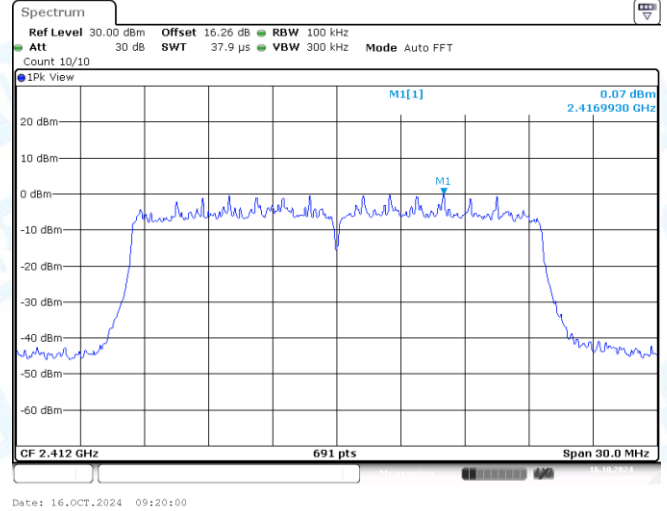
11AX20MIMO-Ant2-2412-0~Reference-PASS
