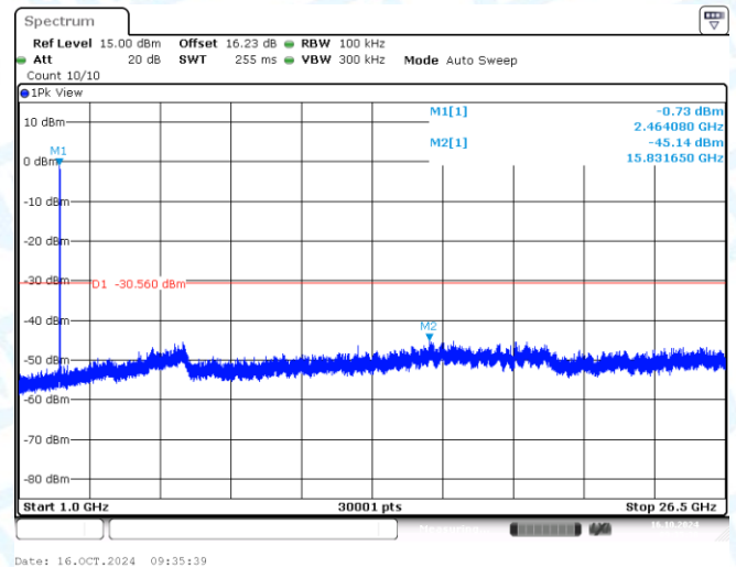
11AX20MIMO-Ant2-2462-1000~26500-PASS
