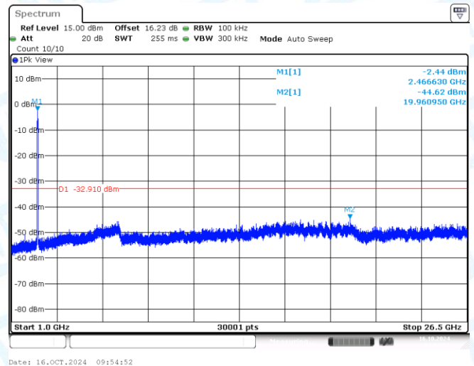
11AX40MIMO-Ant2-2452-1000~26500-PASS
