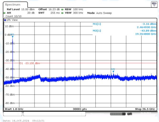
11N40MIMO-Ant2-2452-1000~26500-PASS
