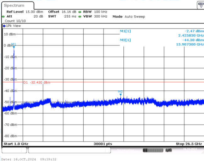
11AX40MIMO-Ant1-2422-1000~26500-PASS
