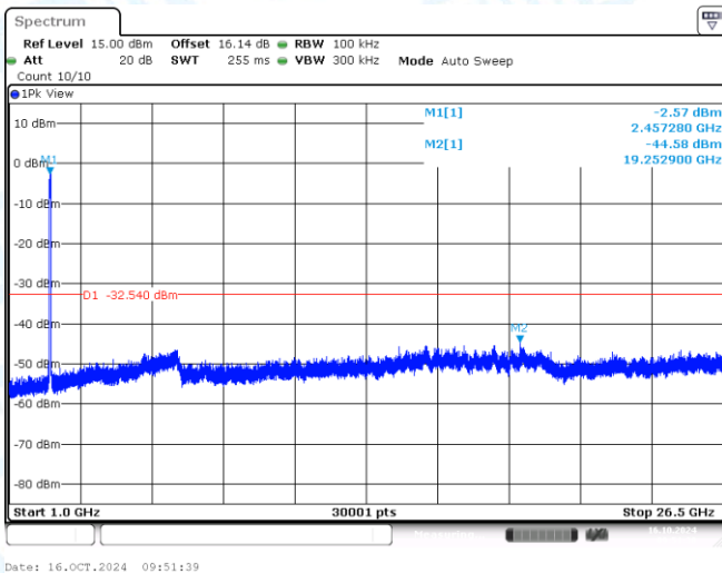
11AX40MIMO-Ant1-2452-1000~26500-PASS
