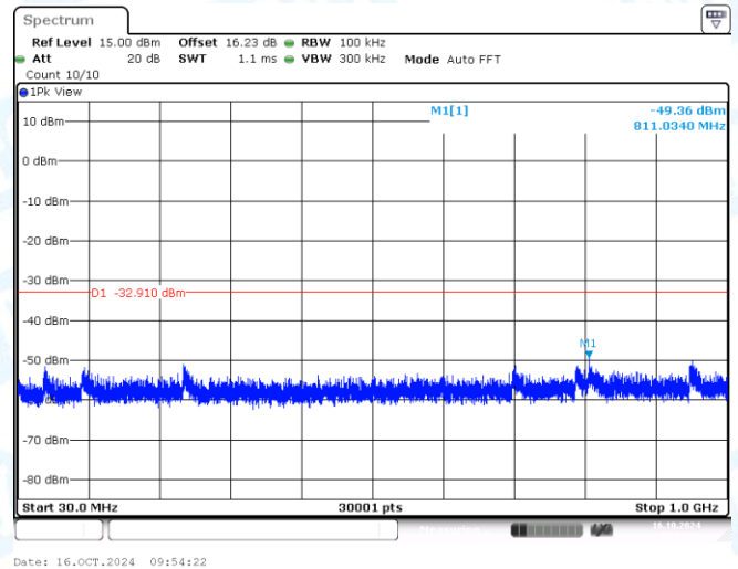
11AX40MIMO-Ant2-2452-30~1000-PASS
