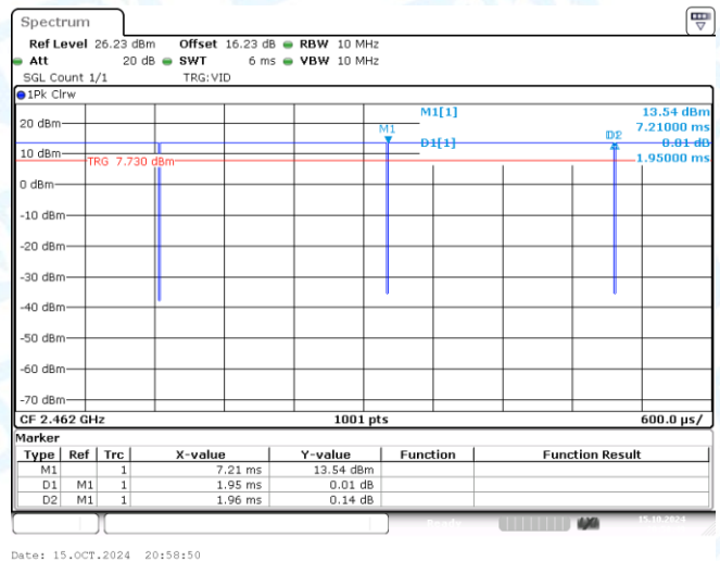
NTNV-11B-CDD-Ant2-2462
