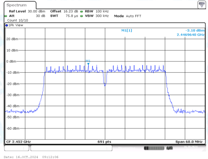
11N40MIMO-Ant2-2452-0~Reference-PASS
