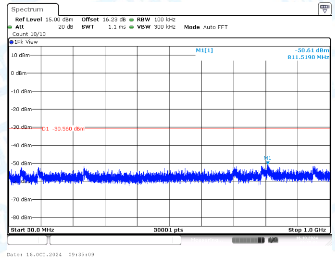
11AX20MIMO-Ant2-2462-30~1000-PASS
