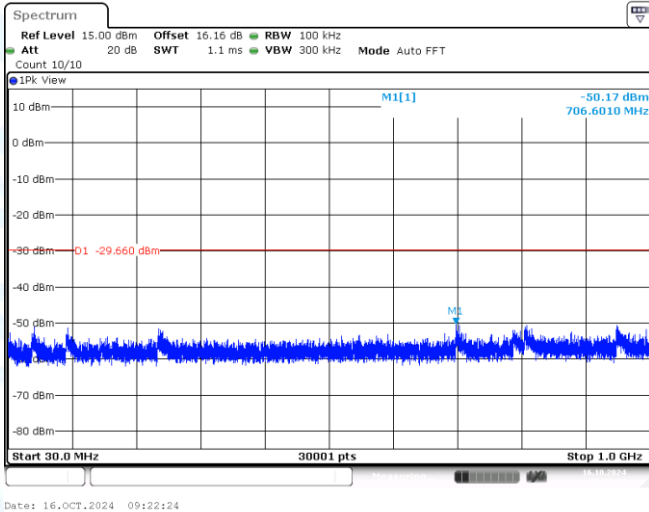
11AX20MIMO-Ant1-2437-30~1000-PASS
