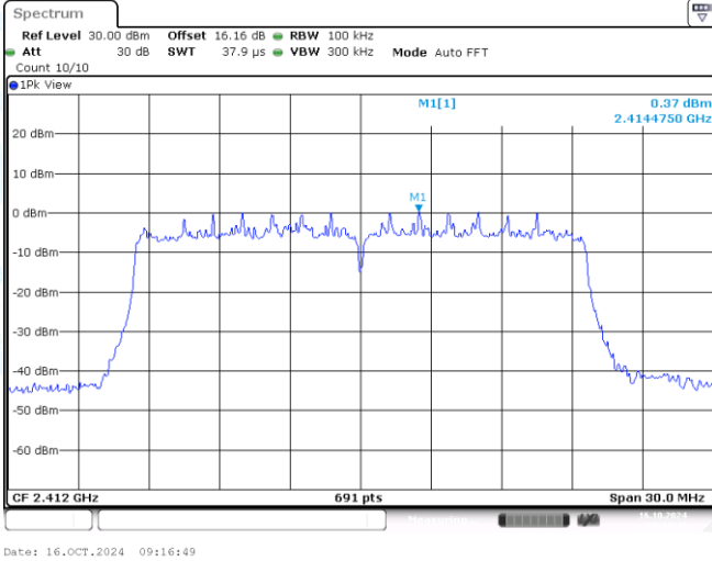
11AX20MIMO-Ant1-2412-0~Reference-PASS
