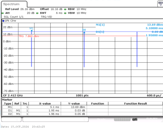
NTNV-11B-CDD-Ant1-2412
