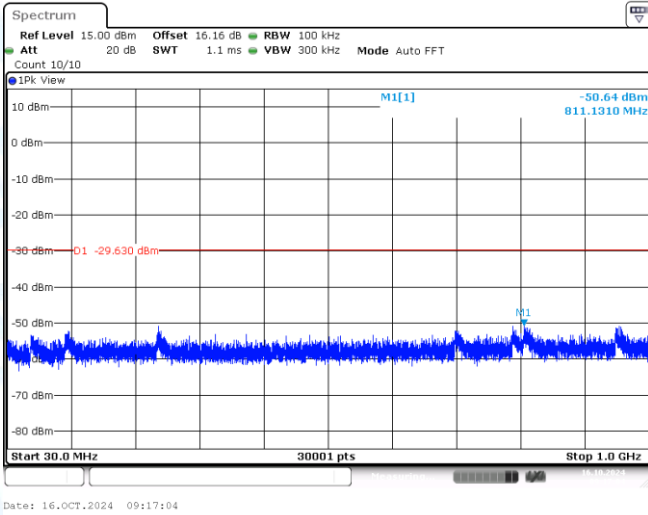
11AX20MIMO-Ant1-2412-30~1000-PASS
