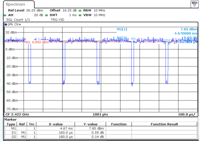
NTNV-11AX40MIMO-Ant2-2422
