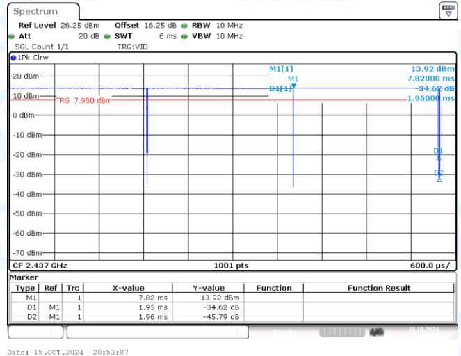
NTNV-11B-CDD-Ant2-2437
