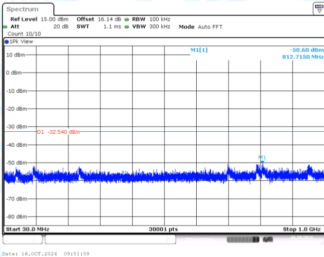
11AX40MIMO-Ant1-2452-30~1000-PASS
