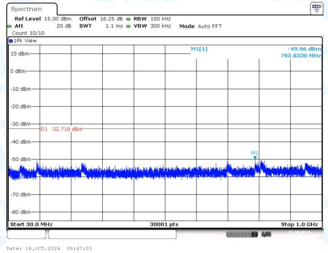
11AX40MIMO-Ant2-2437-30~1000-PASS
