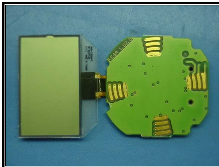
Photograph 31: EUT ICD Display-PCB Bottom View
