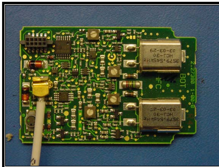
Photograph 45: Module RF PCB without Port Top View
