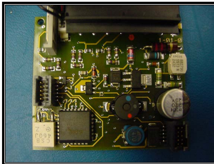
Photograph 41: Module Parts PCB1 Top View
