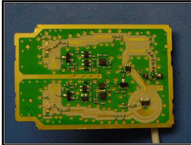
Photograph 46: Module RF PCB without Port Bottom View
