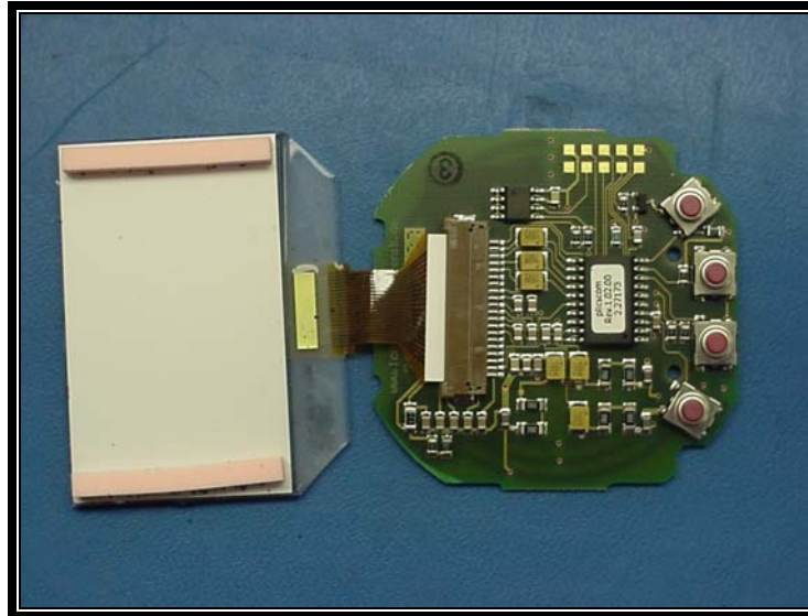
Photograph 32: EUT ICD Display-PCB Top View
