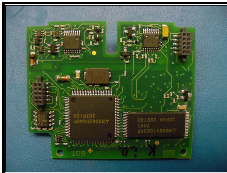
Photograph 43: Module Parts PCB2 Top View
