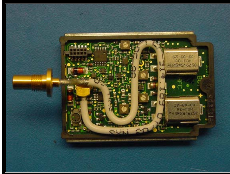
Photograph 44: Module RF PCB with Port Top View
