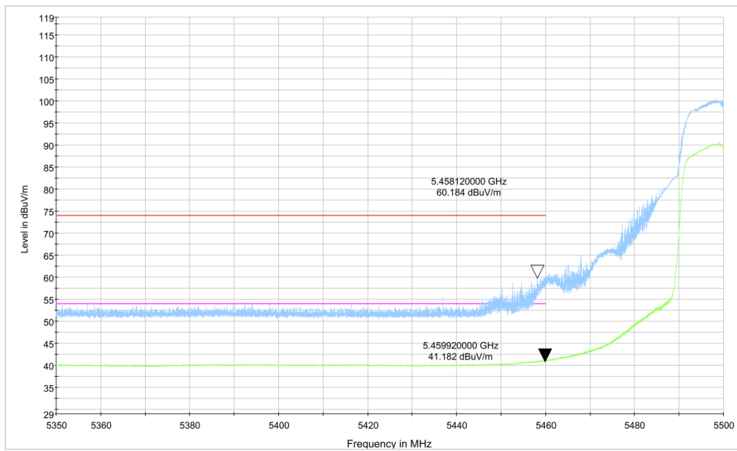
Fig.40 Band Edges (802.11n-HT20 Ch100, 5500MHz)
