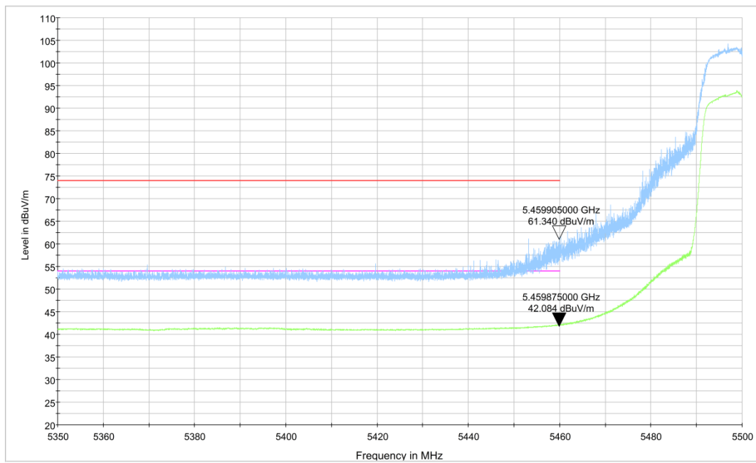
Fig.36 Band Edges (802.11a Ch100, 5500MHz)
