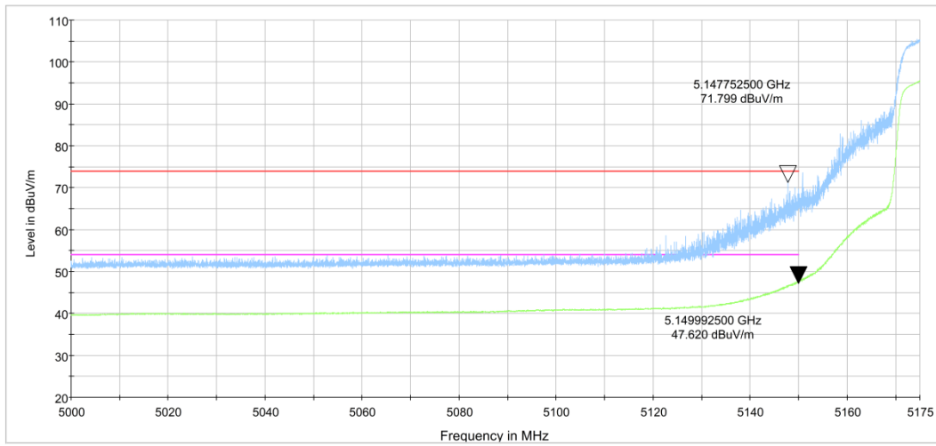
Fig.38 Band Edges (802.11n-HT20 Ch36, 5180MHz)
