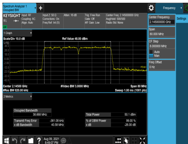
Plot 7-258. Occupied Bandwidth Plot (B66_5M+5M+10M+20M_4C_16QAM – Mid Channel, Port 3)
