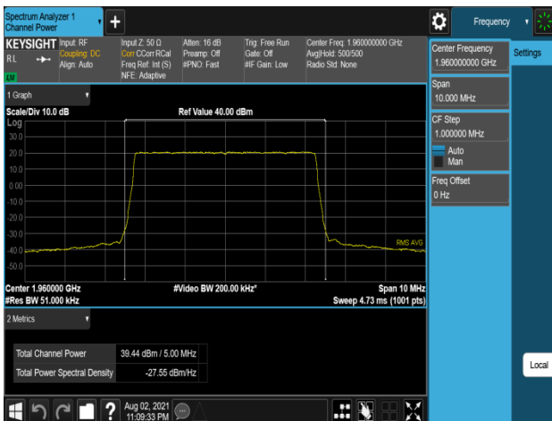
Plot 7-269. Conducted Average Output Power Plot (B2_5M_1C_QPSK - Mid Channel, Port 0)
