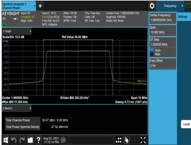
Plot 7-271. Conducted Average Output Power Plot (B2_5M_1C_QPSK - Mid Channel, Port 2)
