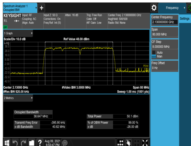
Plot 7-254. Occupied Bandwidth Plot (B66 5M+5M+10M+20M 4C 16QAM - Low Channel, Port 3)
