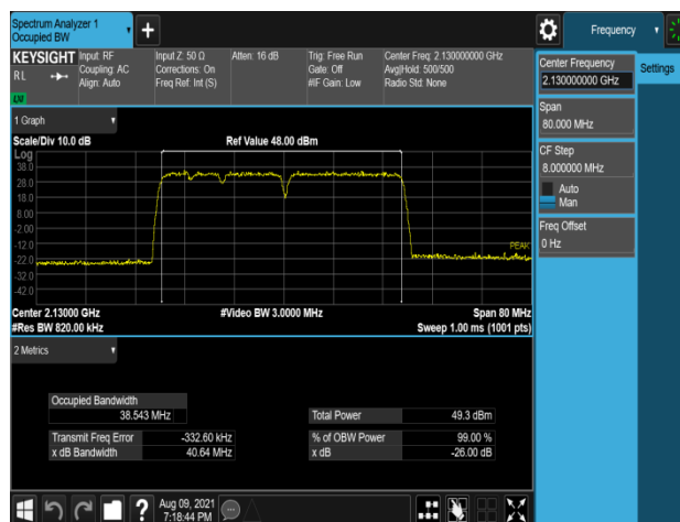
Plot 7-256. Occupied Bandwidth Plot (B66 5M+5M+10M+20M 4C 256QAM - Low Channel, Port 1)
