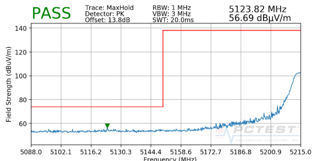
Plot 7-104. Radiated Lower Band Edge Plot (Peak – UNII Band 1 - Interior)
