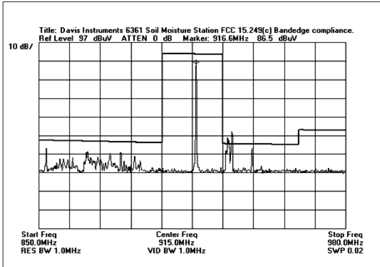
Bandedge Plot
