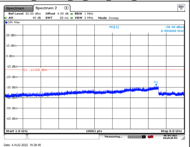
B13_CH23255_5M_1RB0_QPSK_Above 1G
