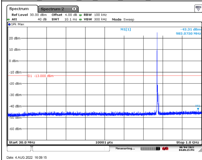
B13_CH23230_5M_1RB0_QPSK_Below 1G
