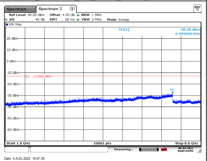
B13_CH23230_5M_1RB0_QPSK_Above 1G
