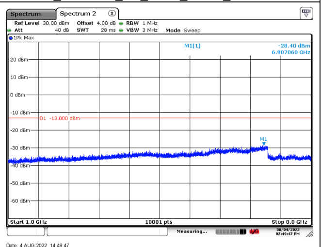
B12_CH23165_3M_1RB0_QPSK_Above 1G
