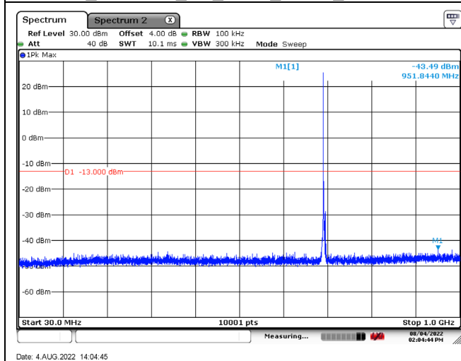
B12_CH23095_3M_1RB0_QPSK_Below 1G
