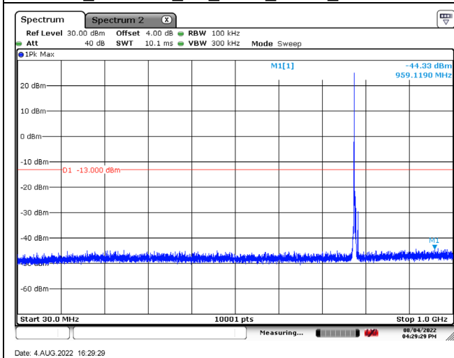
B13_CH23255_5M_1RB0_QPSK_Below 1G
