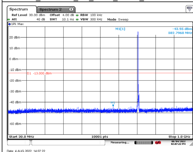
B12_CH23165_3M_1RB0_QPSK_Below 1G
