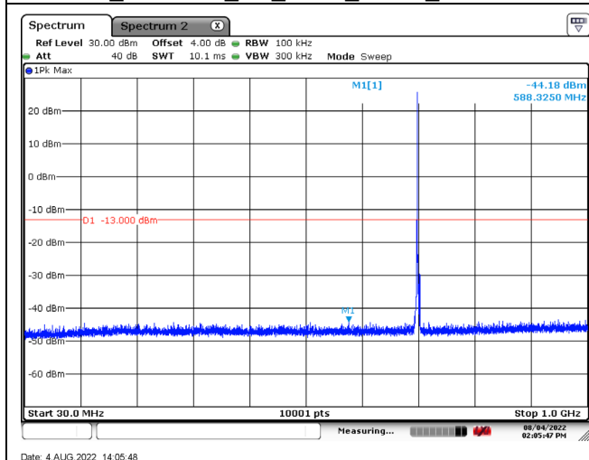
B12_CH23165_3M_1RB0_QPSK_Below 1G
