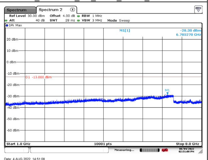
B12_CH23165_3M_1RB0_QPSK_Above 1G
