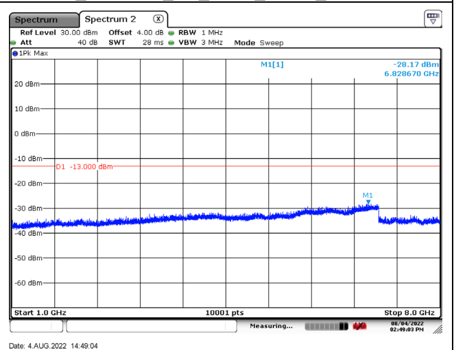
B12_CH23095_3M_1RB0_QPSK_Above 1G
