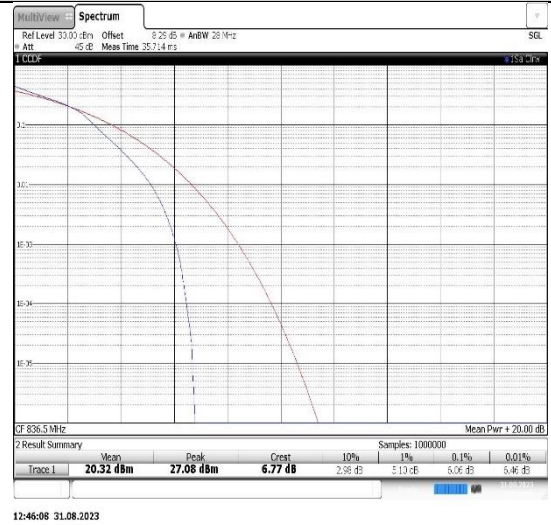
Band26(824-849)-5MHz-16QAM-26915-25RB#0
