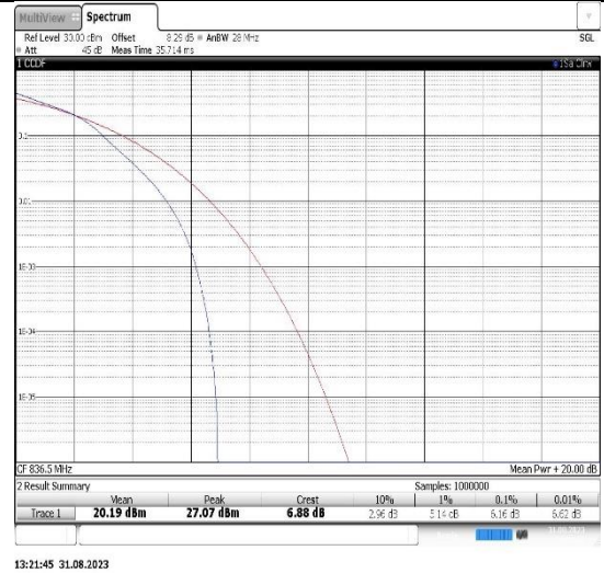
Band26(824-849)-10MHz-16QAM-26915-50RB#0
