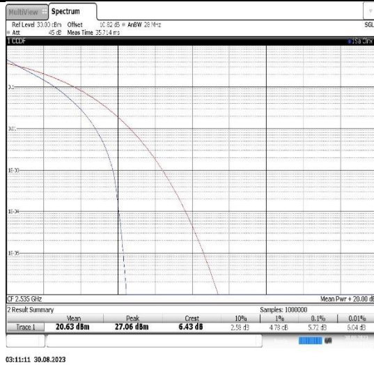
Band7-20MHz-QPSK-21100-100RB#0
