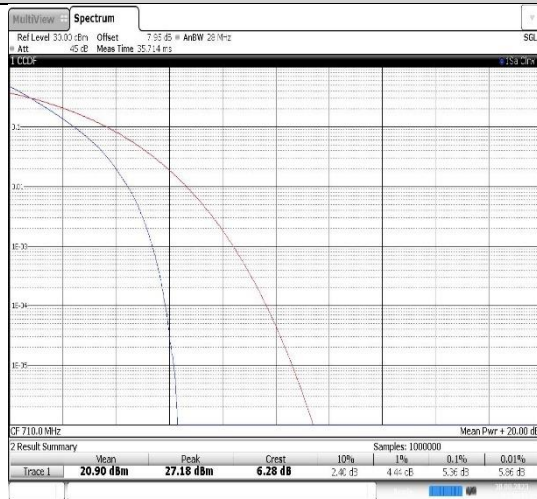
Band17-10MHz-QPSK-23790-50RB#0
