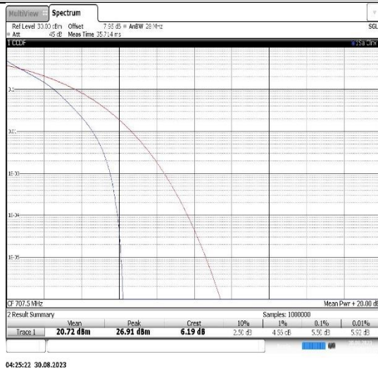
Band12-10MHz-QPSK-23095-50RB#0
