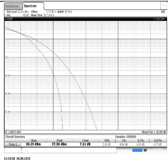
Band25-15MHz-16QAM-26365-75RB#0
