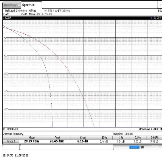
Band26(814-824)-10MHz-QPSK-26740-50RB#0
