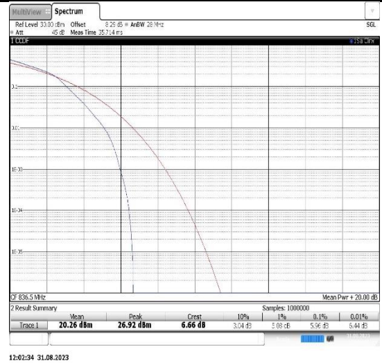
Band26(824-849)-3MHz-16QAM-26915-15RB#0
