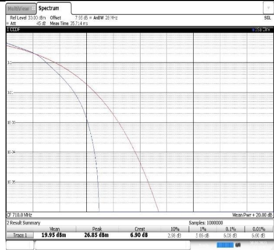
Band17-10MHz-16QAM-23790-50RB#0
