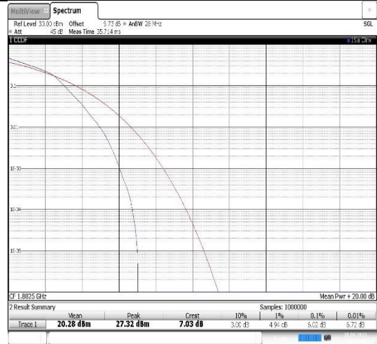
Band25-1.4MHz-16QAM-26365-6RB#0
