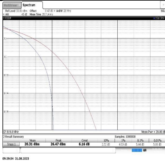
Band26(814-824)-5MHz-QPSK-26740-25RB#0
