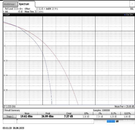
Band7-20MHz-16QAM-21100-100RB#0
