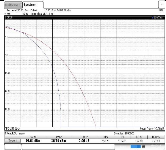
Band7-10MHz-16QAM-21100-50RB#0
