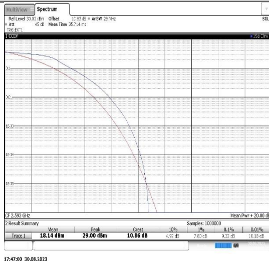
Band41-15MHz-QPSK-40620-75RB#0
