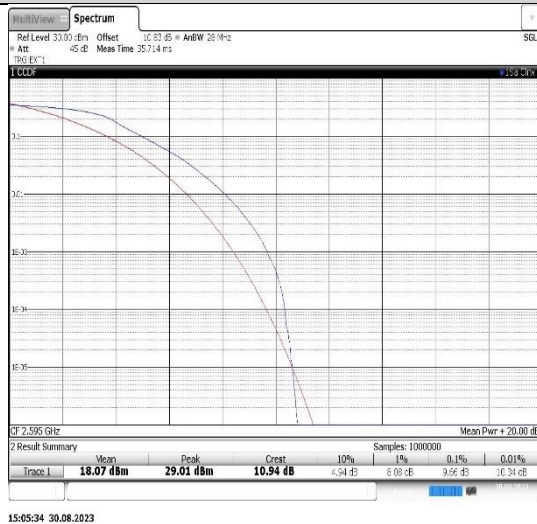
Band38-20MHz-QPSK-38000-100RB#0
