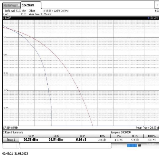
Band26(814-824)-3MHz-QPSK-26740-15RB#0
