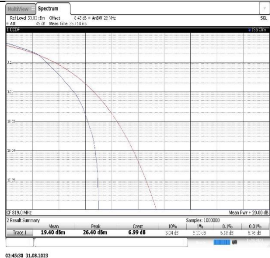
Band26(814-824)-3MHz-16QAM-26740-15RB#0
