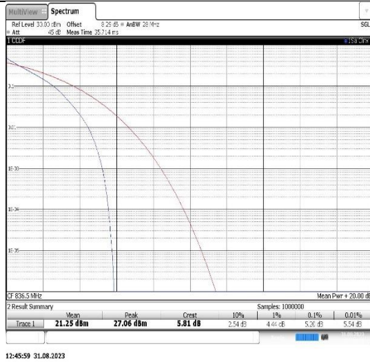
Band26(824-849)-5MHz-QPSK-26915-25RB#0
