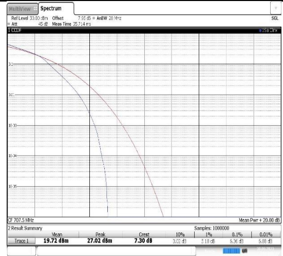
Band12-5MHz-16QAM-23095-25RB#0
