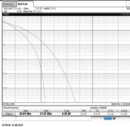
Band26(824-849)-15MHz-QPSK-26915-75RB#0
