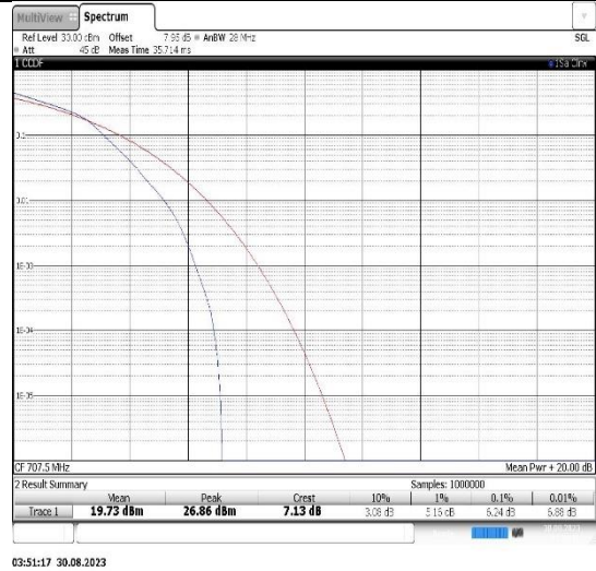
Band12-3MHz-16QAM-23095-15RB#0
