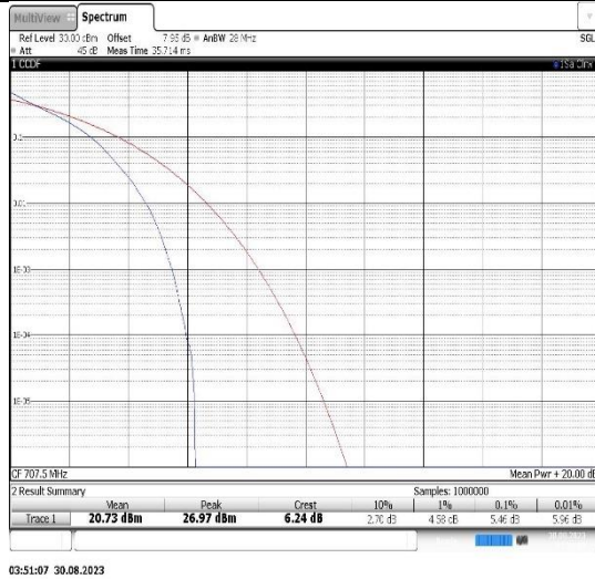
Band12-3MHz-QPSK-23095-15RB#0
