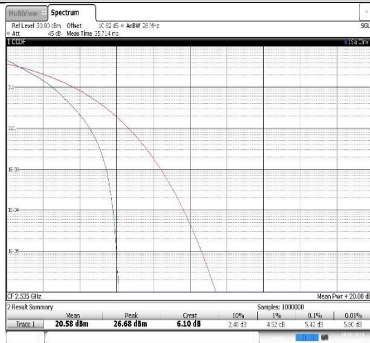
Band7-5MHz-QPSK-21100-25RB#0
