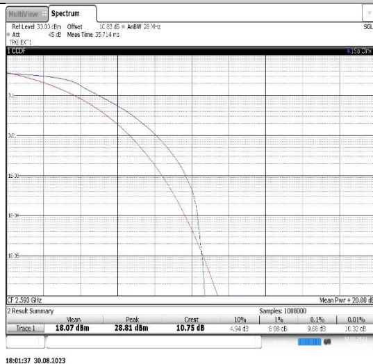
Band41-20MHz-QPSK-40620-100RB#0
