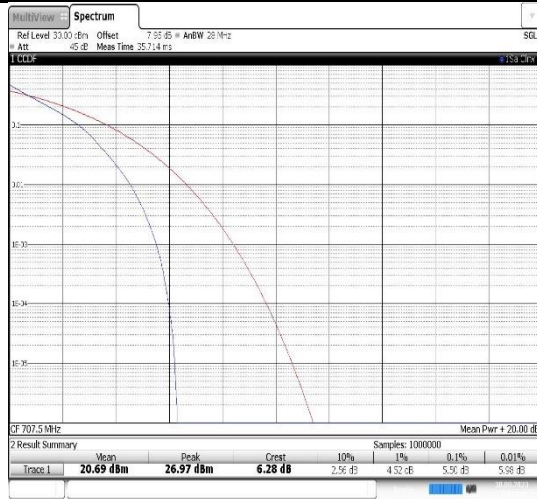
Band12-5MHz-QPSK-23095-25RB#0
