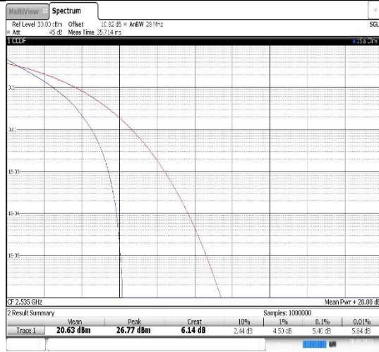
Band7-10MHz-QPSK-21100-50RB#0
