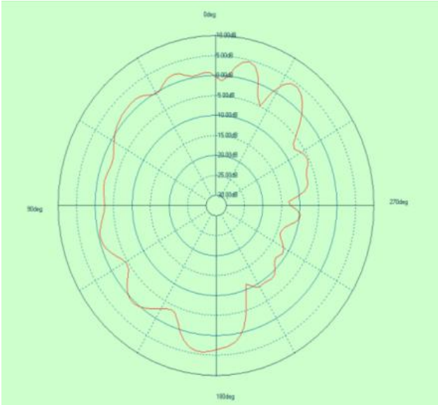
Phi=0.00deg
