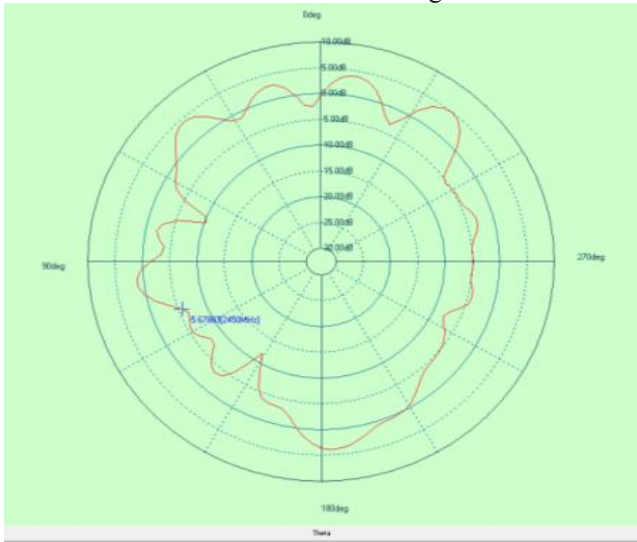
Phi=90.00deg
