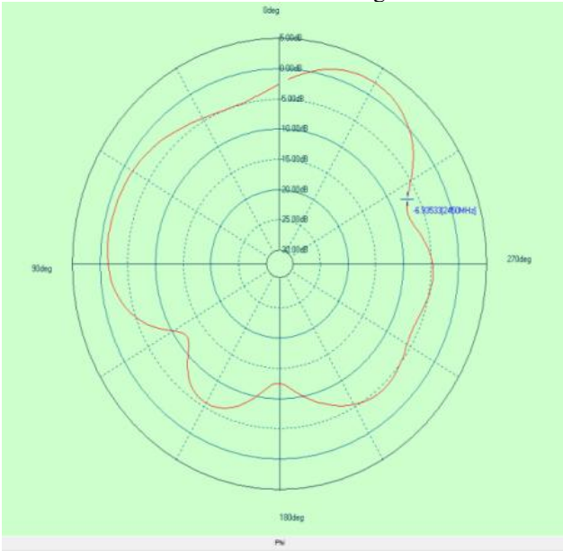
Phi=0.00deg
