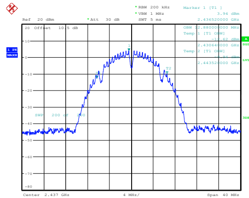
b_2437MHz_Chain 0 12.880MHz
