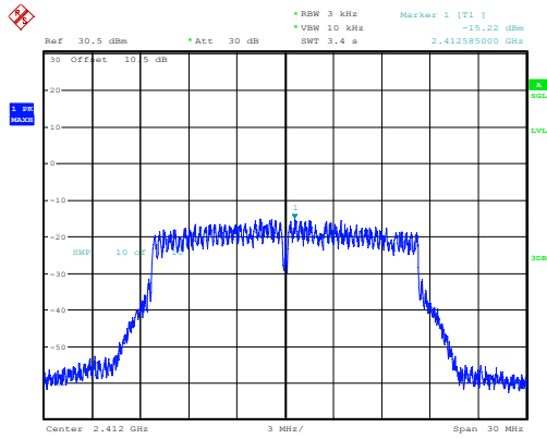
g_2412MHz_Chain 0 -15.22dBm/3kHz
