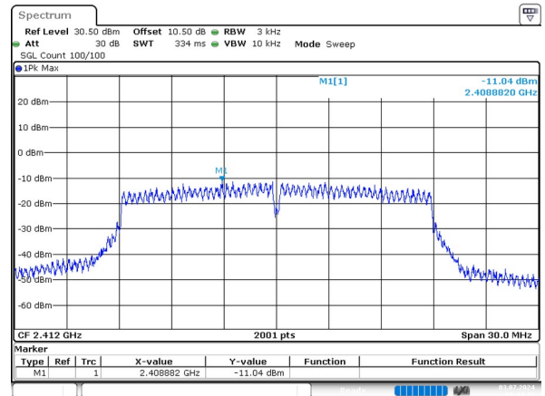
n20_2412MHz_Chain 1 -11.04dBm/3kHz
