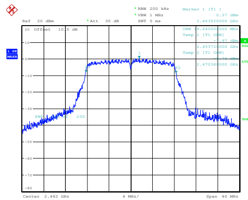
g_2462MHz_Chain 0 16.640MHz
