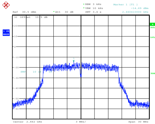
g_2462MHz_Chain 0 -14.69dBm/3kHz
