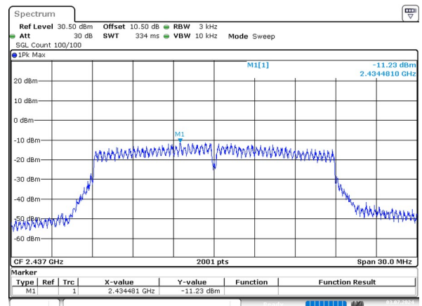
n20_2437MHz_Chain 1 -11.23dBm/3kHz
