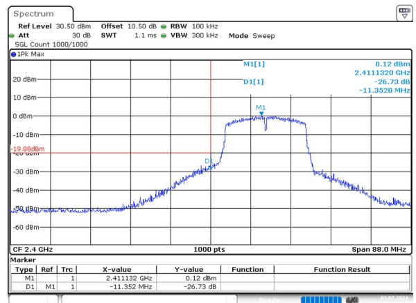
n20_2412MHz_Chain 1 26.73dB
