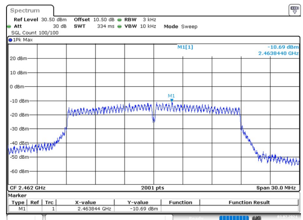
n20_2462MHz_Chain 1 -10.69dBm/3kHz
