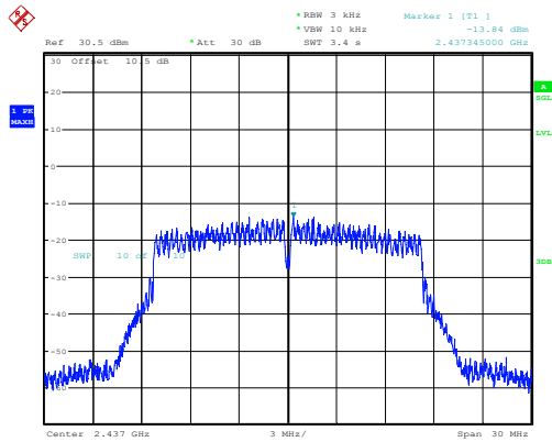
g_2437MHz_Chain 0 -13.84dBm/3kHz
