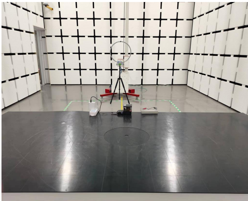
Radiated Disturbance Test (<30M)
