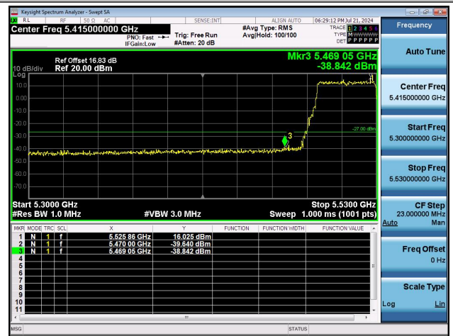
11AX40MIMO-Ant1-5510-PASS
