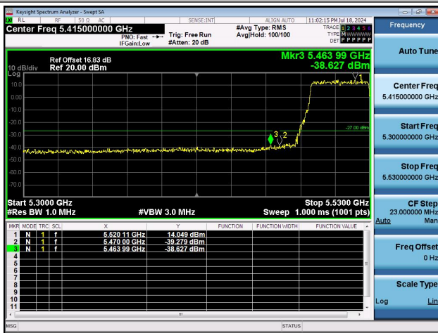
11AX40MIMO-Ant0-5510-PASS
