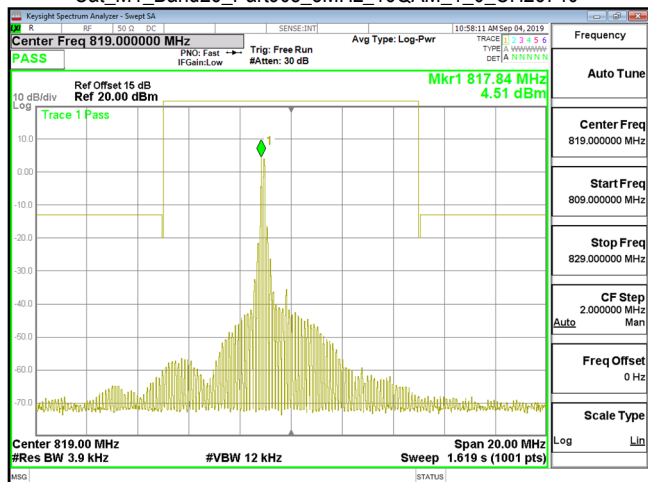
Cat M1_Band26_Part90s_3MHz_16QAM_1_0_CH26740
