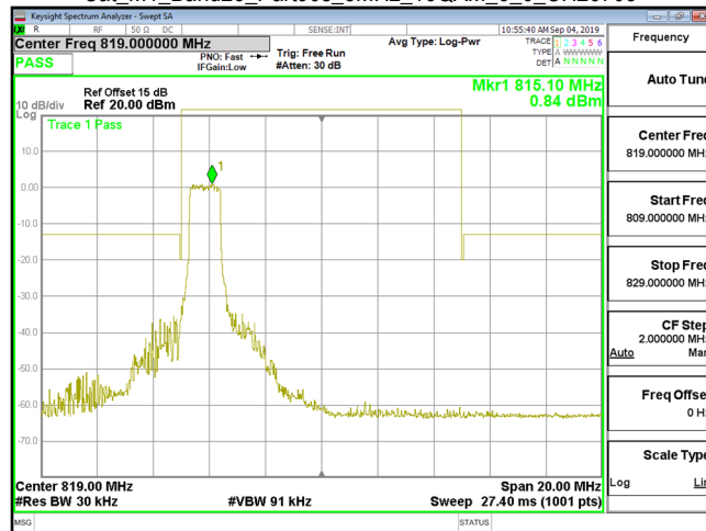
Cat M1_Band26_Part90s_3MHz_16QAM_6_0_CH26705
