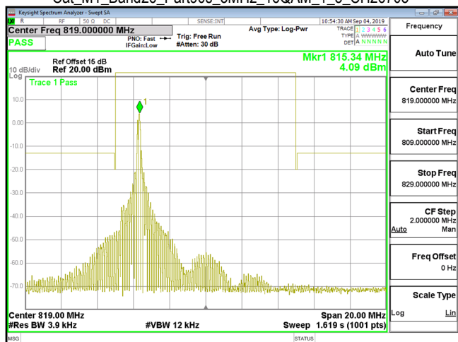
Cat M1_Band26_Part90s_3MHz_16QAM_1_5_CH26705
