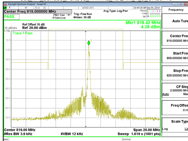
Cat_M1_Band26_Part90s_1.4MHz_16QAM_1_5_CH26740
