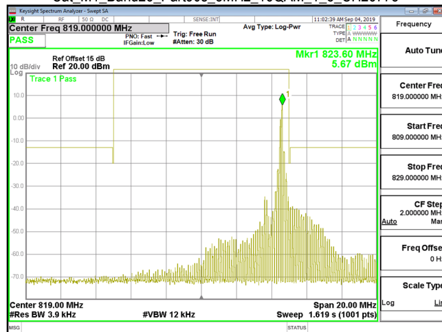
Cat M1_Band26_Part90s_3MHz_16QAM_1_5_CH26775
