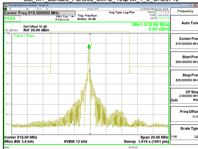
Cat M1_Band26_Part90s_3MHz_16QAM_1_5_CH26740
