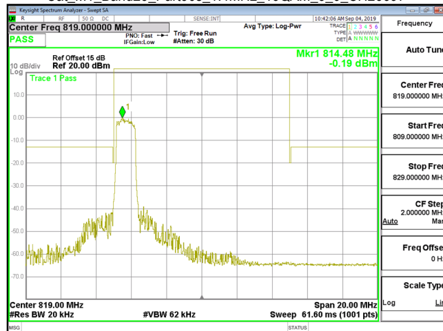
Cat_M1_Band26_Part90s_1.4MHz_16QAM_6_0_CH26697
