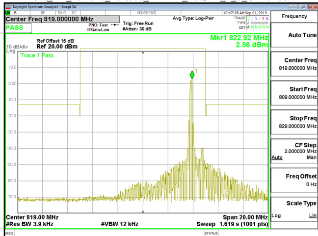
Cat_M1_Band26_Part90s_1.4MHz_16QAM_1_0_CH26783
