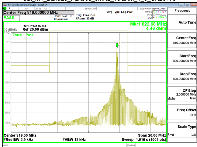
Cat M1_Band26_Part90s_3MHz_16QAM_1_0_CH26775
