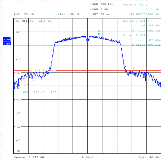
11N40SISO-Ant1-5795
