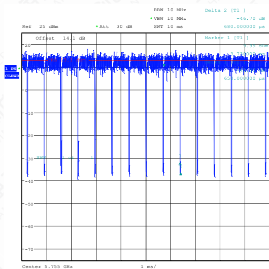
NTNV-11AC40SISO-Ant1-5755
