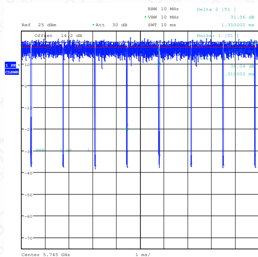
NTNV-11AC20SISO-Ant1-5745
