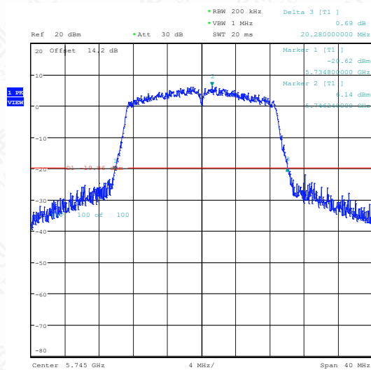
11AC20SISO-Ant1-5745
