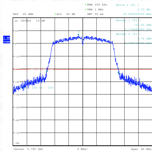
11AC20SISO-Ant1-5785
