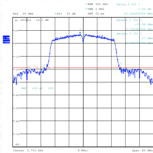
11N40SISO-Ant1-5755
