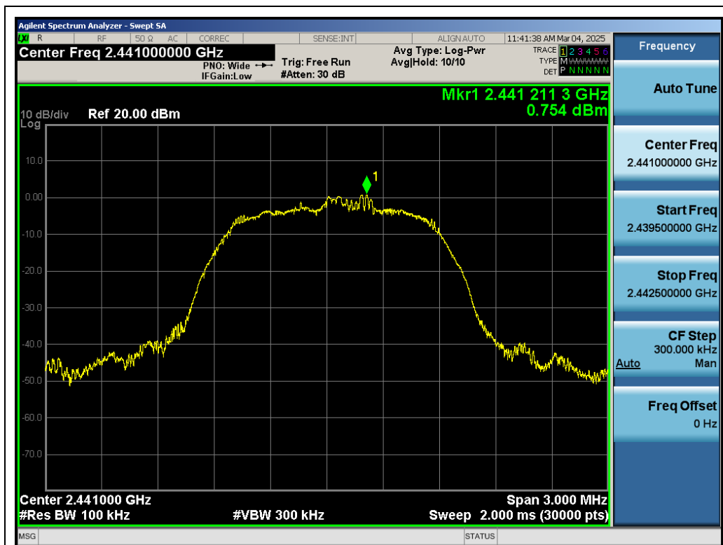
Test_Graph_EDR_ANT1_2441_2Mbps_Reference Level
