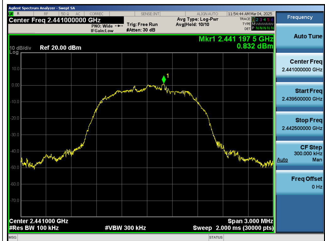
Test_Graph_EDR_ANT1_2441_3Mbps_Reference Level
