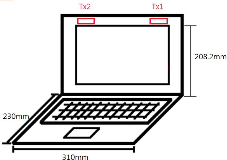
Photograph 11. Antenna position of EUT
