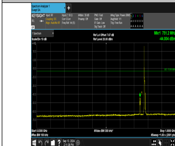
Band13_5MHz_QPSK_23230_1RB#0_30~1000_30~1000
