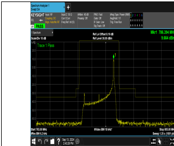
Band13_10MHz_QPSK_23230_1RB#49
