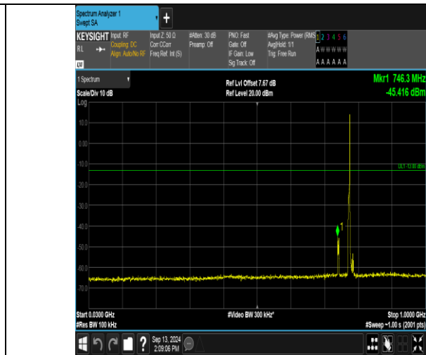
Band13_5MHz_16QAM_23205_1RB#24_30~1000_30~1000
