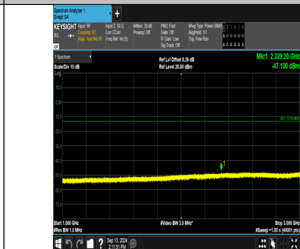
Band13_5MHz_QPSK_23230_1RB#0_1000~3000_1000~3000
