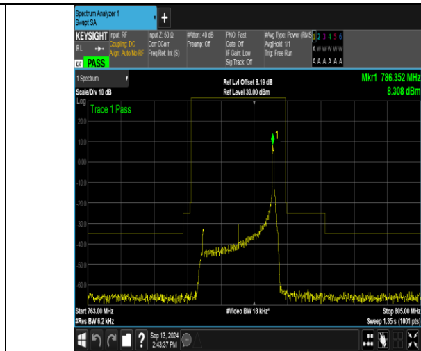
Band13_10MHz_16QAM_23230_1RB#49
