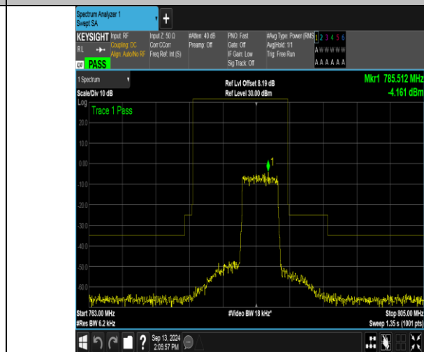
Band13_5MHz_16QAM_23255_25RB#0
