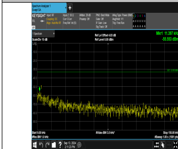
Band13_5MHz_QPSK_23230_1RB#0_0.009~0.15_0.009~0.15
