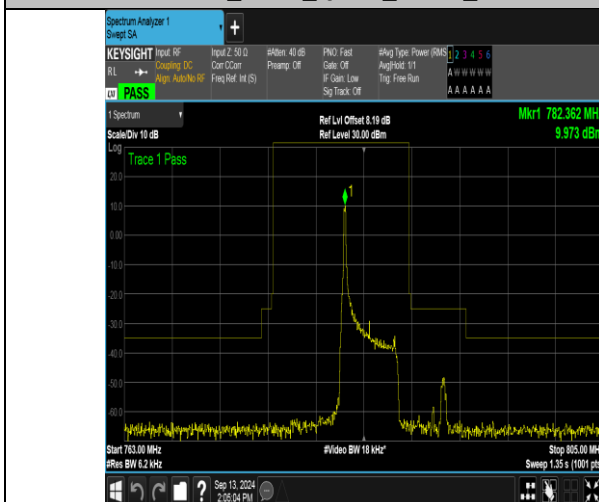
Band13_5MHz_QPSK_23255_1RB#0
