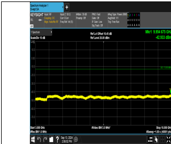
Band13_5MHz_QPSK_23205_1RB#0_3000~10000_3000~10000
