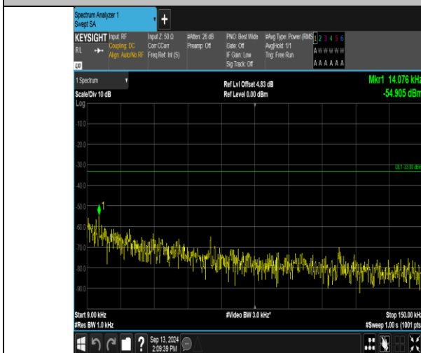
Band13_5MHz_QPSK_23205_25RB#0_0.009~0.15_0.009~0.15
