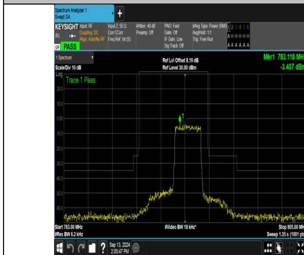
Band13_5MHz_QPSK_23255_25RB#0
