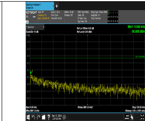
Band13_5MHz_16QAM_23205_1RB#0_0.009~0.15_0.009~0.15
