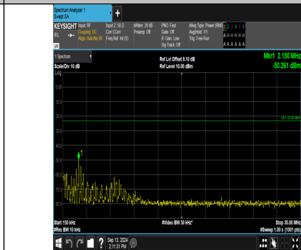
Band13_5MHz_QPSK_23230_1RB#0_0.15~30_0.15~30
