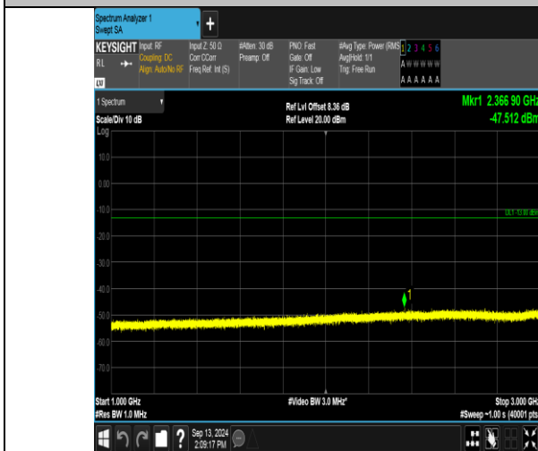
Band13_5MHz_16QAM_23205_1RB#24_1000~3000_1000~3000
