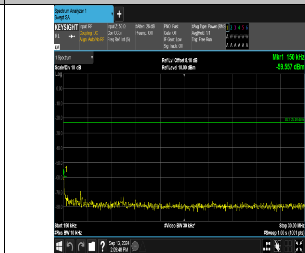
Band13_5MHz_QPSK_23205_25RB#0_0.15~30_0.15~30
