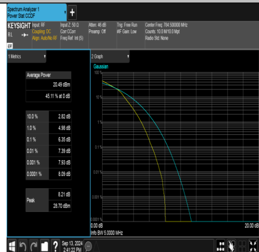
Band13-5MHz-16QAM-23255-25RB#0-PASS
