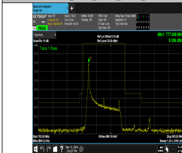
Band13_10MHz_QPSK_23230_1RB#0
