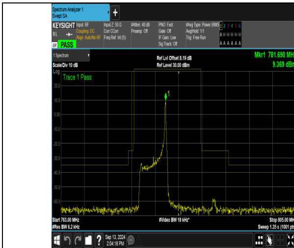
Band13_5MHz_QPSK_23205_1RB#24
