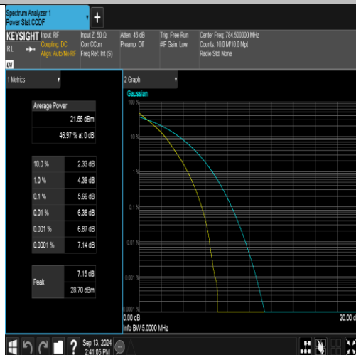
Band13-5MHz-QPSK-23255-25RB#0-PASS
