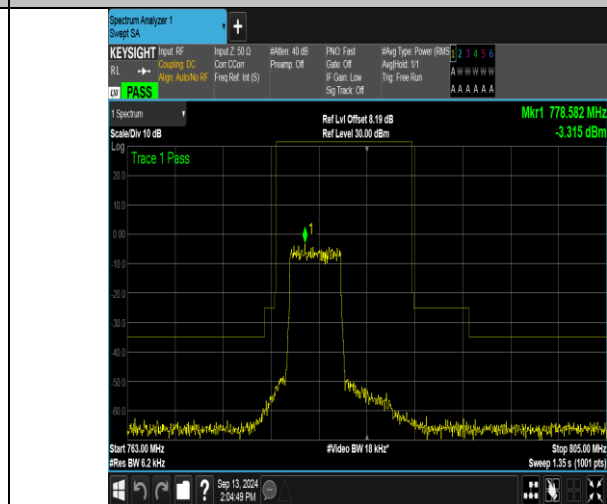
Band13_5MHz_16QAM_23205_25RB#0
