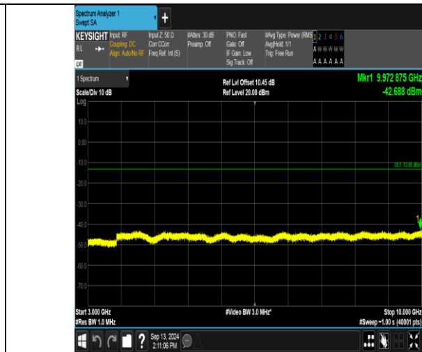
Band13_5MHz_16QAM_23205_25RB#0_3000~10000_3000~10000
