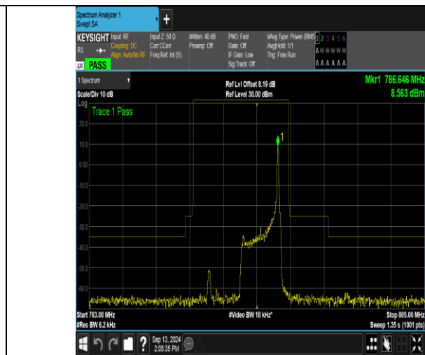
Band13_5MHz_16QAM_23255_1RB#24
