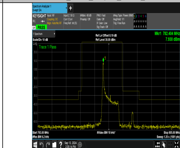
Band13_5MHz_16QAM_23255_1RB#0
