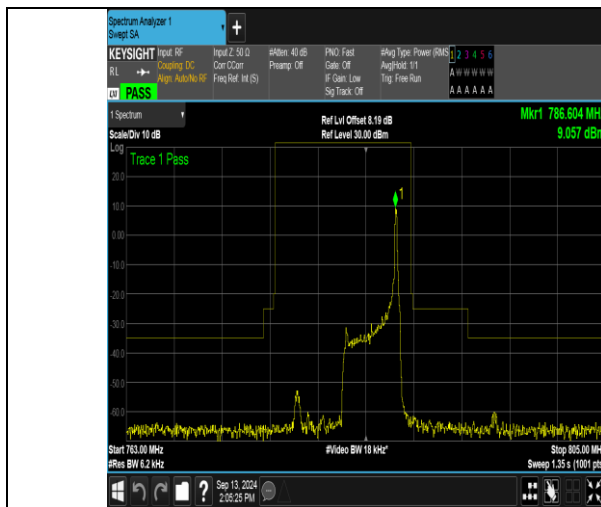
Band13_5MHz_QPSK_23255_1RB#24
