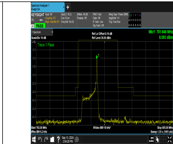
Band13_5MHz_16QAM_23205_1RB#24
