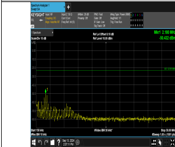
Band13_5MHz_16QAM_23205_1RB#0_0.15~30_0.15~30
