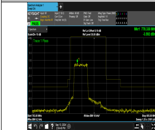
Band13_5MHz_QPSK_23205_25RB#0
