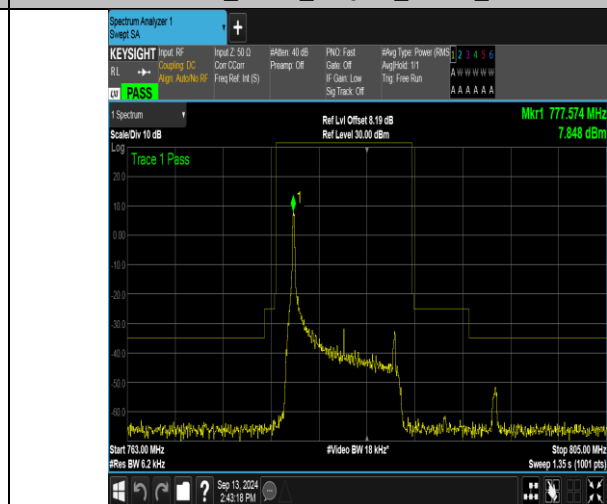
Band13_10MHz_16QAM_23230_1RB#0
