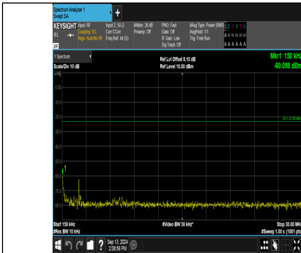
Band13_5MHz_16QAM_23205_1RB#24_0.15~30_0.15~30
