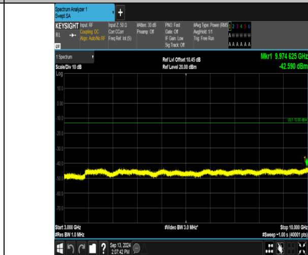
Band13_5MHz_16QAM_23205_1RB#0_3000~10000_3000~10000
