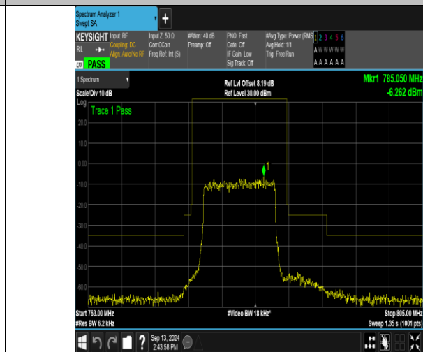
Band13_10MHz_16QAM_23230_50RB#0
