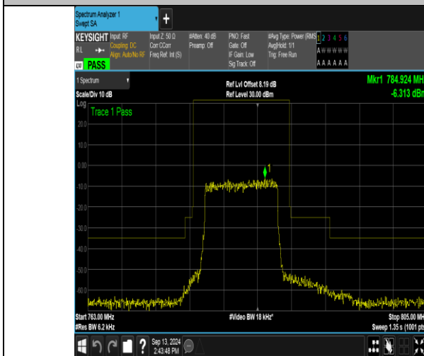
Band13_10MHz_QPSK_23230_50RB#0
