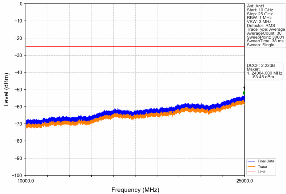
Band41_5MHz_16QAM_MCH_2605MHz_RB_1_0_NTNV
