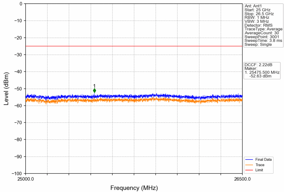
Band41_5MHz_16QAM_HCH_2652.5MHz_RB_1_0_NTNV
