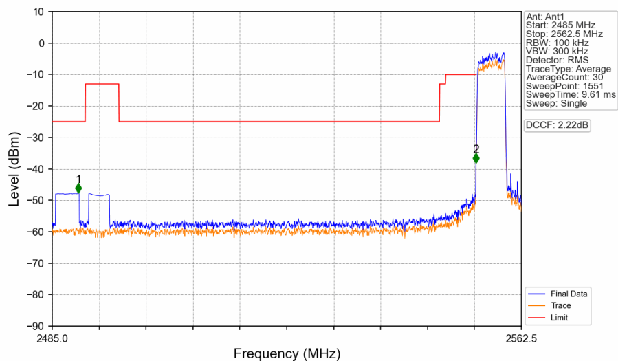
Band41_5MHz_16QAM_LCH_2557.5MHz_RB_25_0_NTNV
