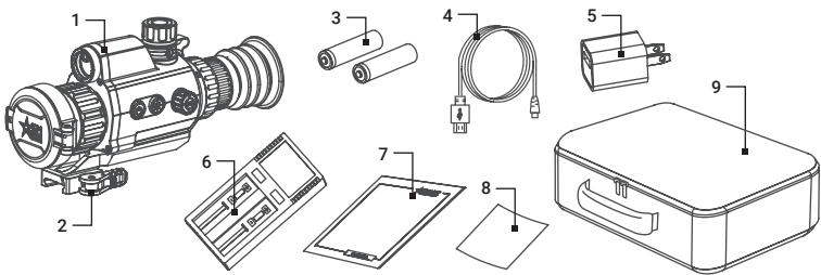
FIGURE 1-2. STANDARD COMPONENTS
