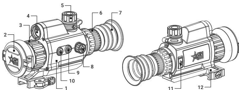
FIGURE 1-1. MAIN PARTS
