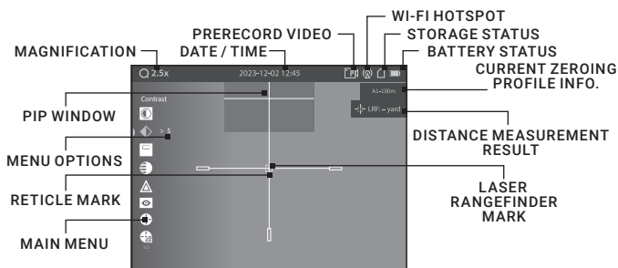
FIGURE 2-3. ON-SCREEN DISPLAY
