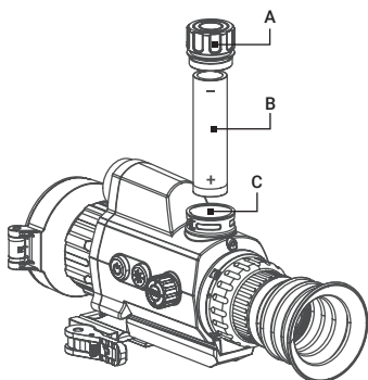
FIGURE 2-1. BATTERY INSTALLATION
