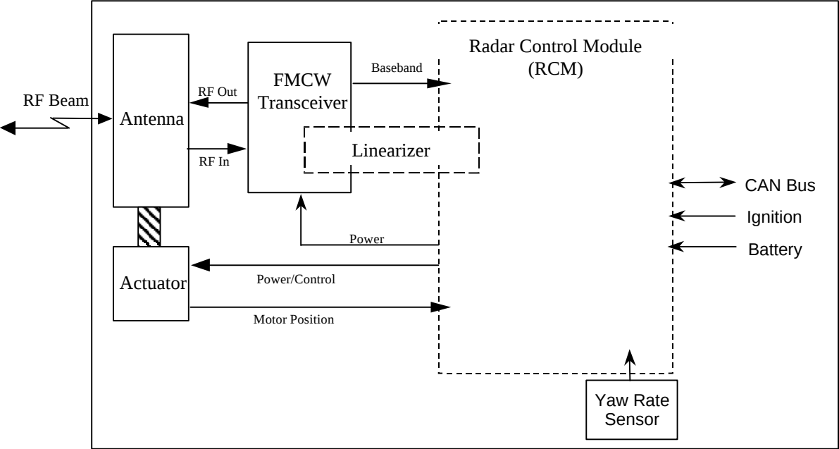
ACC2 System Block Diagram
