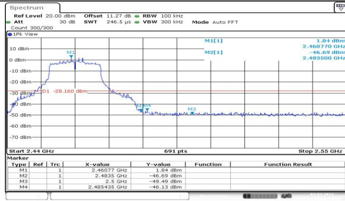
11G_Ant1_High_2462
