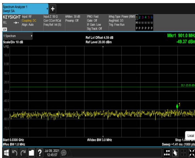
Band7-5MHz-QPSK-21100:30~1000MHz
