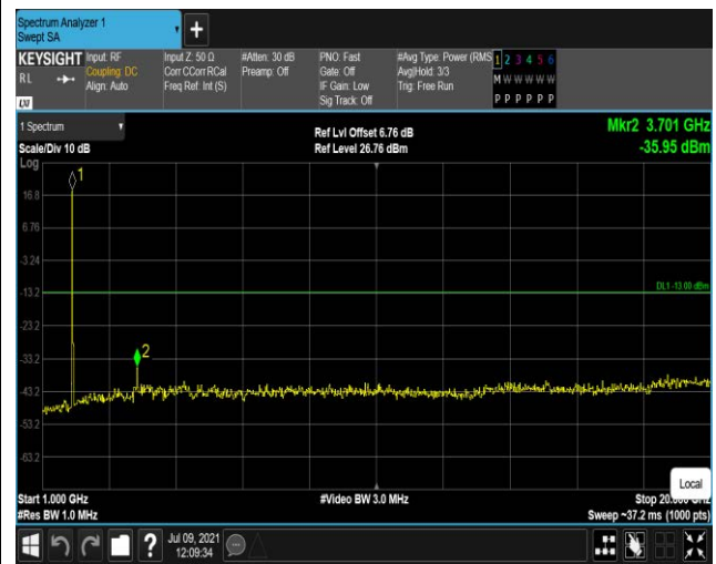
Band2-20MHz-16QAM-18900:1000~20000MHz
