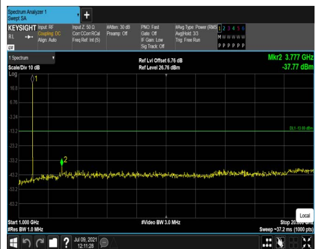
Band2-20MHz-16QAM-19100:1000~20000MHz
