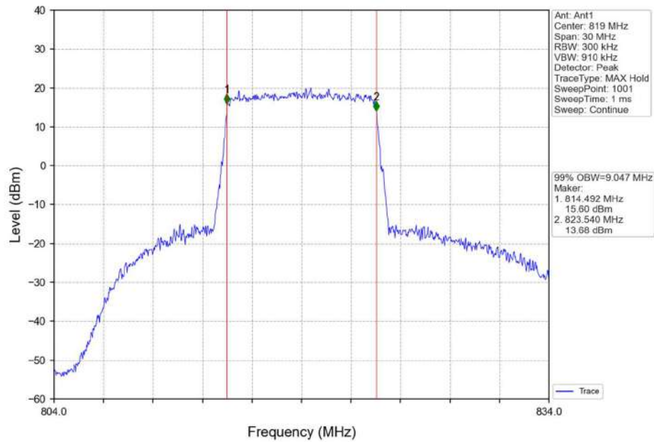
Band26a 10MHz 16QAM MCH 819MHz RB 50 0 NTNV
