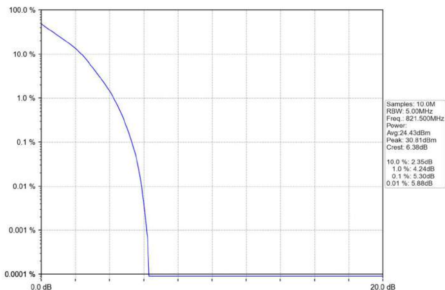
Band26a_5MHz_QPSK_HCH_821.5MHz_RB_25_0_NTNV
