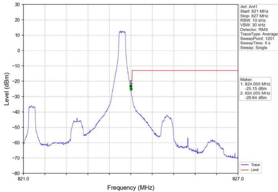
Band26a 3MHz 16QAM HCH 822.5MHz RB 1 14 NTNv
