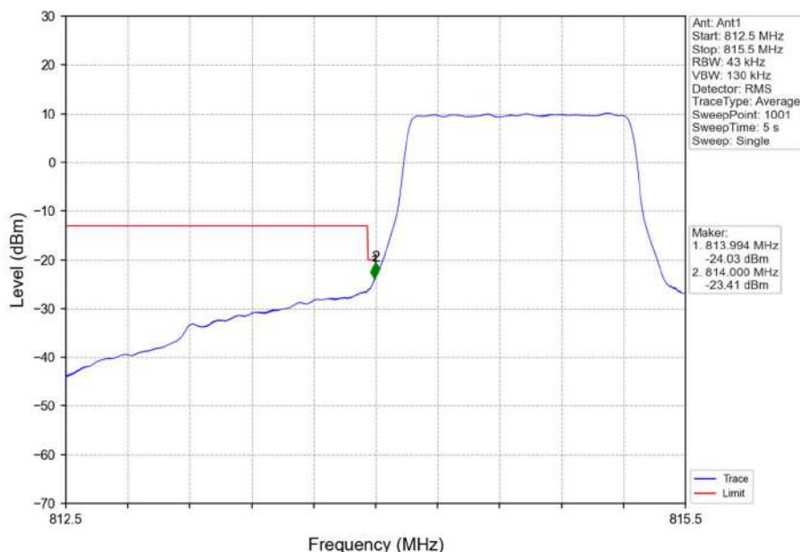
Band26a_1.4MHz_16QAM_LCH_814.7MHz_RB_6_0_NTNV
