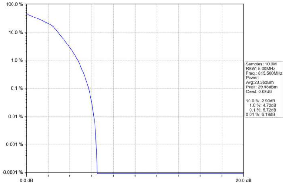
Band26a_3MHz_16QAM_LCH_815.5MHz_RB_15_0_NTNV
