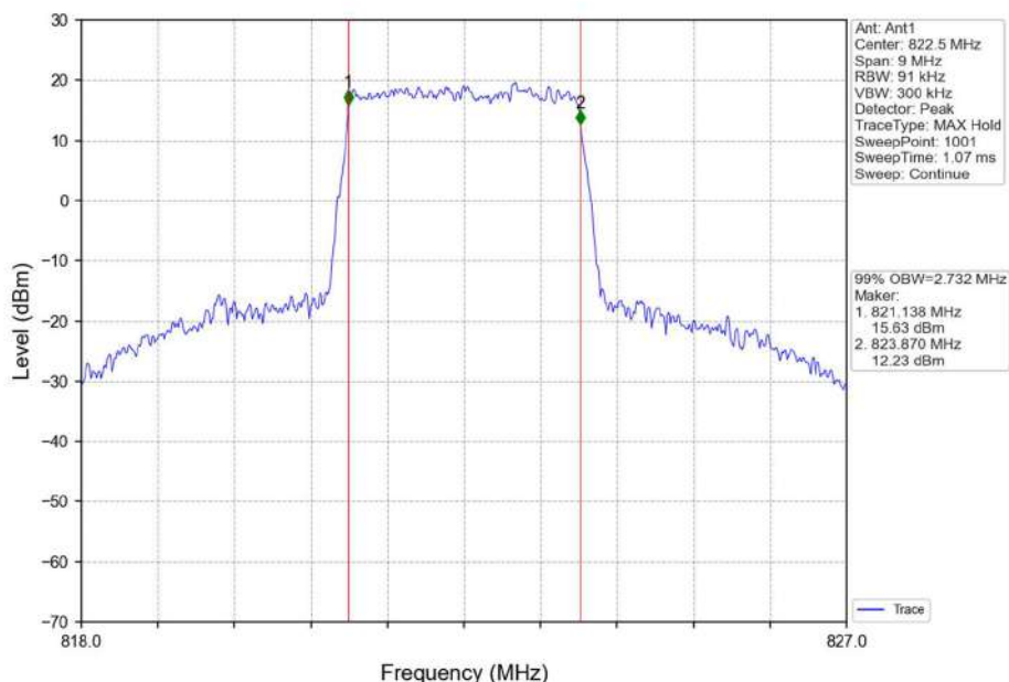
Band26a_3MHz_16QAM_HCH_822.5MHz_RB_15_0_NTNV
