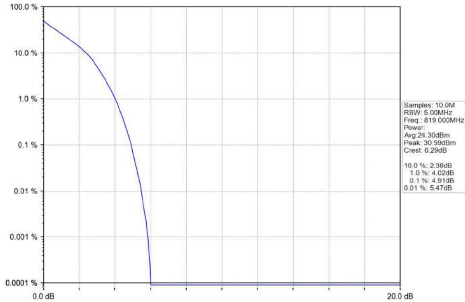
Band26a_3MHz_QPSK_MCH_819MHz_RB_15_0_NTNV
