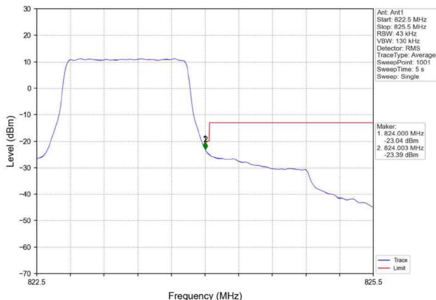
Band26a_1.4MHz_QPSK_HCH_823.3MHz_RB_6_0_NTNV
