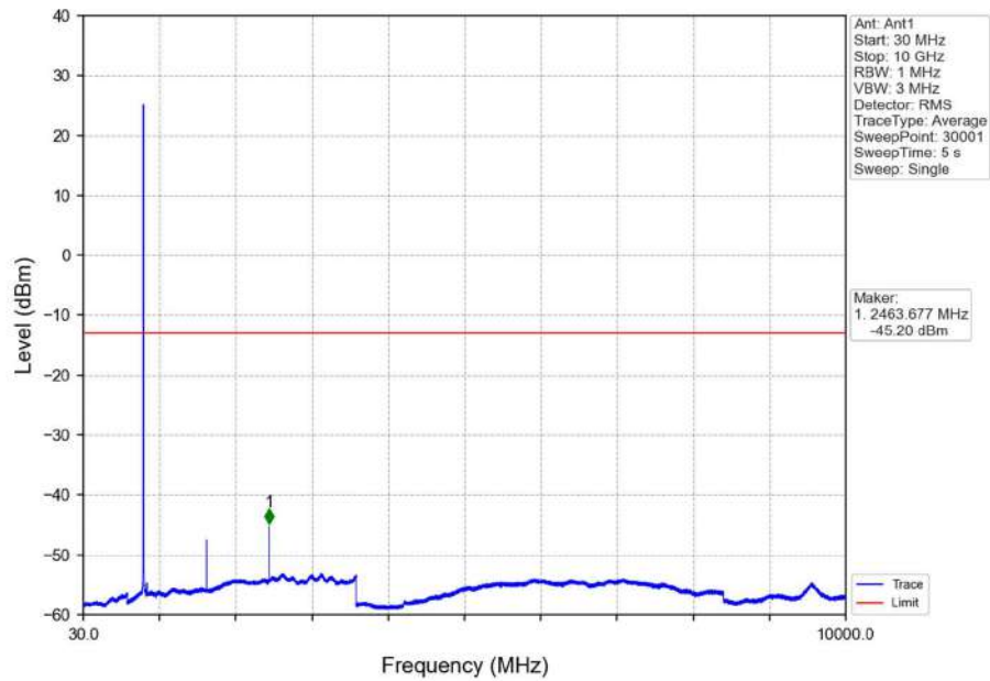
Band26a 3MHz QPSK HCH 822.5MHz RB 1 0 NTNV
