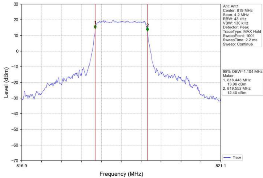
Band26a 1.4MHz 16QAM MCH 819MHz RB 6 0 NTN
