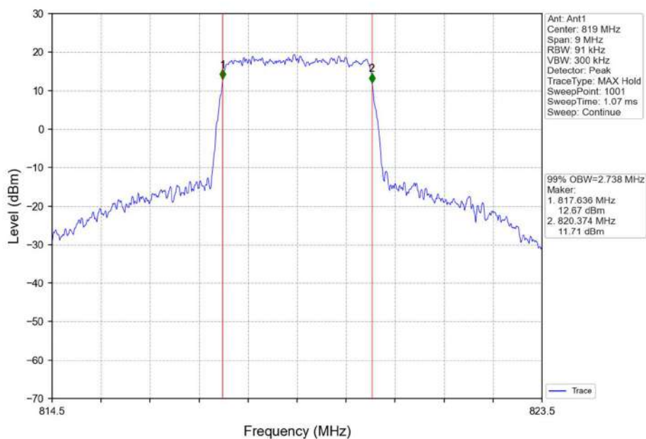
Band26a 3MHz 16QAM MCH 819MHz RB 15 0 NTNV
