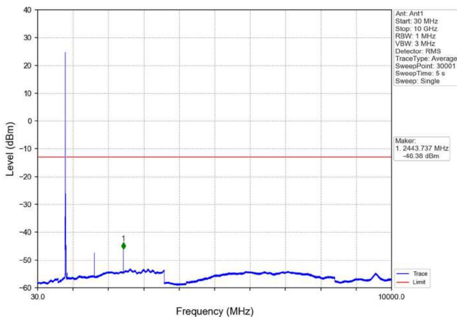
Band26a 10MHz 16QAM LCH 819MHz RB 1 0 NTN
