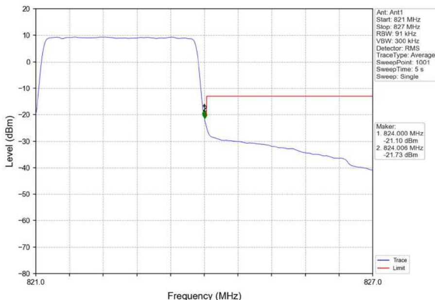
Band26a_3MHz_16QAM_HCH_822.5MHz_RB_15_0_NTNV
