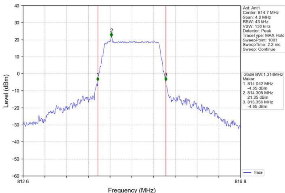
Band26a_1.4MHz_16QAM_LCH_814.7MHz_RB_6_0_NTNV
