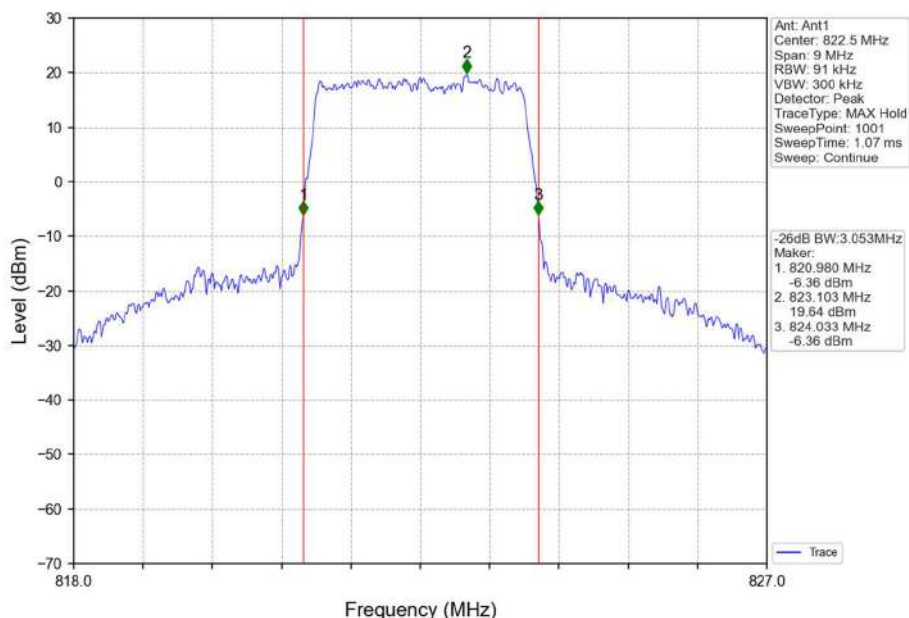
Band26a_3MHz_16QAM_HCH_822.5MHz_RB_15_0_NTNV
