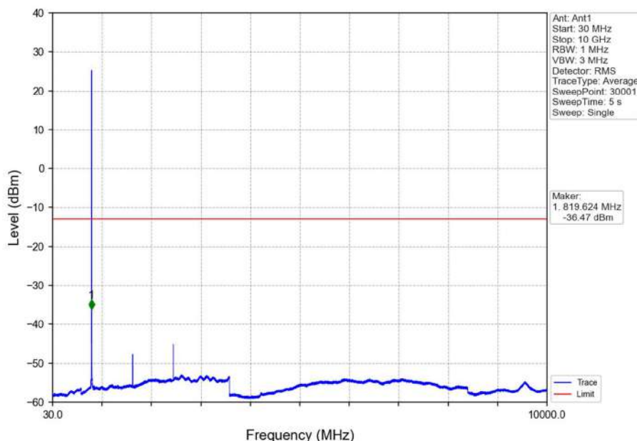
Band26a_1.4MHz_QPSK_HCH_823.3MHz_RB_1_0_NTNV
