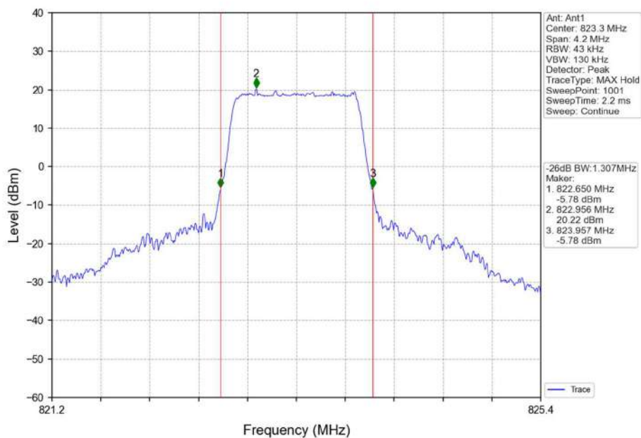
Band26a_1.4MHz_16QAM_HCH_823.3MHz_RB_6_0_NTNV
