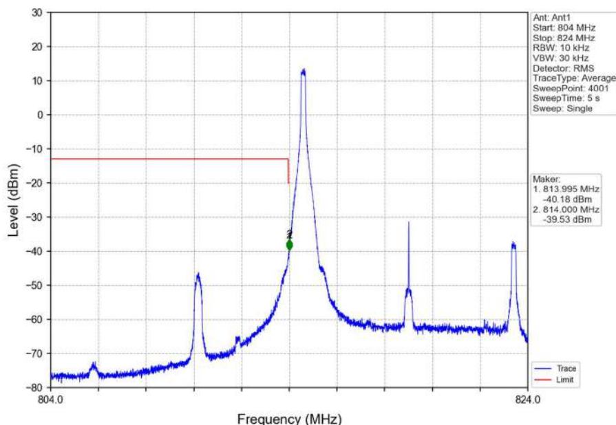
Band26a_10MHz_16QAM_LCH_819MHz_RB_1_0_NTNV
