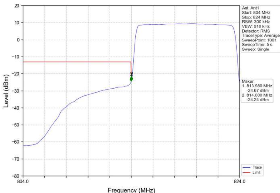
Band26a_10MHz_16QAM_LCH_819MHz_RB_50_0_NTNV
