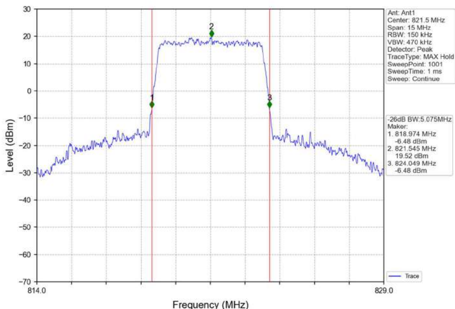
Band26a_5MHz_16QAM_HCH_821.5MHz_RB_25_0_NTNV
