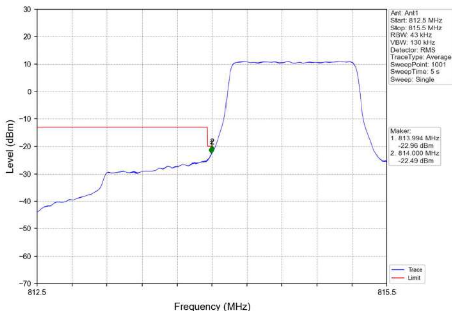
Band26a_1.4MHz_QPSK_LCH_814.7MHz_RB_6_0_NTNV
