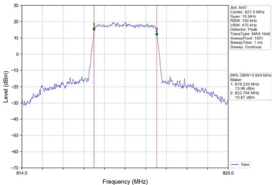
Band26a_5MHz_16QAM_HCH_821.5MHz_RB_25_0_NTNV
