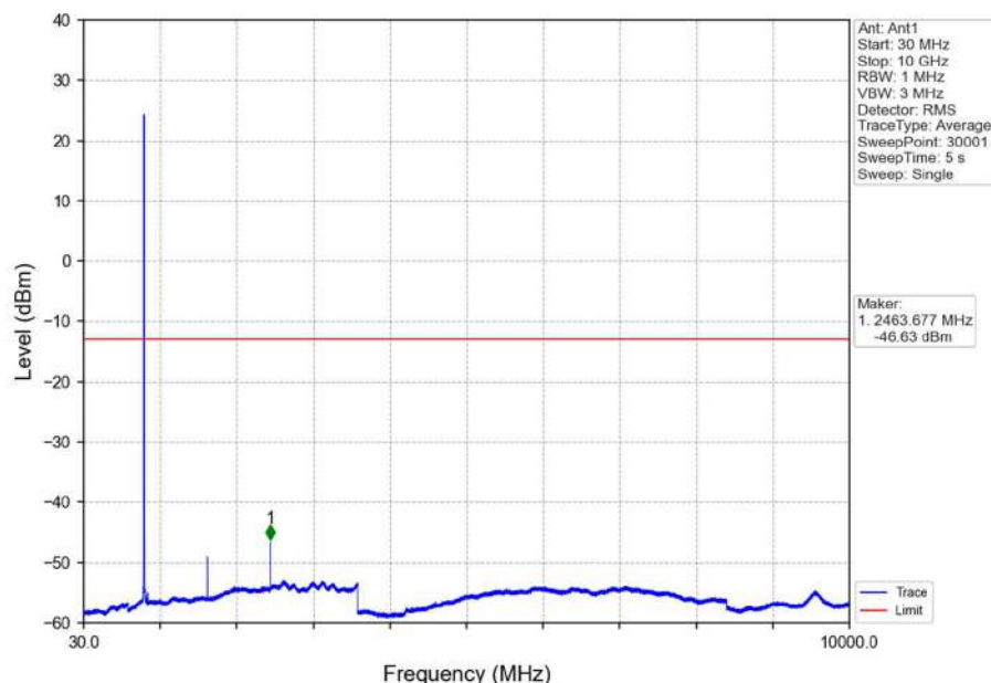
Band26a_3MHz_16QAM_HCH_822.5MHz_RB_1_0_NTNV
