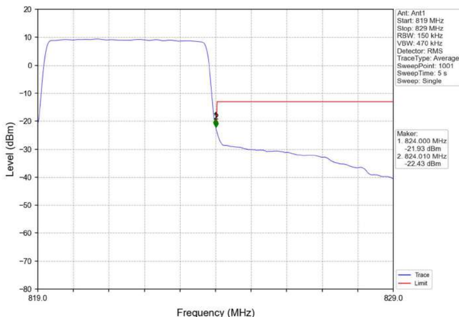
Band26a_5MHz_16QAM_HCH_821.5MHz_RB_25_0_NTNV
