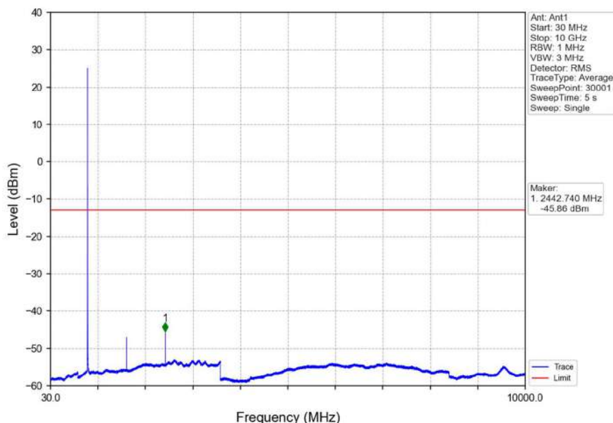
Band26a_3MHz_QPSK_LCH_815.5MHz_RB_1_0_NTNV
