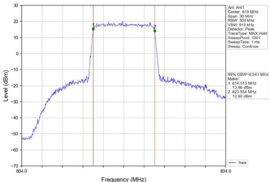
Band26a_10MHz_16QAM_LCH_819MHz_RB_50_0_NTNV
