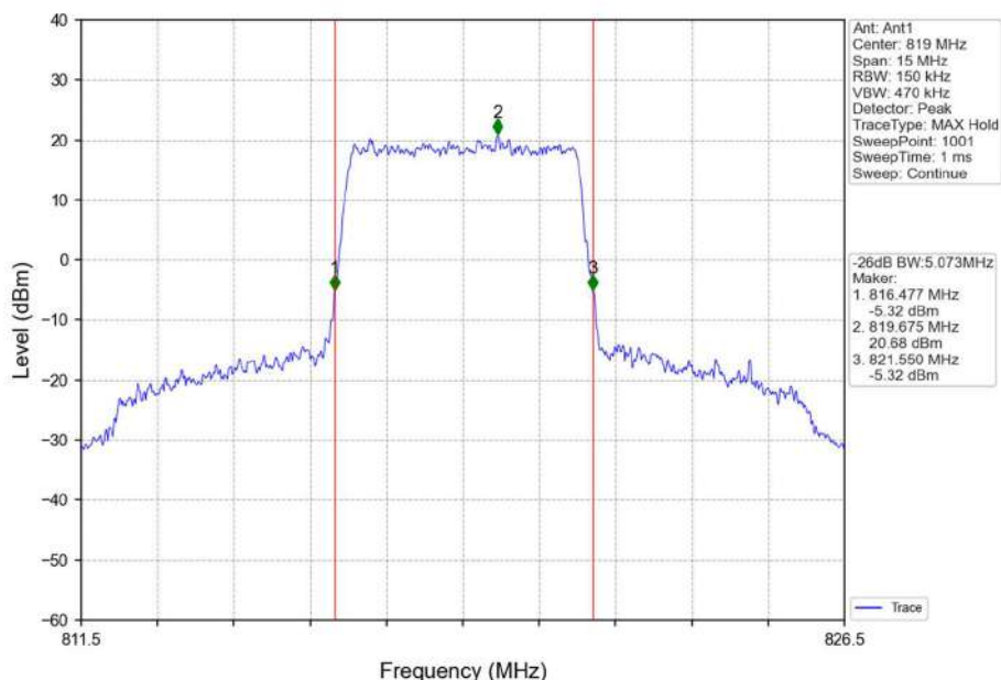
Band26a_5MHz_QPSK_MCH_819MHz_RB_25_0_NTNV
