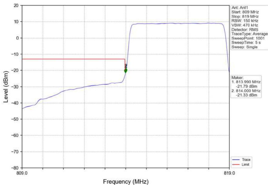
Band26a_5MHz_16QAM_LCH_816.5MHz_RB_25_0_NTNV
