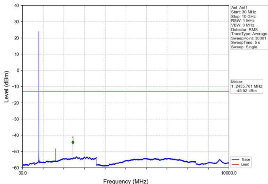
Band26a_1.4MHz_16QAM_MCH_819MHz_RB_1_0_NTNV
