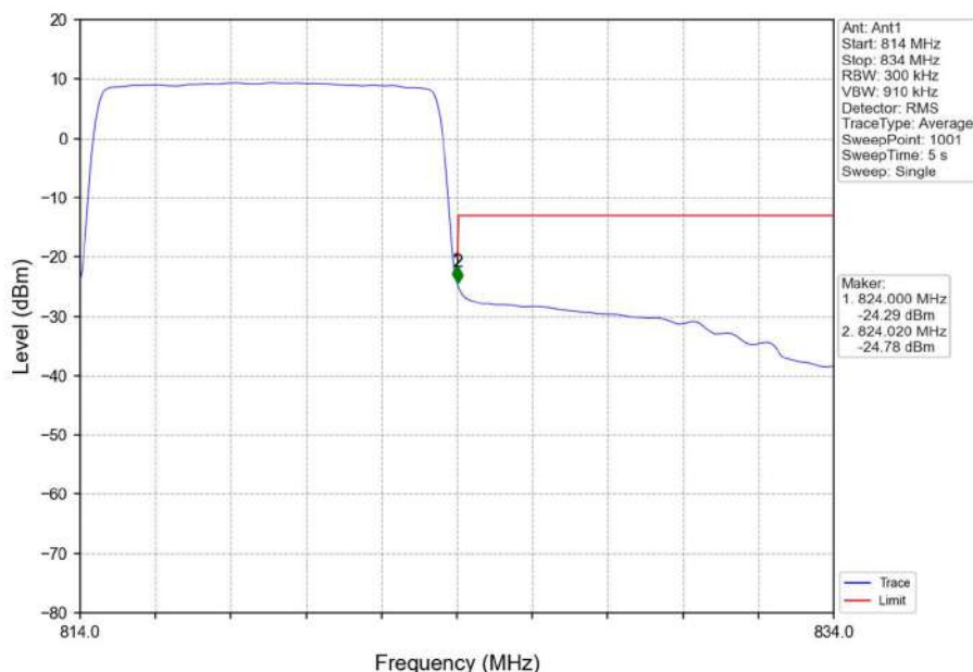
Band26a_10MHz_16QAM_HCH_819MHz_RB_50_0_NTNV
