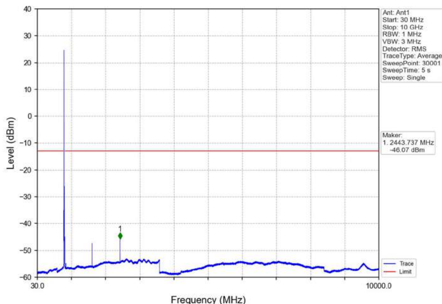
Band26a_10MHz_16QAM_HCH_819MHz_RB_1_0_NTNV
