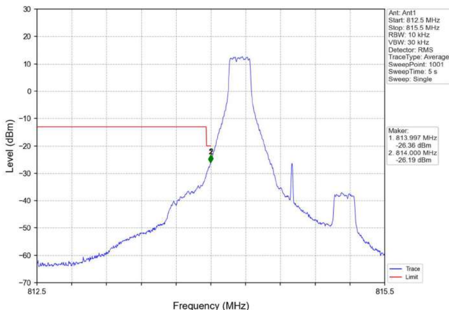
Band26a_1.4MHz_16QAM_LCH_814.7MHz_RB_1_0_NTNV
