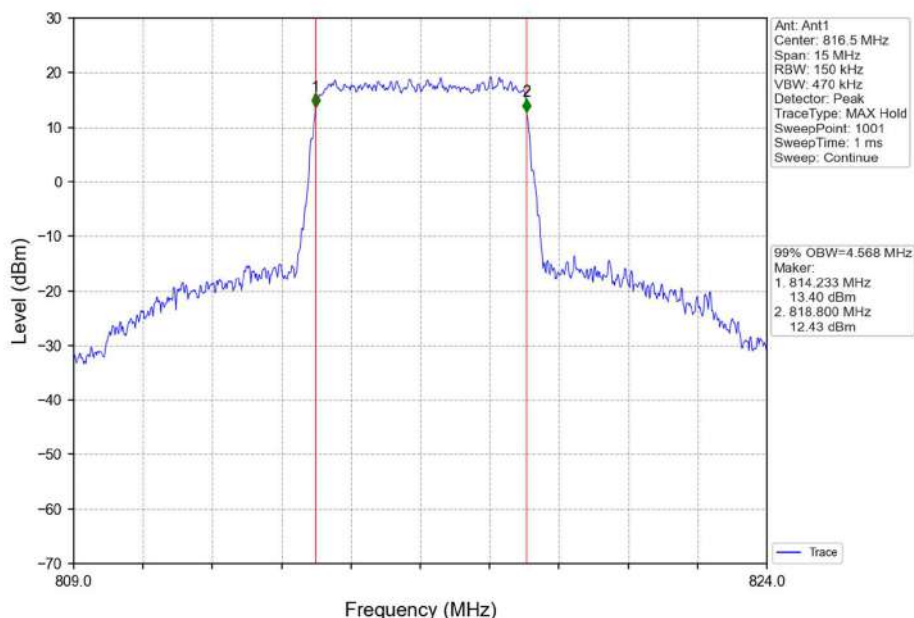
Band26a_5MHz_16QAM_LCH_816.5MHz_RB_25_0_NTNV
