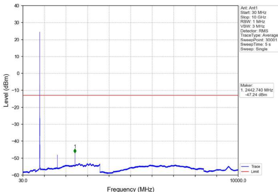
Band26a_5MHz_16QAM_LCH_816.5MHz_RB_1_0_NTNV
