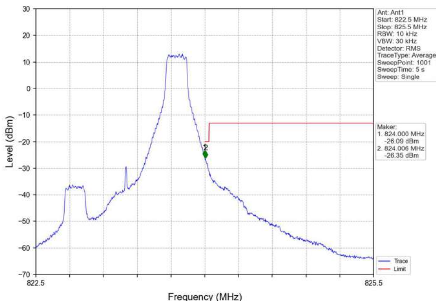
Band26a_1.4MHz_16QAM_HCH_823.3MHz_RB_1_5_NTNV
