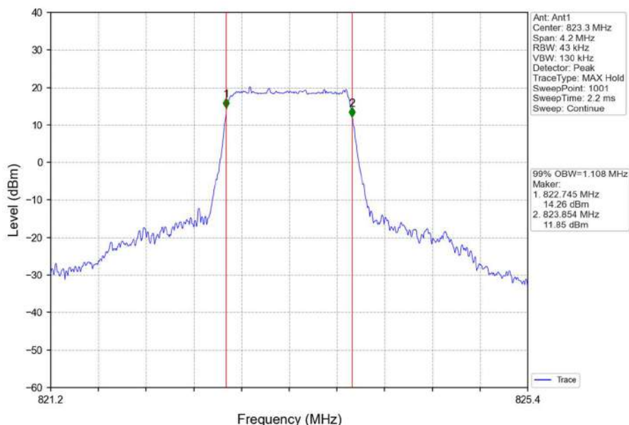
Band26a_1.4MHz_16QAM_HCH_823.3MHz_RB_6_0_NTNV
