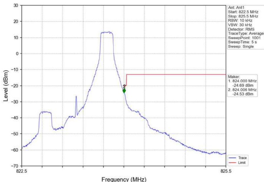
Band26a_1.4MHz_QPSK_HCH_823.3MHz_RB_1_5_NTNV
