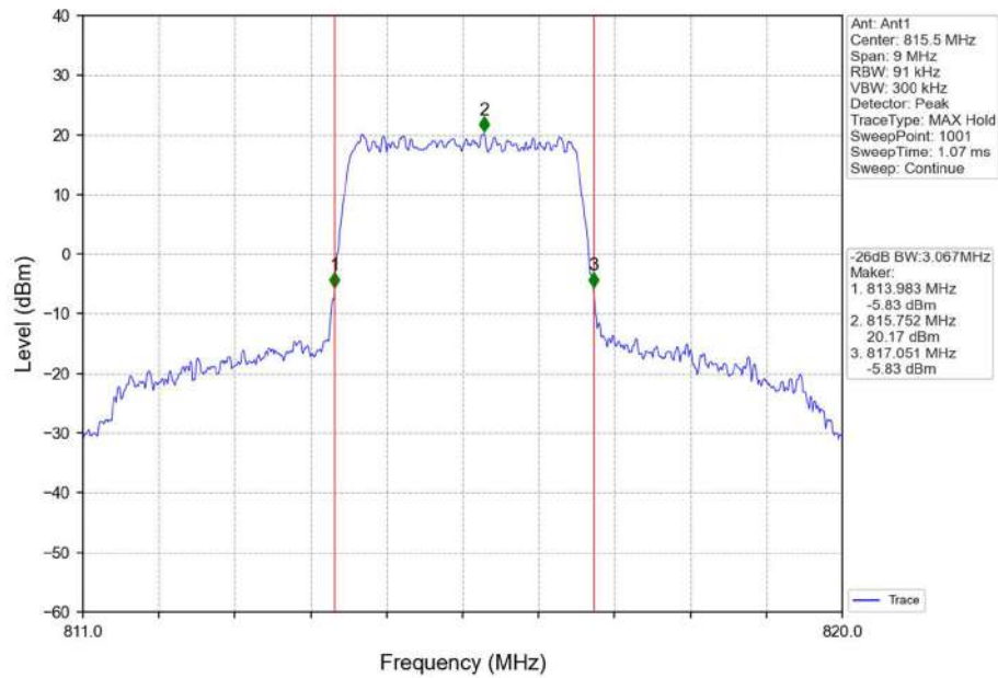
Band26a 3MHz QPSK LCH 815.5MHz RB 15 0 NTN
