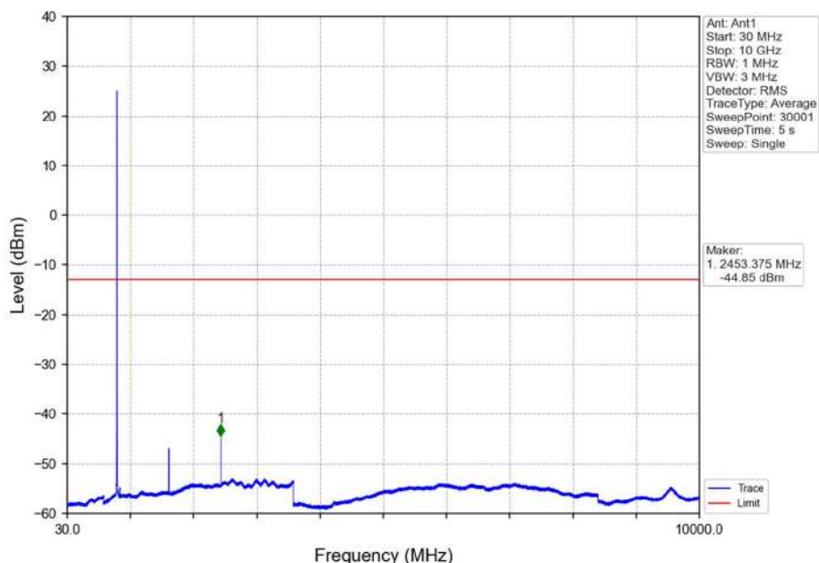
Band26a_3MHz_QPSK_MCH_819MHz_RB_1_0_NTNV
