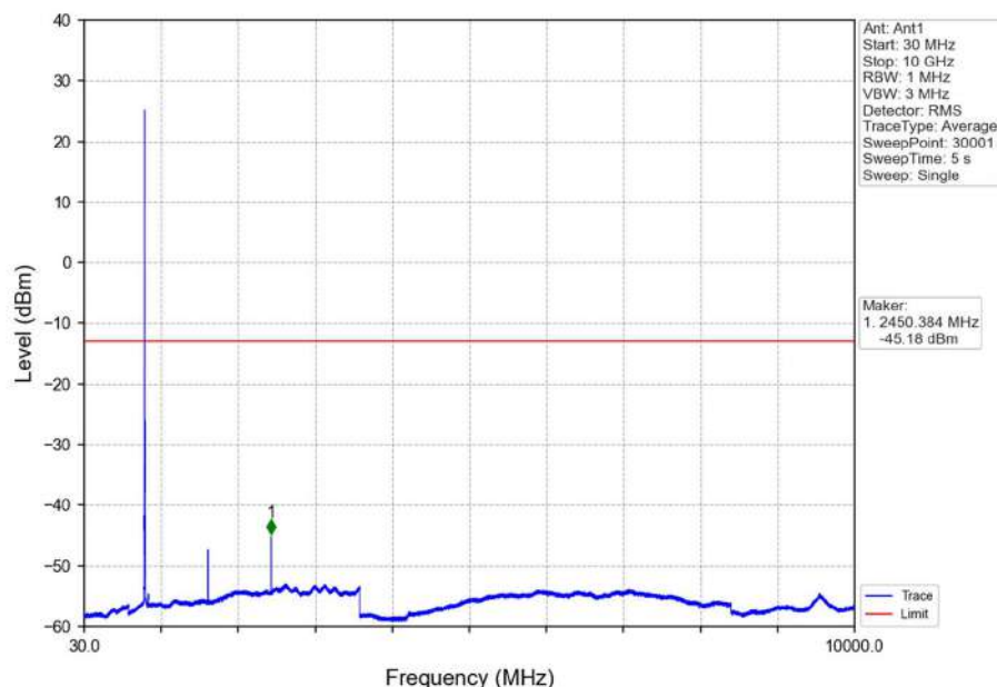
Band26a_5MHz_QPSK_MCH_819MHz_RB_1_0_NTNV
