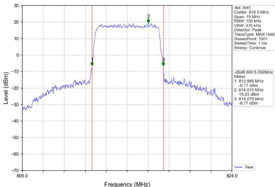
Band26a_5MHz_16QAM_LCH_816.5MHz_RB_25_0_NTNV
