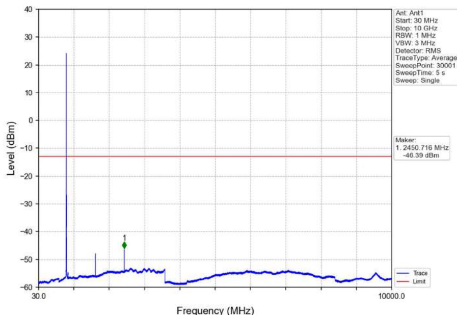
Band26a_5MHz_16QAM_MCH_819MHz_RB_1_0_NTNV
