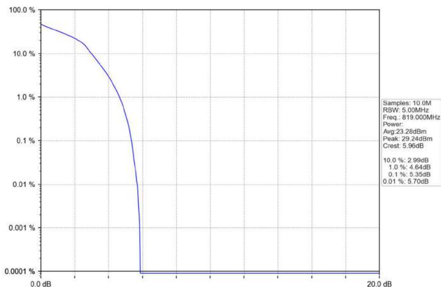
Band26a_1.4MHz_16QAM_MCH_819MHz_RB_6_0_NTNV
