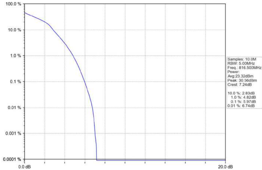
Band26a_5MHz_16QAM_LCH_816.5MHz_RB_25_0_NTNV
