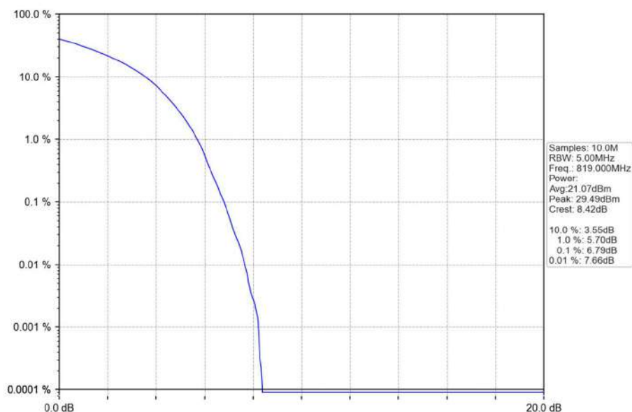
Band26a_10MHz_16QAM_HCH_819MHz_RB_50_0_NTNV
