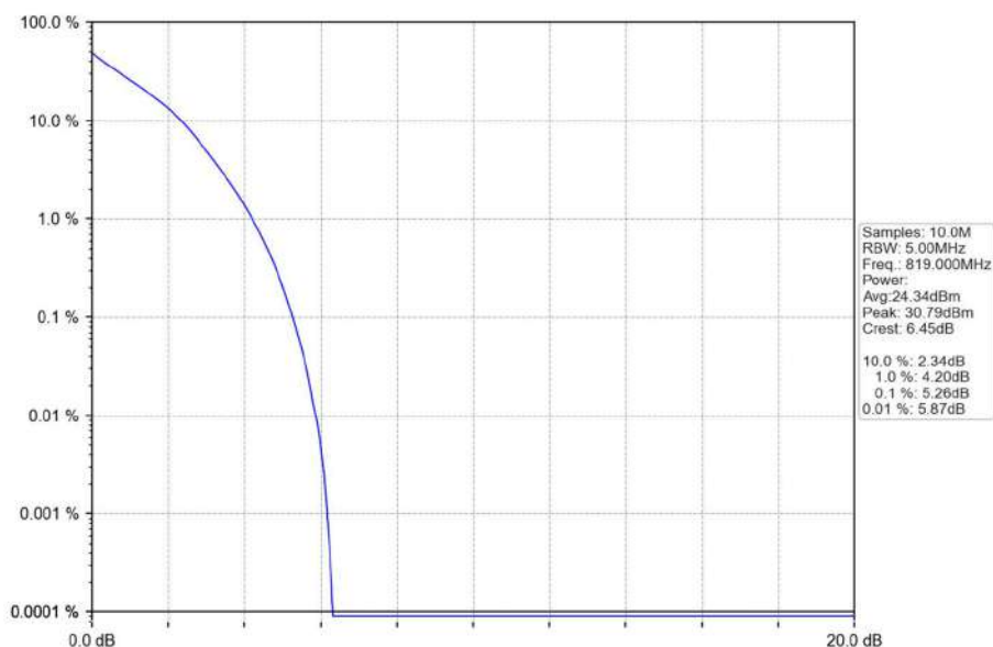
Band26a_5MHz_QPSK_MCH_819MHz_RB_25_0_NTNV
