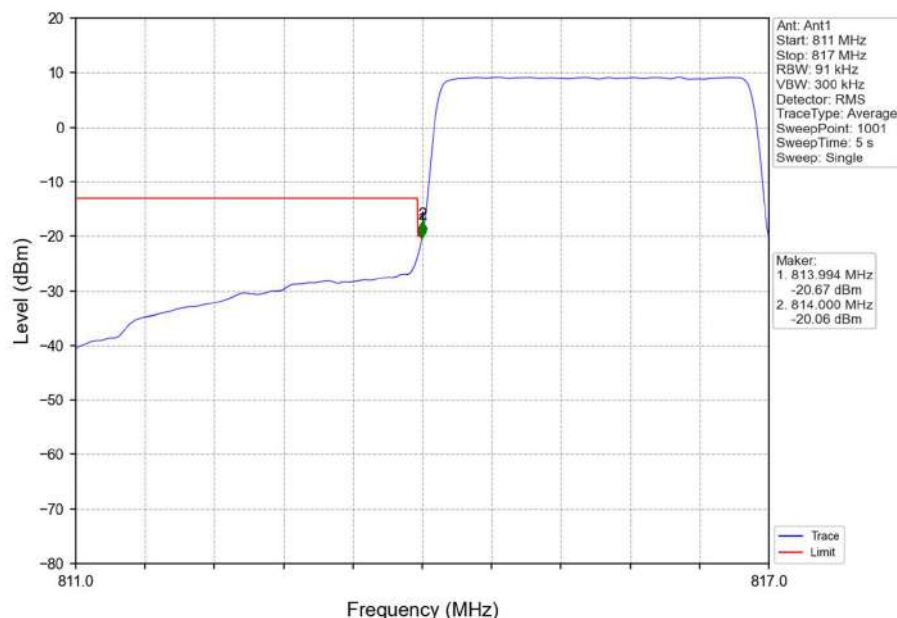
Band26a_3MHz_16QAM_LCH_815.5MHz_RB_15_0_NTNV
