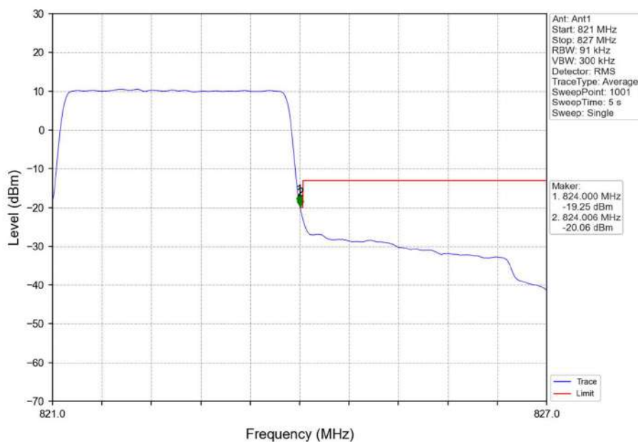
Band26a 3MHz QPSK HCH 822.5MHz RB 15 0 NTN
