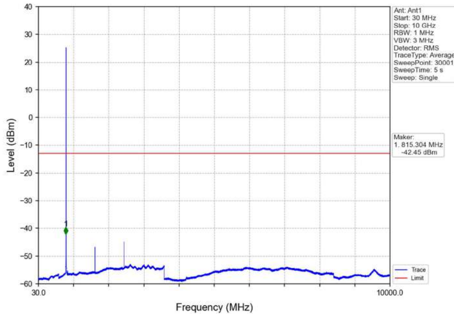
Band26a_1.4MHz_QPSK_MCH_819MHz_RB_1_0_NTNV
