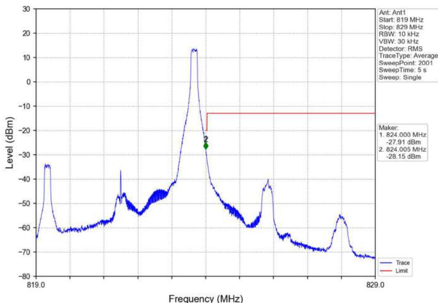
Band26a_5MHz_QPSK_HCH_821.5MHz_RB_1_24_NTNV
