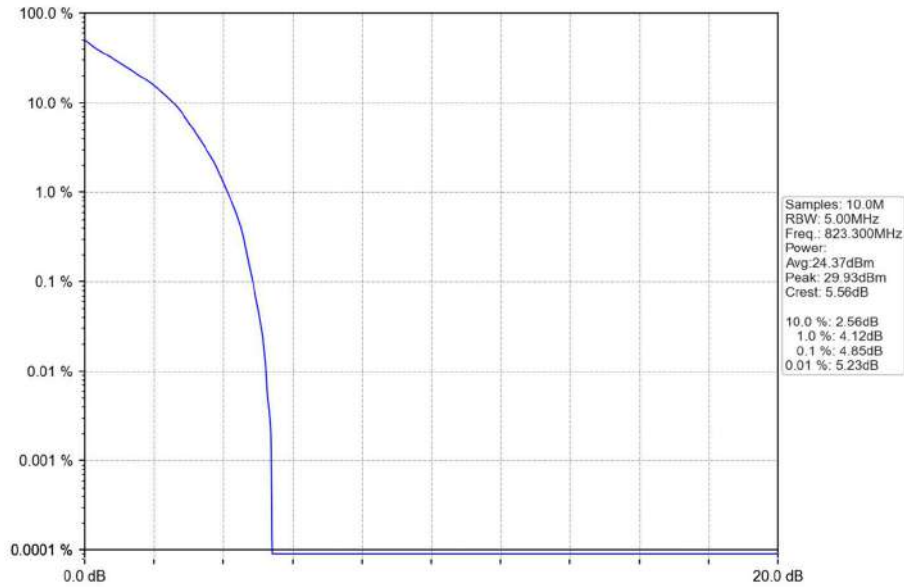
Band26a_1.4MHz_QPSK_HCH_823.3MHz_RB_6_0_NTNV
