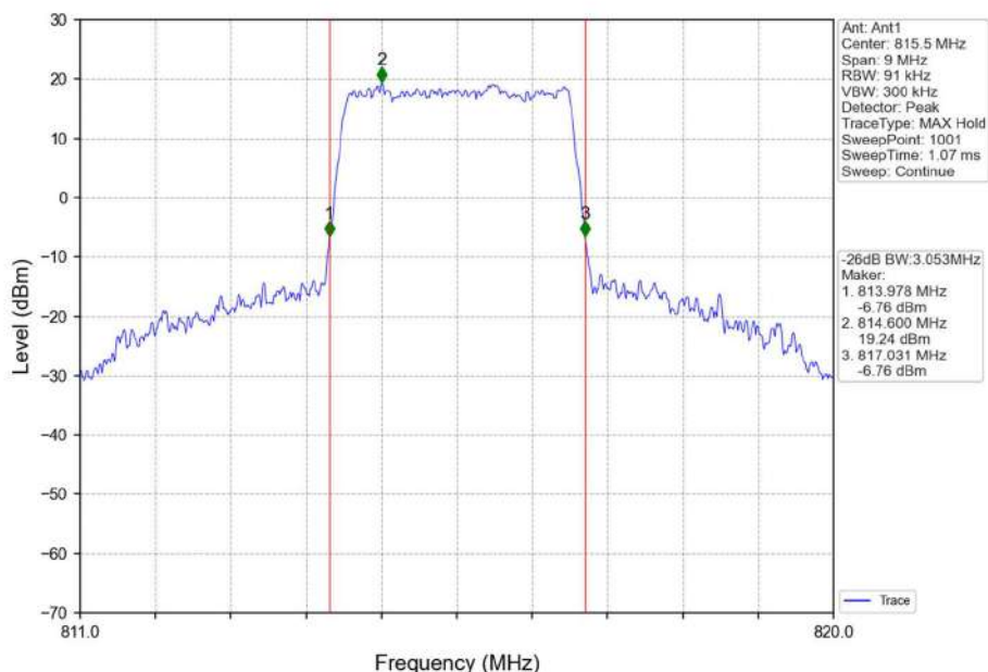
Band26a_3MHz_16QAM_LCH_815.5MHz_RB_15_0_NTNV
