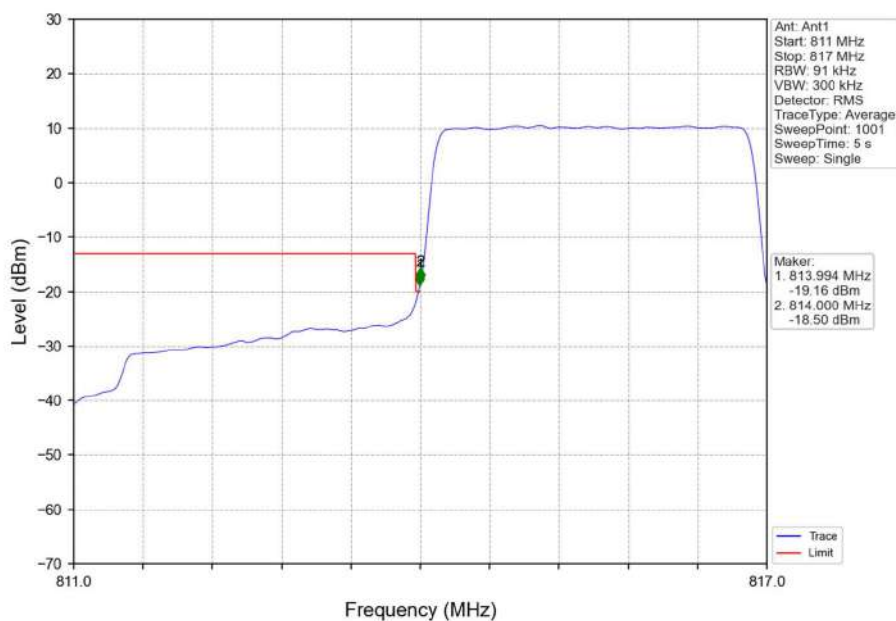
Band26a 3MHz QPSK LCH 815.5MHz RB 15 0 NTNV
