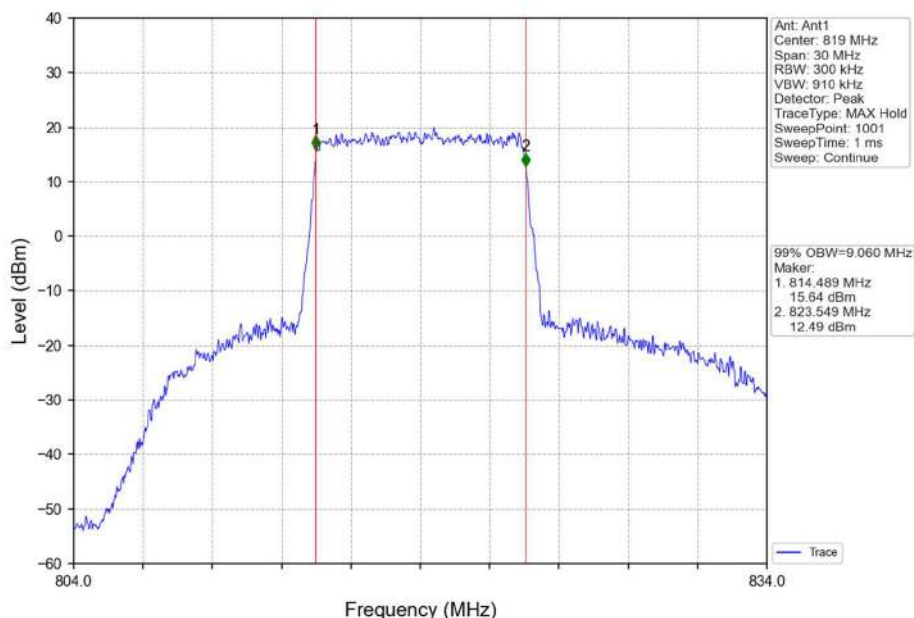
Band26a_10MHz_16QAM_HCH_819MHz_RB_50_0_NTNV
