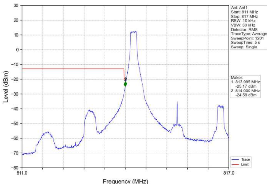
Band26a_3MHz_16QAM_LCH_815.5MHz_RB_1_0_NTNV
