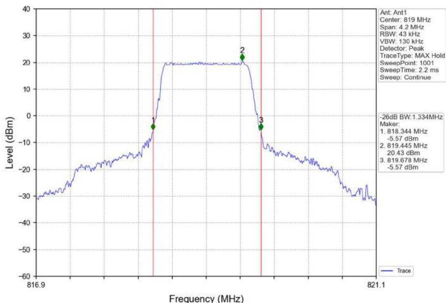
Band26a_1.4MHz_QPSK_MCH_819MHz_RB_6_0_NTNV
