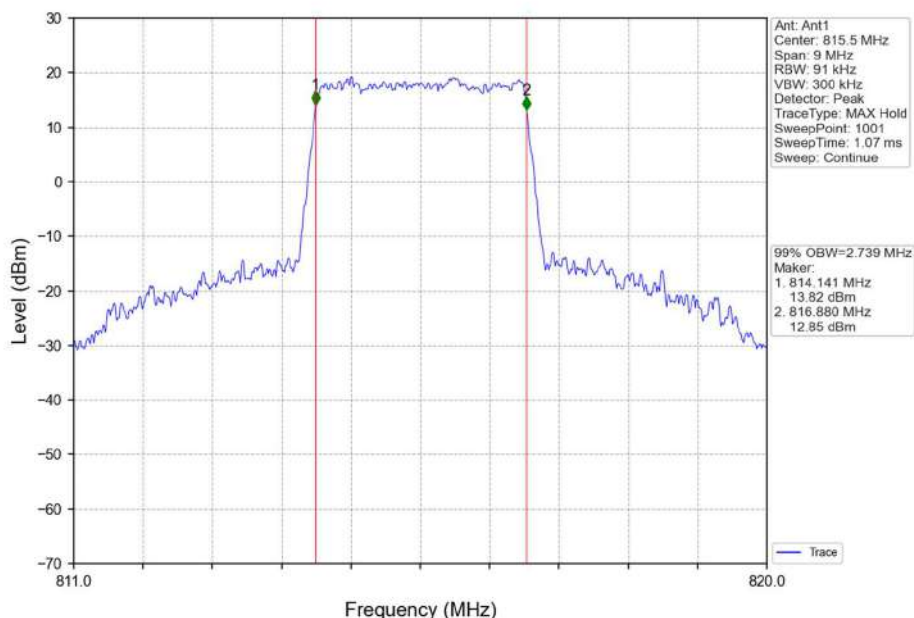
Band26a_3MHz_16QAM_LCH_815.5MHz_RB_15_0_NTNV
