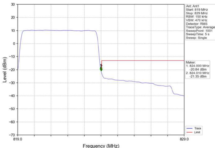
Band26a_5MHz_QPSK_HCH_821.5MHz_RB_25_0_NTNV
