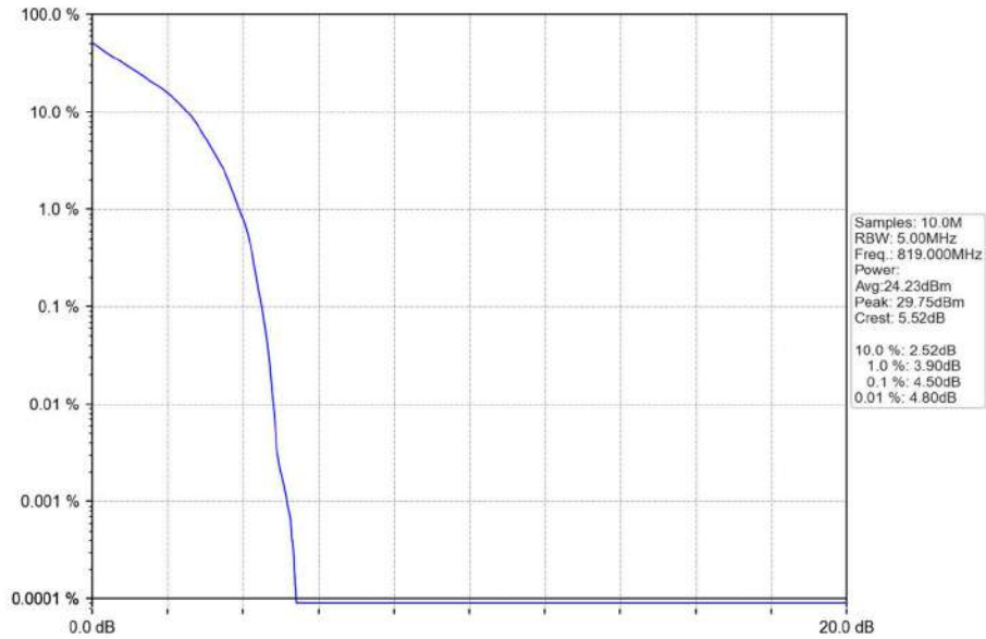
Band26a_1.4MHz_QPSK_MCH_819MHz_RB_6_0_NTNV
