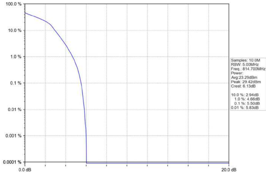
Band26a_1.4MHz_16QAM_LCH_814.7MHz_RB_6_0_NTNV
