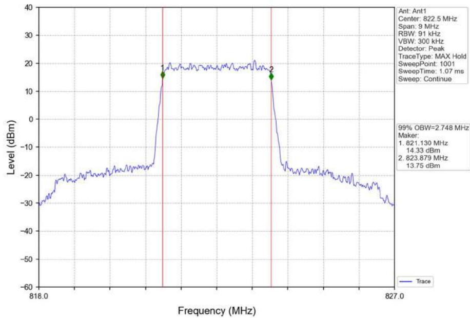
Band26a 3MHz QPSK HCH 822.5MHz RB 15 0 NTN
