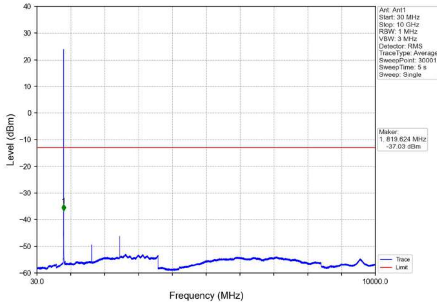
Band26a_1.4MHz_16QAM_HCH_823.3MHz_RB_1_0_NTNV
