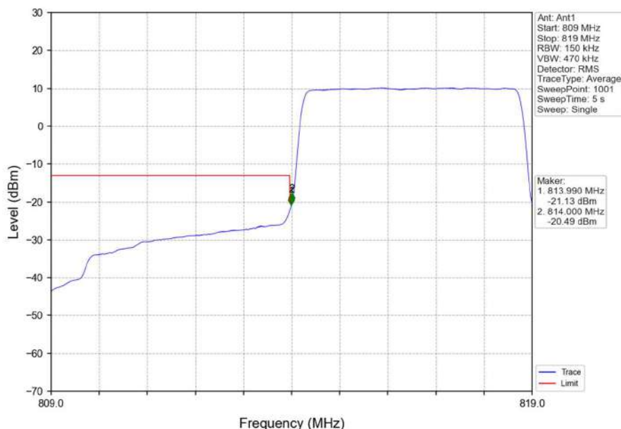
Band26a_5MHz_QPSK_LCH_816.5MHz_RB_25_0_NTNV
