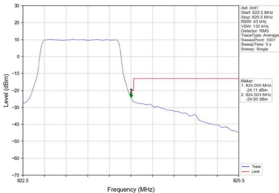
Band26a_1.4MHz_16QAM_HCH_823.3MHz_RB_6_0_NTNV
