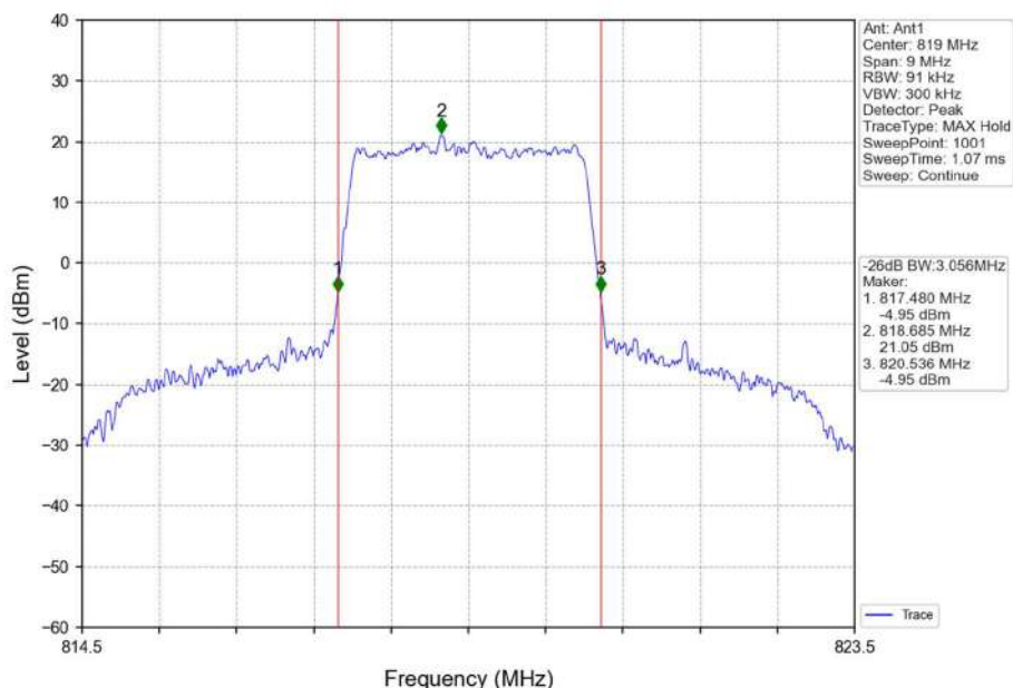
Band26a_3MHz_QPSK_MCH_819MHz_RB_15_0_NTNV
