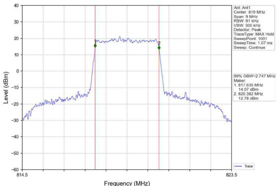
Band26a_3MHz_QPSK_MCH_819MHz_RB_15_0_NTNV
