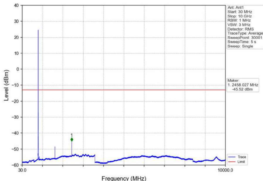
Band26a_5MHz_16QAM_HCH_821.5MHz_RB_1_0_NTNV
