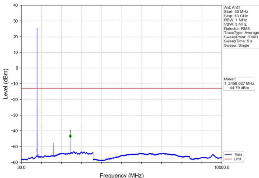
Band26a_5MHz_QPSK_HCH_821.5MHz_RB_1_0_NTNV
