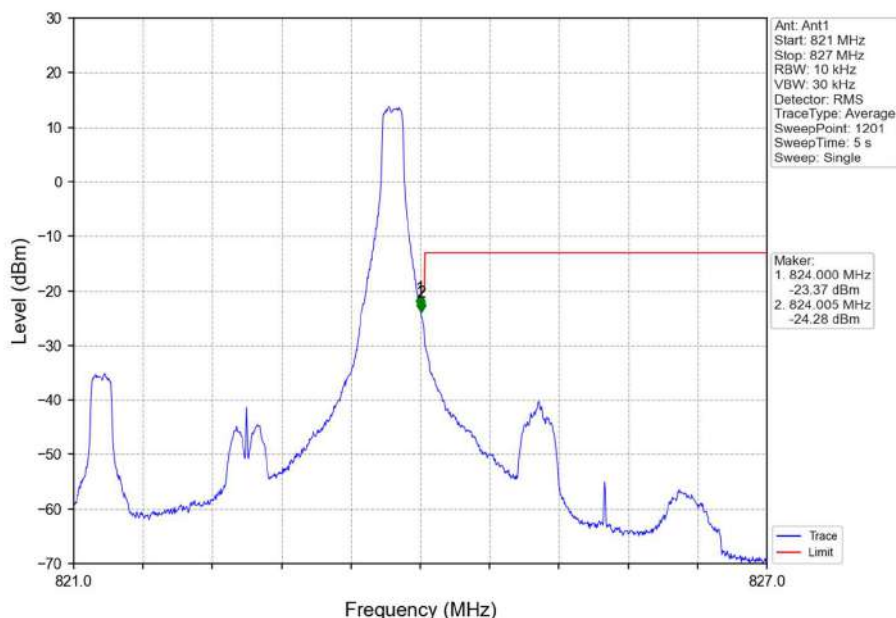
Band26a_3MHz_QPSK_HCH_822.5MHz_RB_1_14_NTNV
