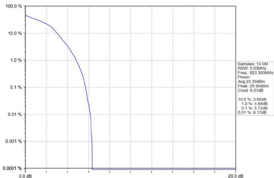
Band26a_1.4MHz_16QAM_HCH_823.3MHz_RB_6_0_NTNV
