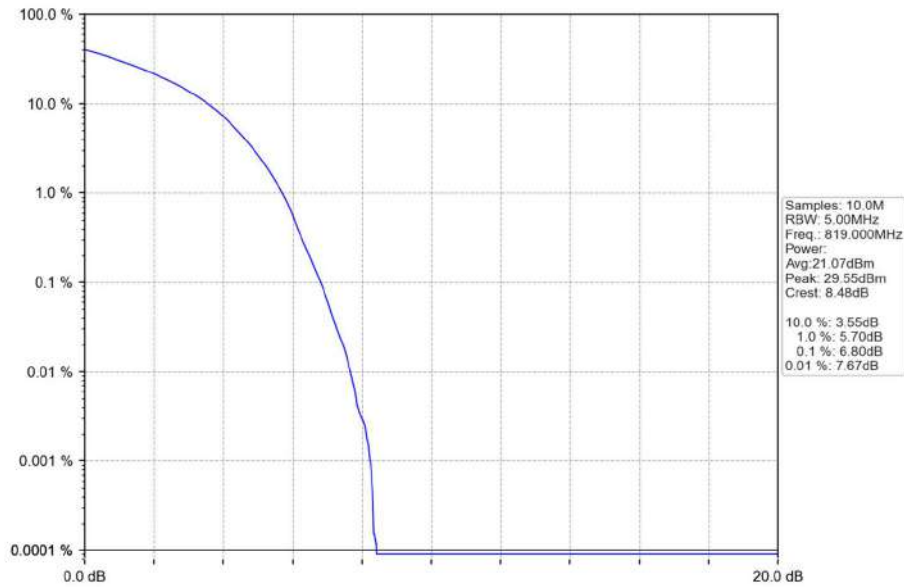
Band26a 10MHz 16QAM MCH 819MHz RB 50 0 NTNV
