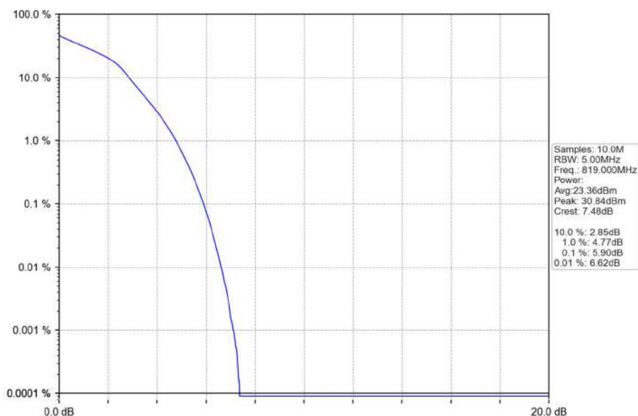
Band26a_5MHz_16QAM_MCH_819MHz_RB_25_0_NTNV
