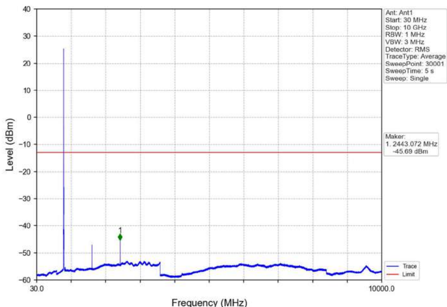
Band26a_5MHz_QPSK_LCH_816.5MHz_RB_1_0_NTNV
