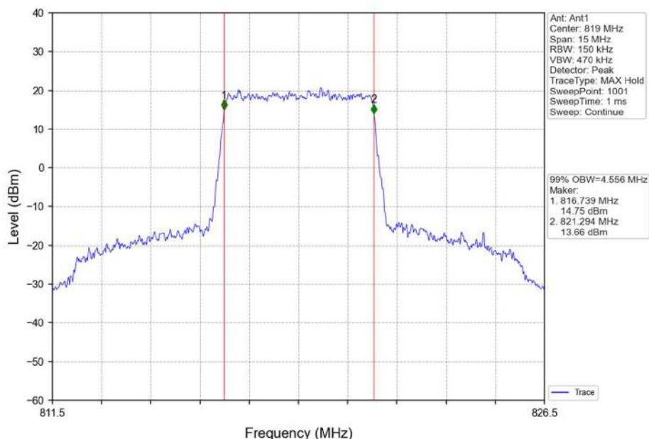
Band26a_5MHz_QPSK_MCH_819MHz_RB_25_0_NTNV
