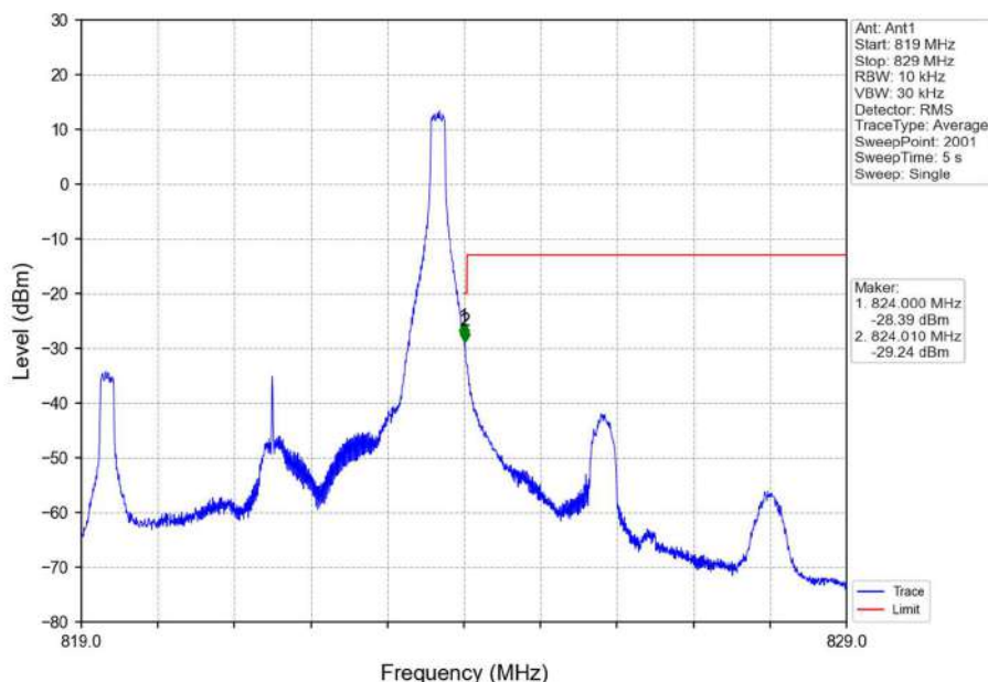
Band26a_5MHz_16QAM_HCH_821.5MHz_RB_1_24_NTNV
