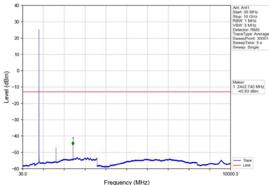
Band26a_1.4MHz_QPSK_LCH_814.7MHz_RB_1_0_NTNV
