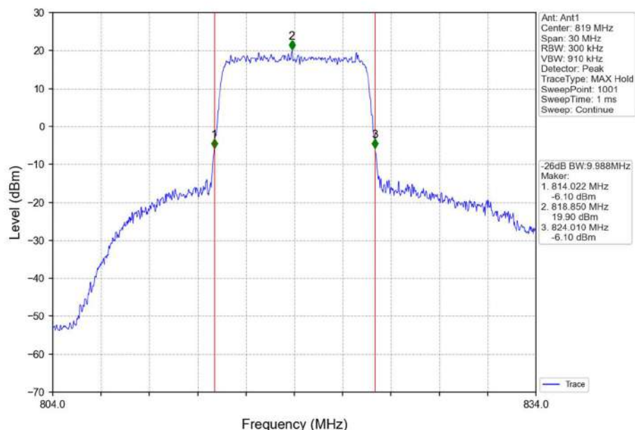
Band26a_10MHz_16QAM_LCH_819MHz_RB_50_0_NTNV
