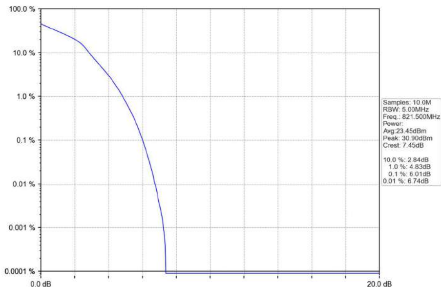
Band26a_5MHz_16QAM_HCH_821.5MHz_RB_25_0_NTNV
