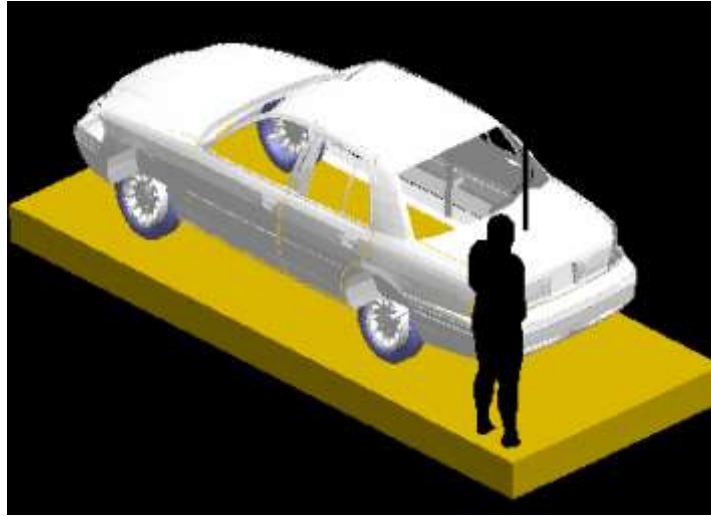
Figure 3: Bystander model exposed to a trunk-mount antenna: XFDTD geometry. Bystander is located at the back corner of the car replicating the measurement conditions.
