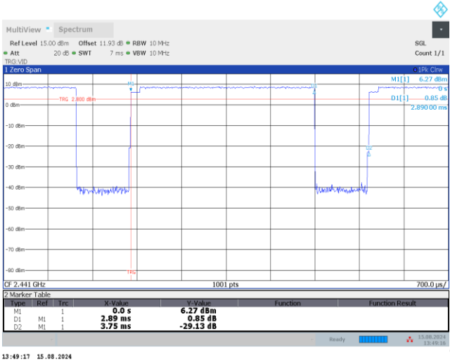
2DH5_2441MHz
