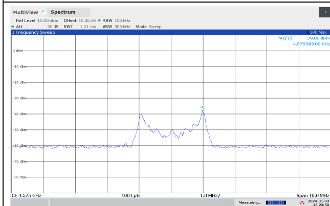
Conducted Emissions 4575 MHz, 915.00 MHz
