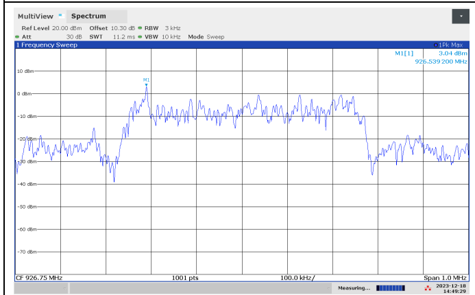
PSD, 926.75 MHz
