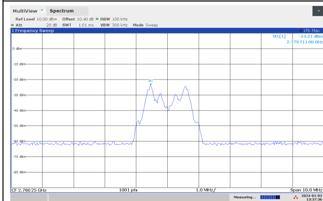
Conducted Emissions 2780.25 MHz, 926.75 MHz
