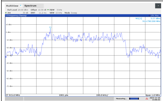
PSD, 915.00 MHz
