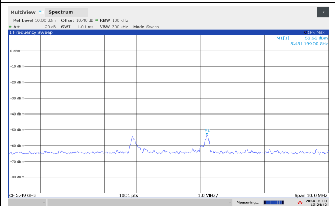
Conducted Emissions 5490 MHz, 915.00 MHz
