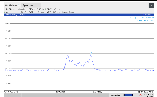
Conducted Emissions 3707 MHz, 926.75 MHz
