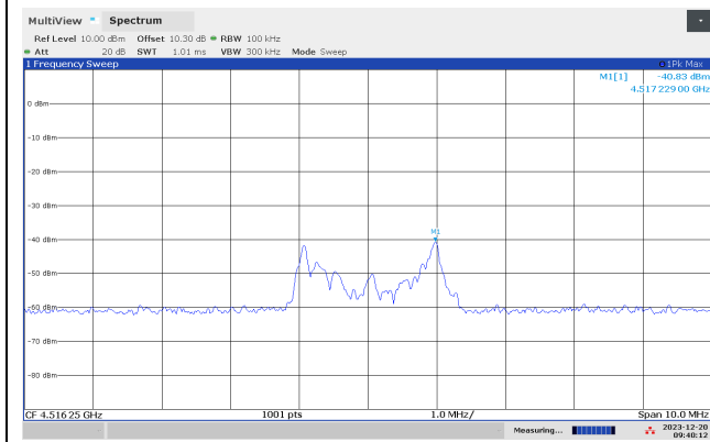
Conducted Emissions 4516.25 MHz, 903.25 MHz
