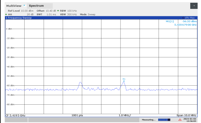
Conducted Emissions 5419.5 MHz, 903.25 MHz
