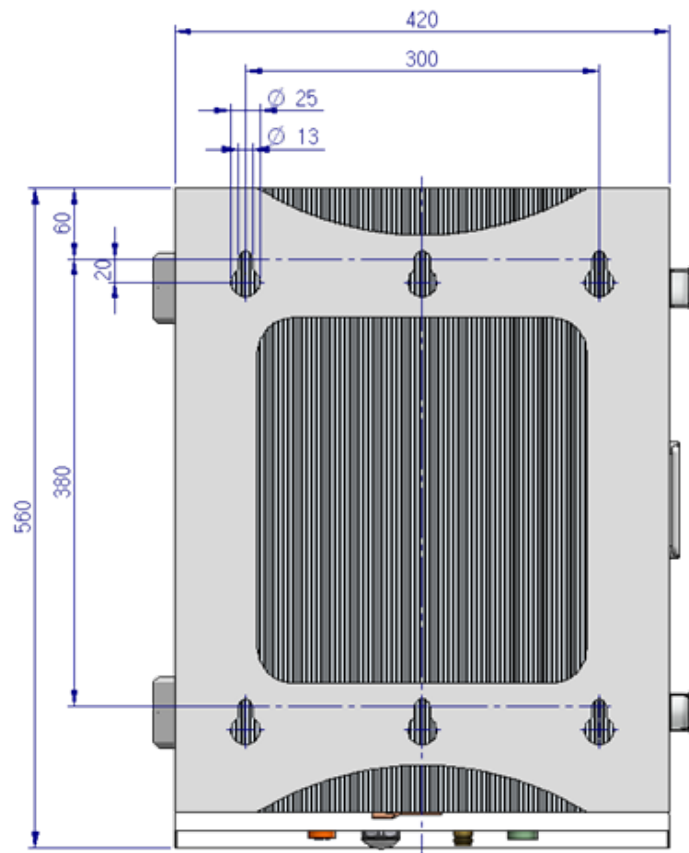
Figure 3.2 – How to install ROU
