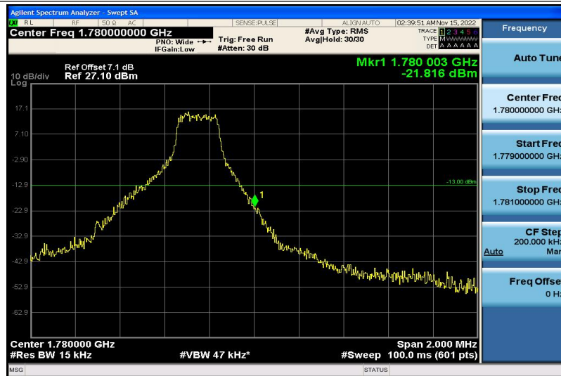
Band66-1.4MHz-QPSK-132665-1RB#5
