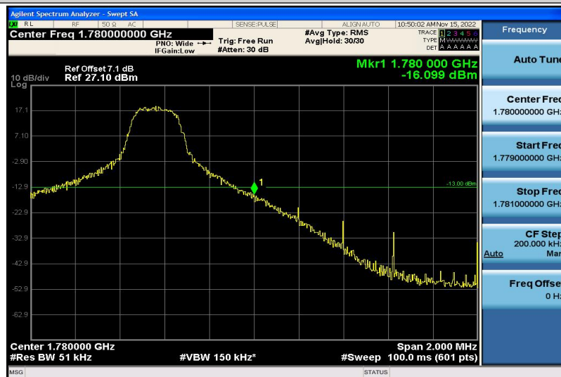
Band66-5MHz-QPSK-132647-1RB#24
