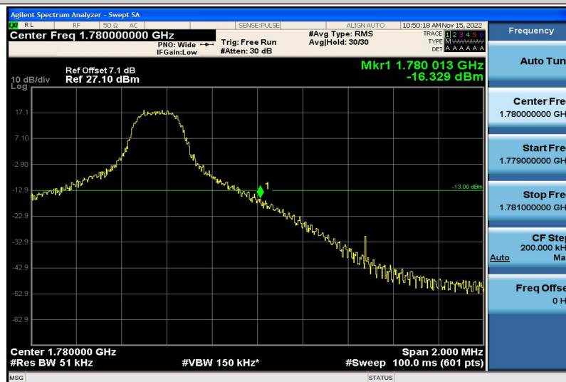
Band66-5MHz-16QAM-132647-1RB#24
