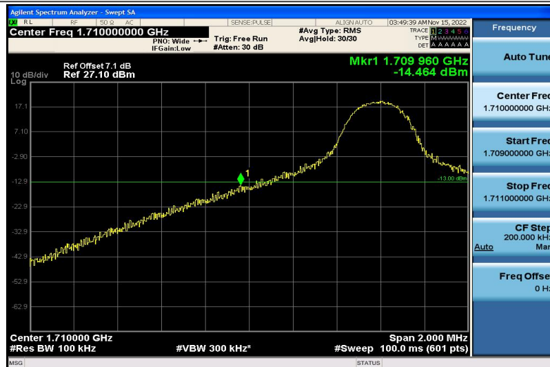
Band66-10MHz-16QAM-132022-1RB#0
