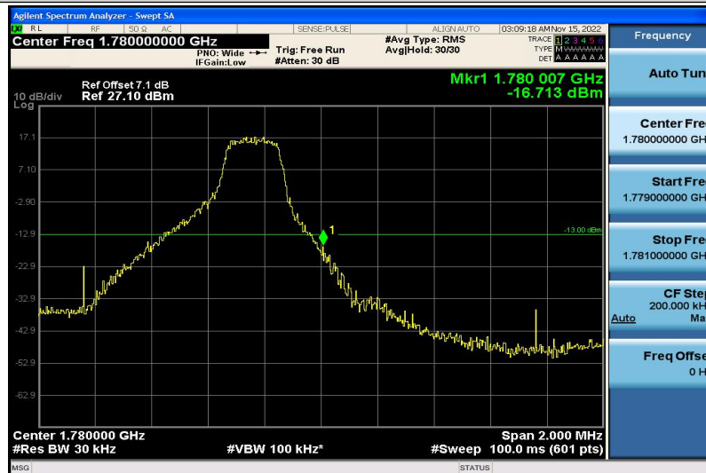
Band66-3MHz-QPSK-132657-1RB#14
