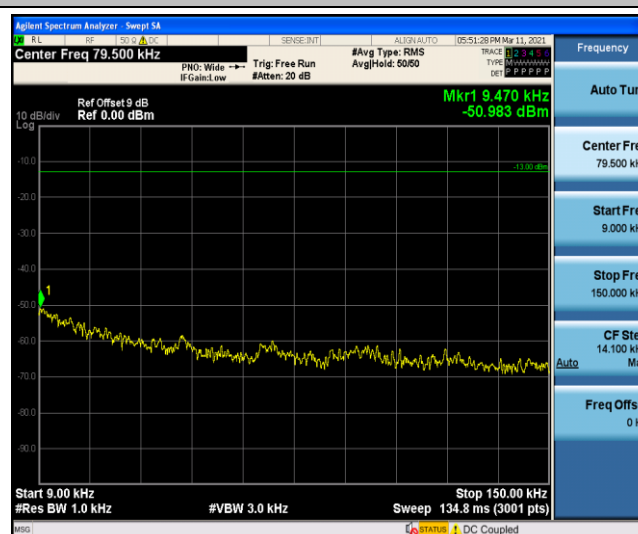
Band 71_15MHz_QPSK_133197_1RB#0
