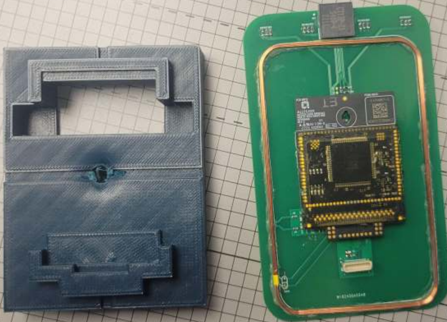
EUT W/ ATTACHED LARGE COIL ANTENNA
