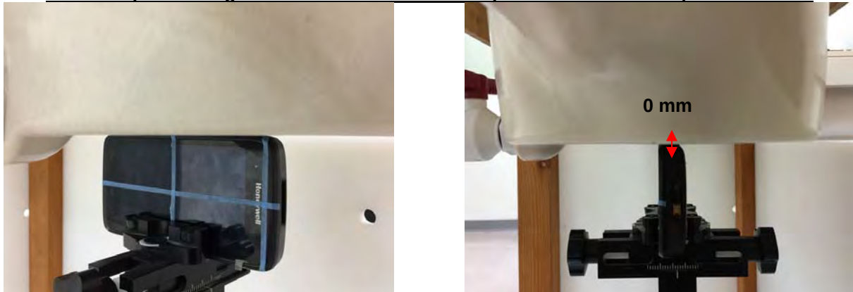
Fig.12 EUT Left side to flat phantom
