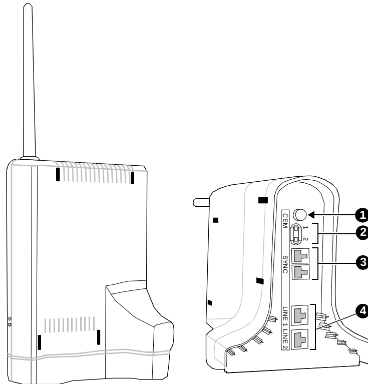
Figure 1. The Dual-Radio Module (DRM)
