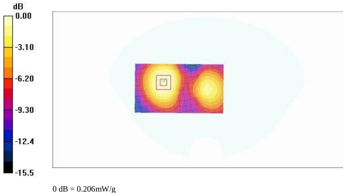
Fig.89 Flat Phantom Body-worn Position 1900MHz GPRS CH810 with the display of the handset toward the phantom
