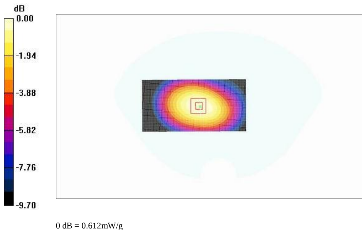
Fig.97 Flat Phantom Hand-worn Position 850MHz GPRS CH128 with the display of the handset toward the phantom
