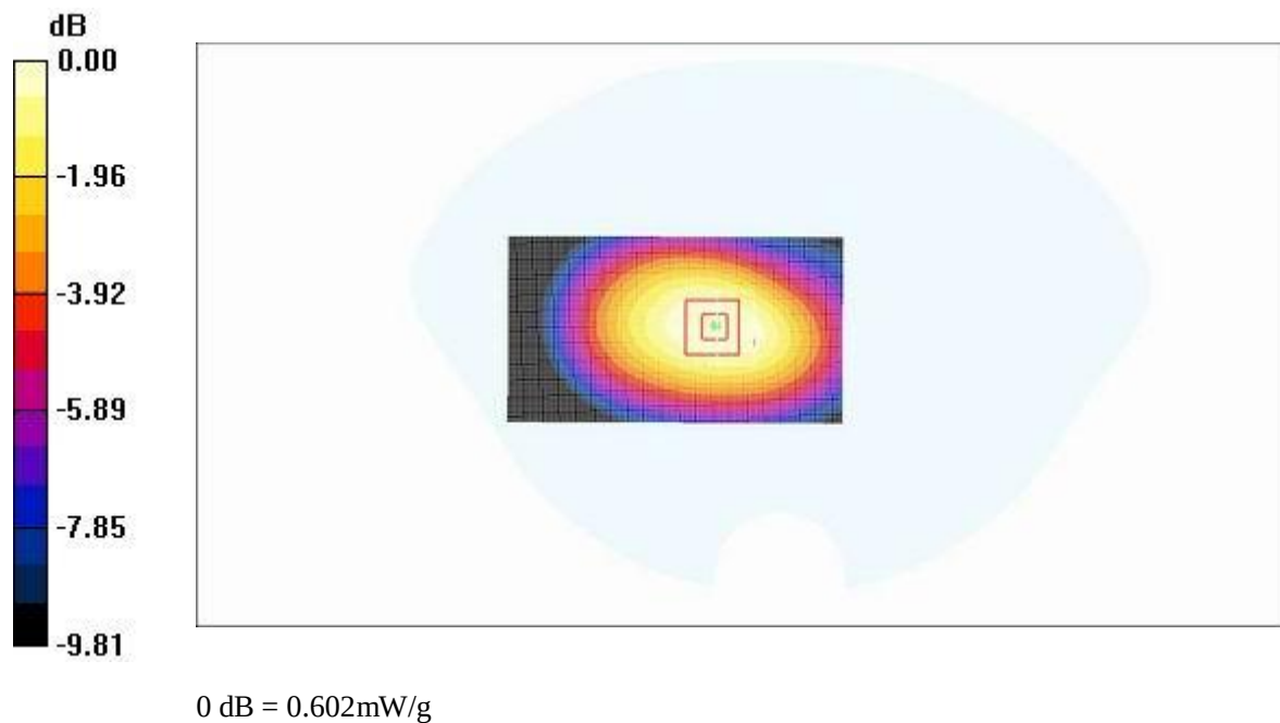
Fig.73 Flat Phantom Body-worn Position 850MHz GPRS CH128 with the display of the handset toward the phantom
