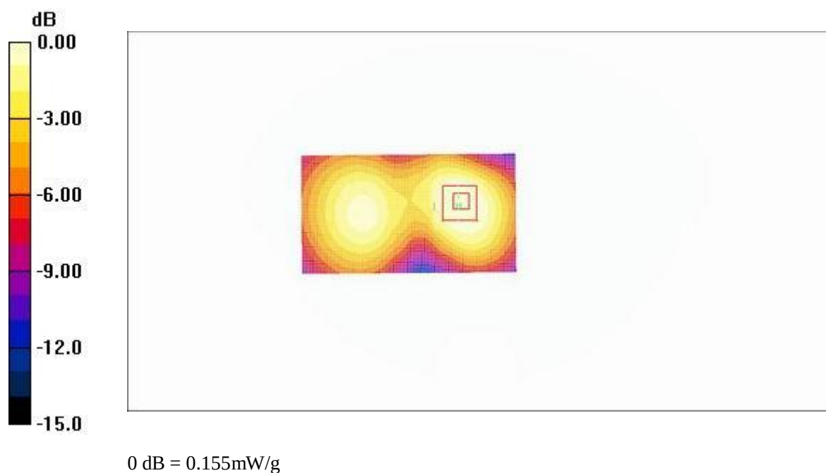
Fig. 71 Flat Phantom Body-worn Position 1900MHz CH810 with the display of the handset toward the ground
