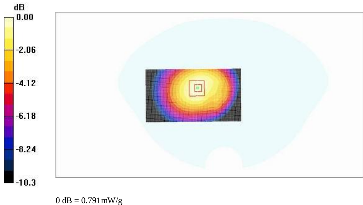
Fig.83 Flat Phantom Body-worn Position 850MHz GPRS CH251 with the display of the handset toward the ground
