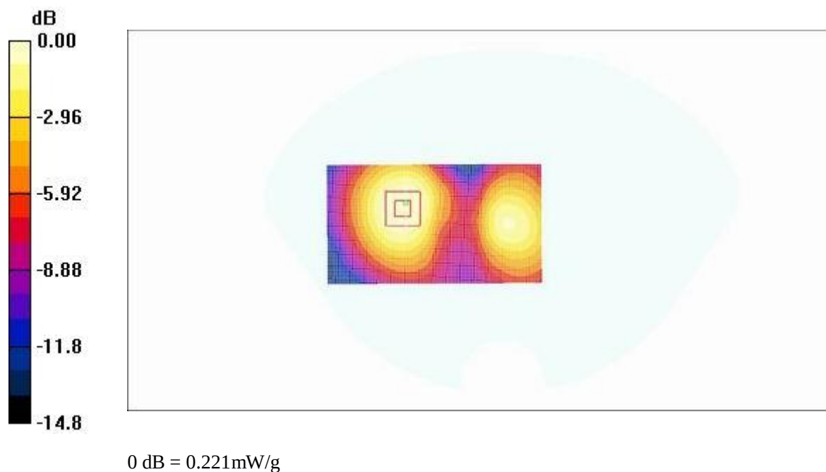
Fig.85 Flat Phantom Body-worn Position 1900MHz GPRS CH512 with the display of the handset toward the phantom
