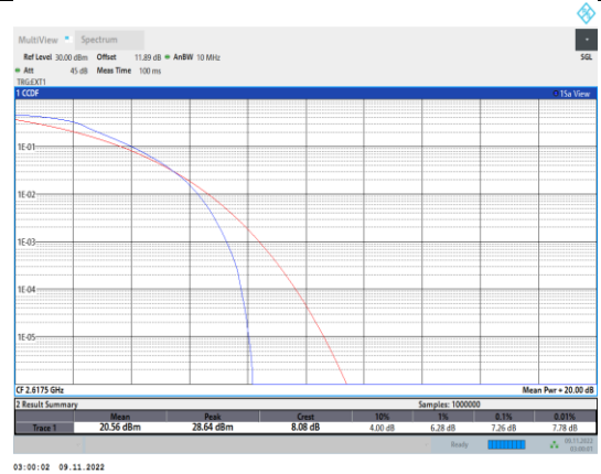
Band38-5MHz-QPSK-38225-25RB#0
