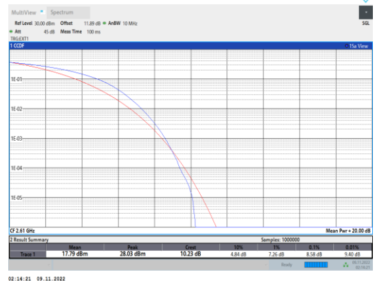
Band38-20MHz-16QAM-38150-100RB#0
