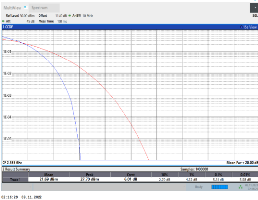
Band7-15MHz-QPSK-21100-75RB#0
