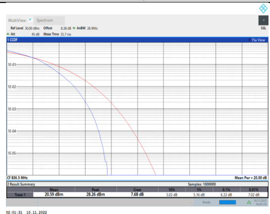
Band26-15MHz-16QAM-26915-75RB#0
