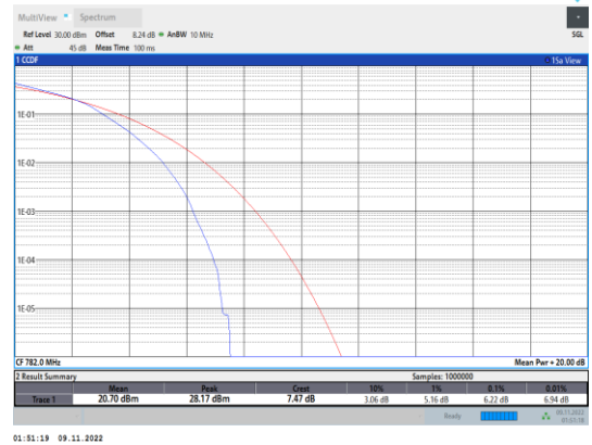
Band13-5MHz-16QAM-23230-25RB#0
