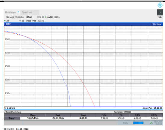
Band7-20MHz-64QAM-21350-100RB#0
