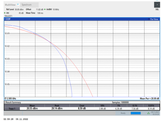
Band38-5MHz-QPSK-38000-25RB#0
