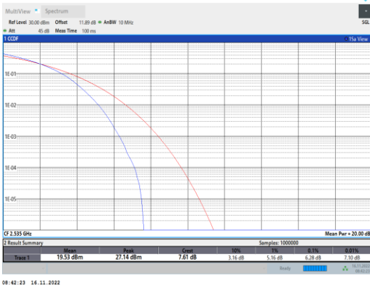
Band7-15MHz-64QAM-21100-75RB#0
