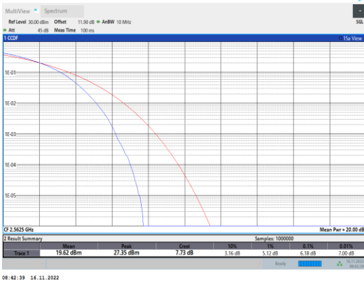
Band7-15MHz-64QAM-21375-75RB#0
