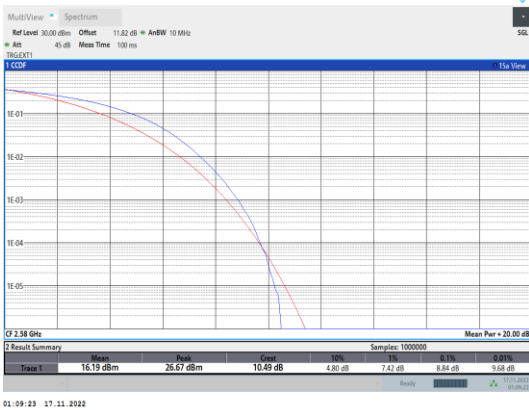
Band38-20MHz-64QAM-37850-100RB#0
