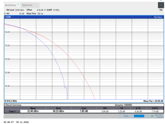
Band26-5MHz-16QAM-26715-25RB#0
