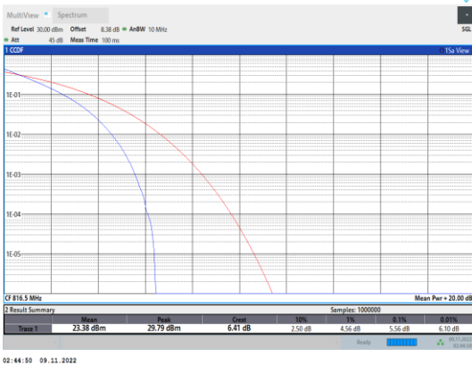
Band26-5MHz-QPSK-26715-25RB#0
