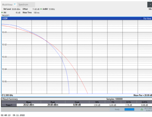
Band38-10MHz-QPSK-38000-50RB#0
