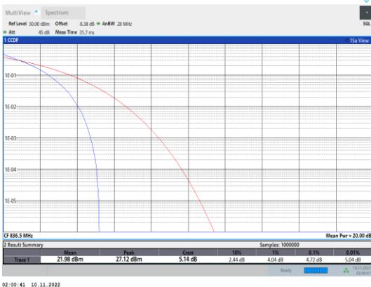
Band26-15MHz-QPSK-26915-1RB#0
