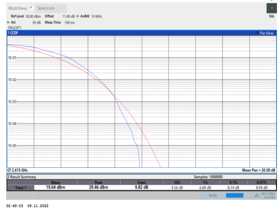
Band38-10MHz-16QAM-38200-50RB#0
