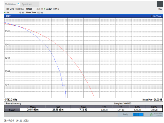
Band13-10MHz-16QAM-23230-50RB#0
