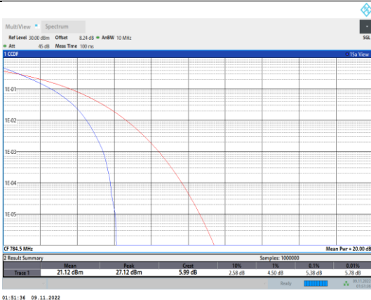
Band13-5MHz-QPSK-23255-25RB#0
