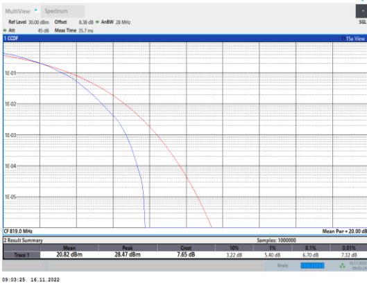
Band26-1.4MHz-64QAM-26740-6RB#0
