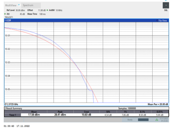
Band38-5MHz-64QAM-37775-25RB#0
