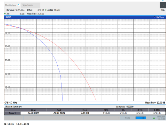
Band26-1.4MHz-16QAM-26697-6RB#0
