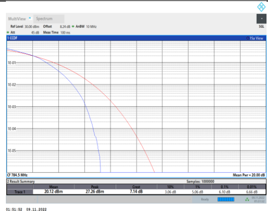
Band13-5MHz-16QAM-23255-25RB#0
