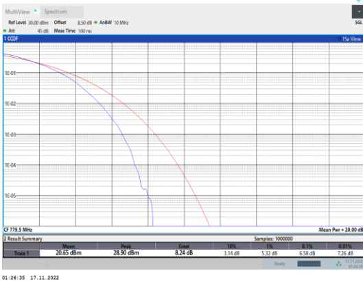
Band13-5MHz-64QAM-23205-25RB#0
