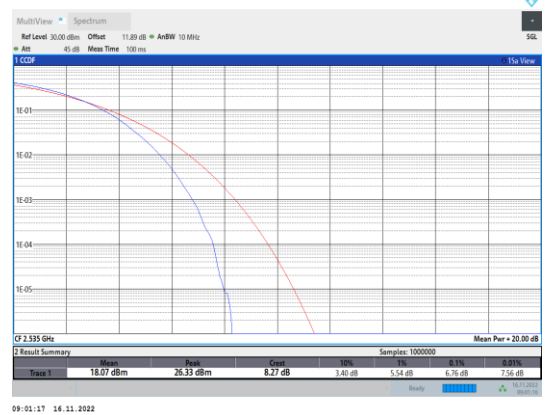
Band7-20MHz-64QAM-21100-100RB#0
