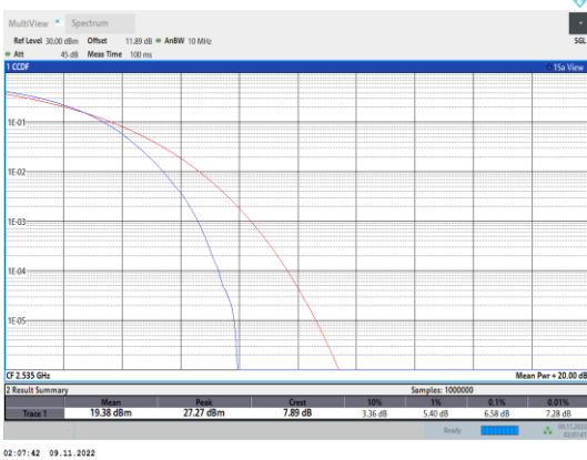
Band7-20MHz-16QAM-21100-100RB#0
