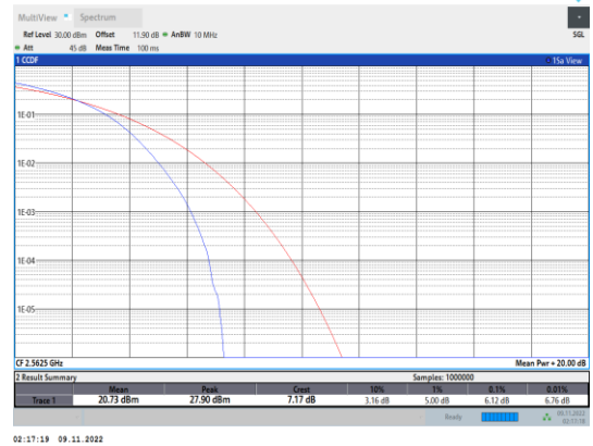
Band7-15MHz-16QAM-21375-75RB#0
