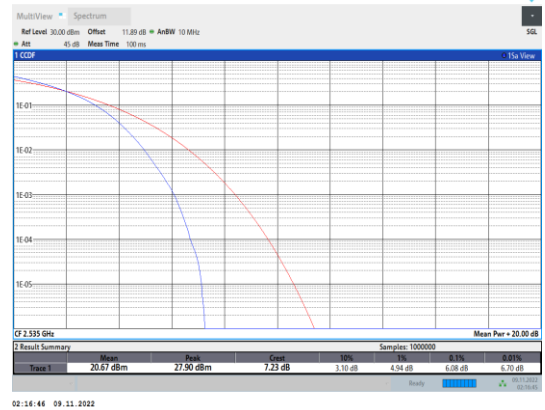
Band7-15MHz-16QAM-21100-75RB#0
