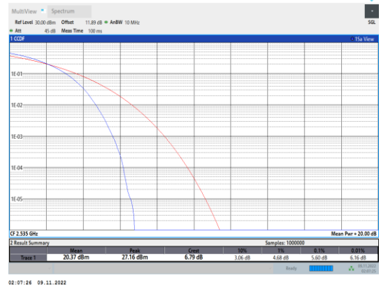
Band7-20MHz-QPSK-21100-100RB#0
