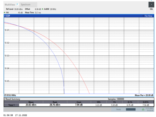
Band26-3MHz-64QAM-26740-15RB#0
