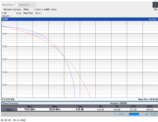
Band38-15MHz-16QAM-38175-75RB#0
