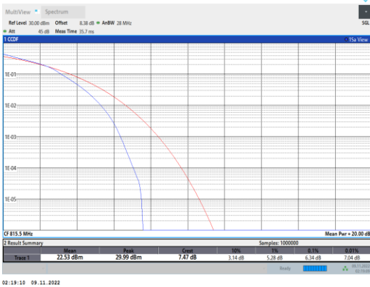
Band26-3MHz-16QAM-26705-15RB#0
