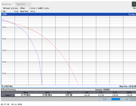
Band7-15MHz-QPSK-21375-75RB#0
