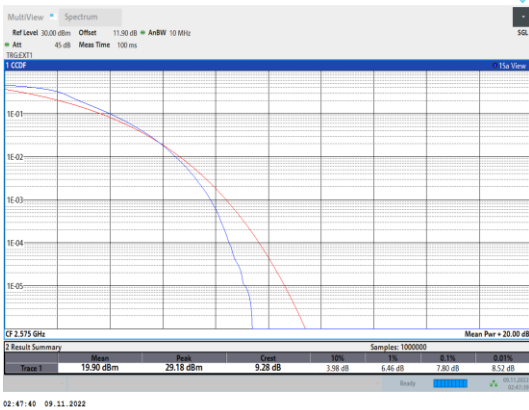
Band38-10MHz-QPSK-37800-50RB#0
