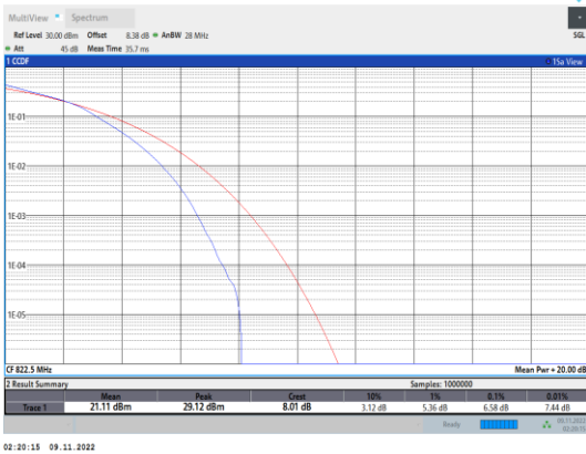
Band26-3MHz-16QAM-26775-15RB#0
