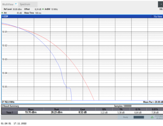
Band13-5MHz-64QAM-23230-25RB#0
