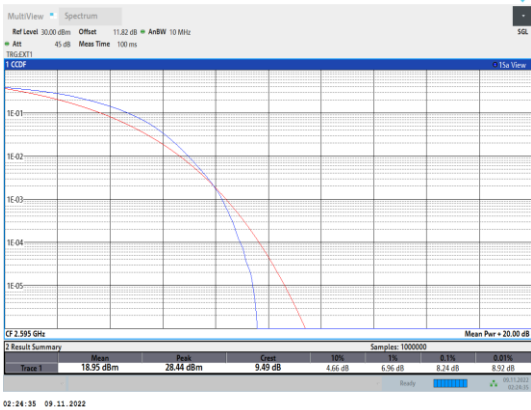
Band38-15MHz-16QAM-38000-75RB#0
