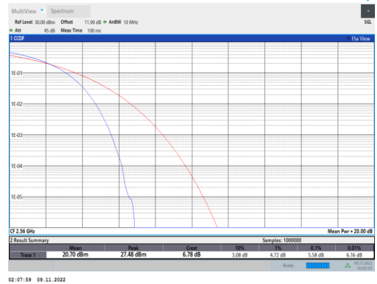
Band7-20MHz-QPSK-21350-100RB#0
