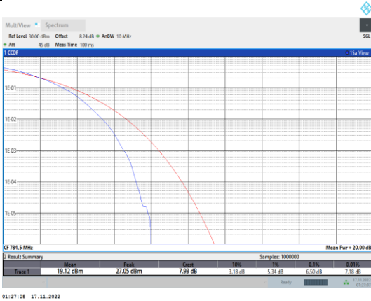
Band13-5MHz-64QAM-23255-25RB#0
