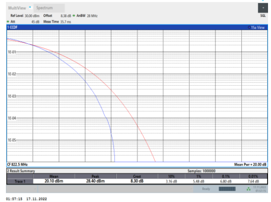
Band26-3MHz-64QAM-26775-15RB#0
