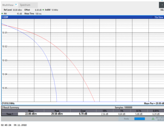
Band26-5MHz-QPSK-26740-25RB#0
