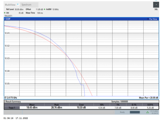
Band38-5MHz-64QAM-38225-25RB#0
