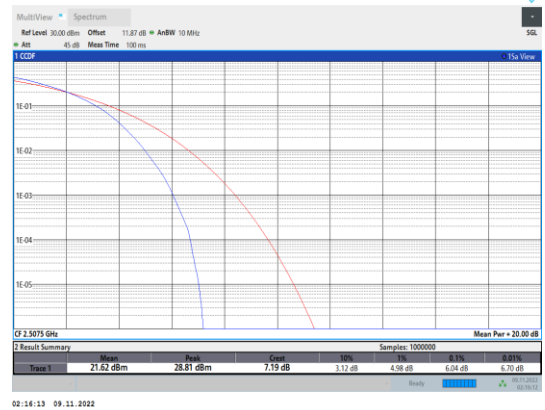
Band7-15MHz-16QAM-20825-75RB#0
