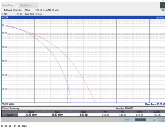
Band26-15MHz-64QAM-26765-75RB#0
