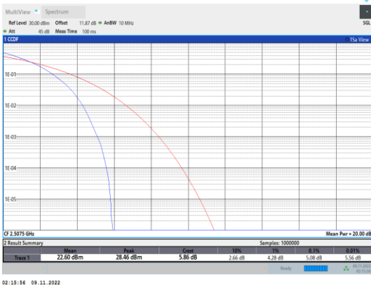
Band7-15MHz-QPSK-20825-75RB#0
