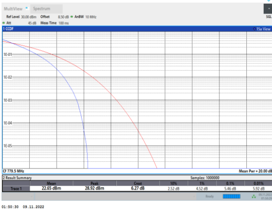
Band13-5MHz-QPSK-23205-25RB#0
