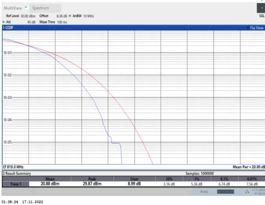
Band26-5MHz-64QAM-26740-25RB#0
