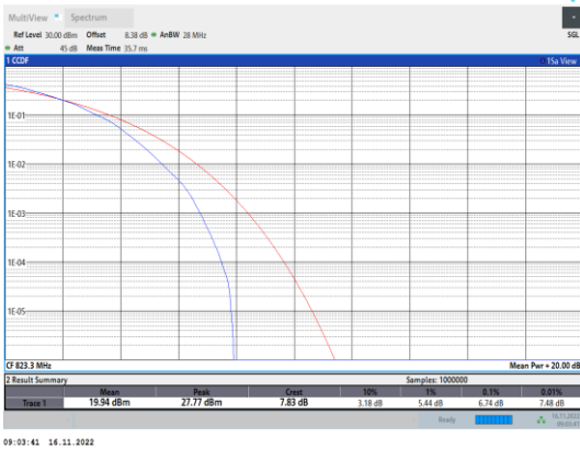
Band26-1.4MHz-64QAM-26783-6RB#0
