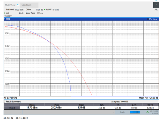
Band38-5MHz-QPSK-37775-25RB#0
