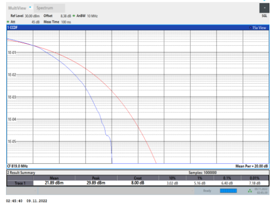
Band26-5MHz-16QAM-26740-25RB#0
