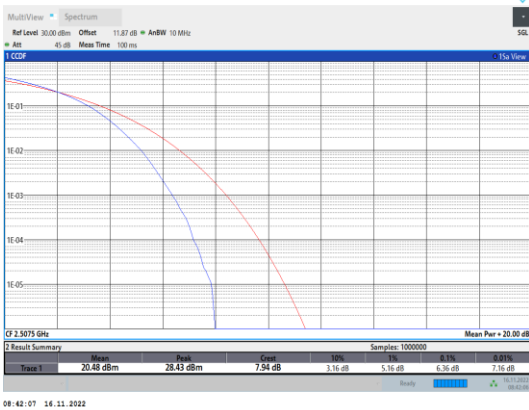
Band7-15MHz-64QAM-20825-75RB#0
