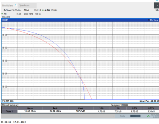
Band38-20MHz-64QAM-38000-100RB#0
