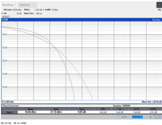
Band38-20MHz-QPSK-38000-100RB#0
