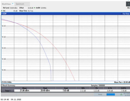
Band26-3MHz-16QAM-26740-15RB#0
