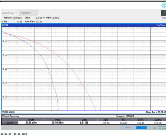
Band26-15MHz-QPSK-26915-75RB#0
