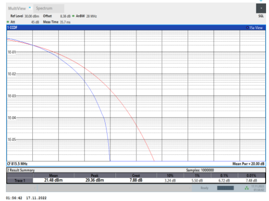
Band26-3MHz-64QAM-26705-15RB#0
