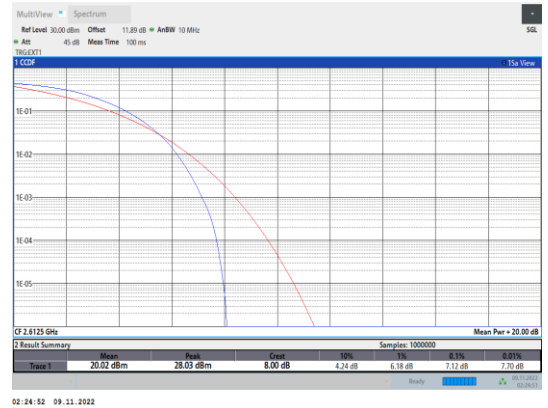
Band38-15MHz-QPSK-38175-75RB#0
