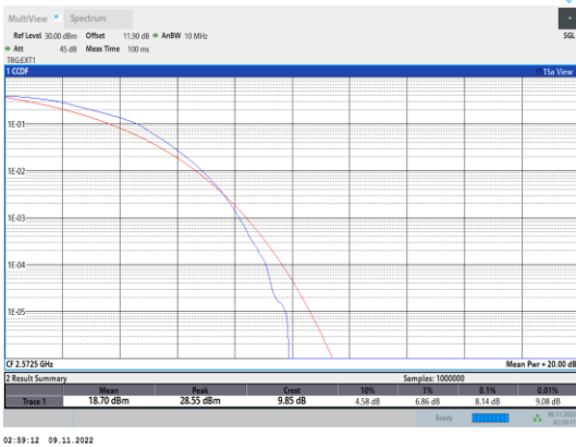
Band38-5MHz-16QAM-37775-25RB#0
