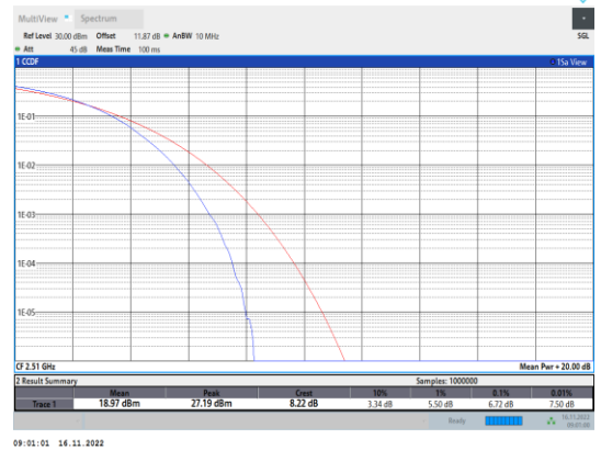
Band7-20MHz-64QAM-20850-100RB#0
