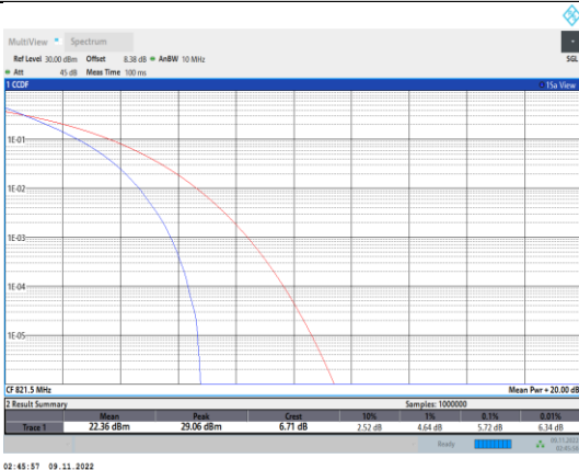
Band26-5MHz-QPSK-26765-25RB#0
