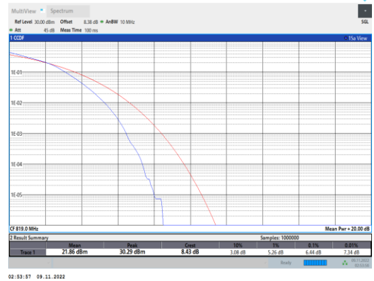
Band26-10MHz-16QAM-26740-50RB#0
