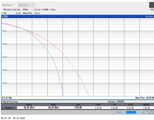
Band7-20MHz-16QAM-20850-100RB#0
