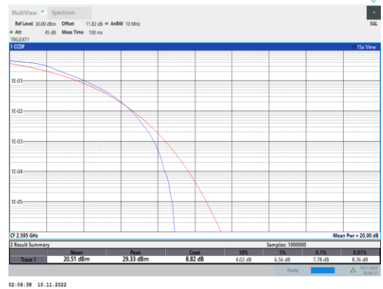
Band41-5MHz-QPSK-40640-25RB#0
