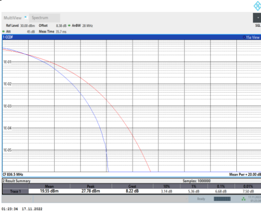
Band26-15MHz-64QAM-26915-75RB#0
