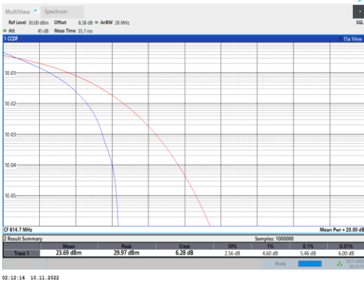
Band26-1.4MHz-QPSK-26697-6RB#0
