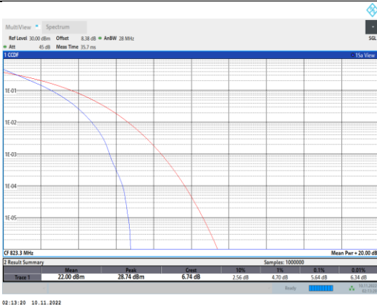
Band26-1.4MHz-QPSK-26783-6RB#0
