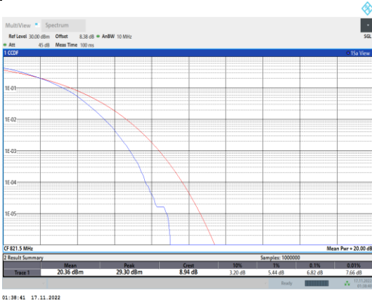
Band26-5MHz-64QAM-26765-25RB#0
