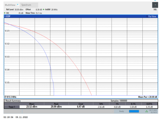
Band26-3MHz-QPSK-26705-15RB#0
