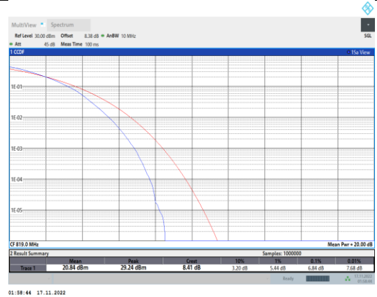
Band26-10MHz-64QAM-26740-50RB#0
