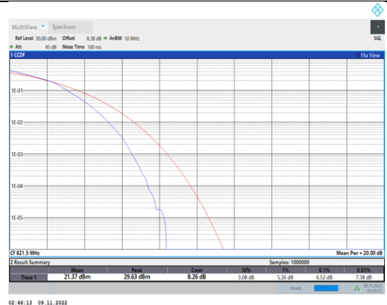
Band26-5MHz-16QAM-26765-25RB#0
