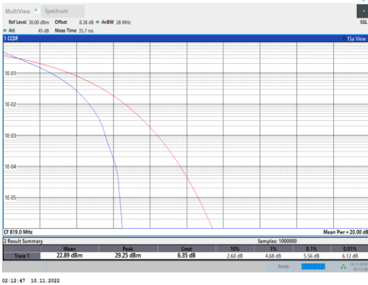
Band26-1.4MHz-QPSK-26740-6RB#0
