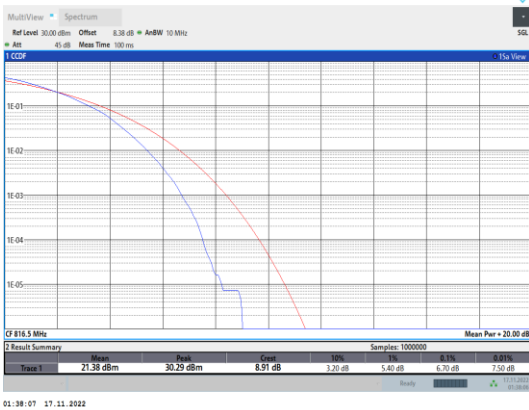
Band26-5MHz-64QAM-26715-25RB#0
