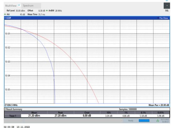
Band26-15MHz-16QAM-26915-1RB#0
