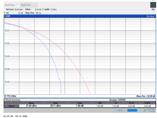
Band13-5MHz-16QAM-23205-25RB#0
