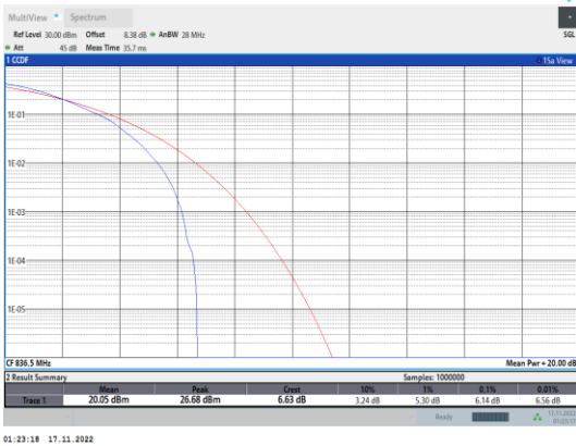
Band26-15MHz-64QAM-26915-1RB#0
