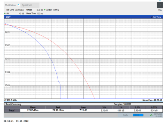
Band26-10MHz-QPSK-26740-50RB#0
