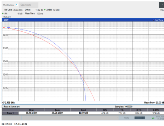
Band38-10MHz-64QAM-38000-50RB#0
