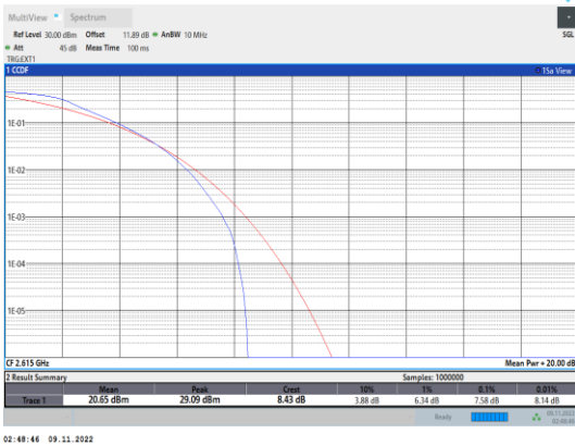
Band38-10MHz-QPSK-38200-50RB#0
