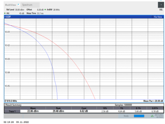
Band26-3MHz-QPSK-26740-15RB#0
