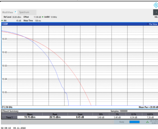
Band7-20MHz-16QAM-21350-100RB#0
