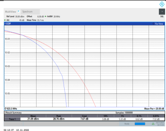
Band26-1.4MHz-16QAM-26783-6RB#0
