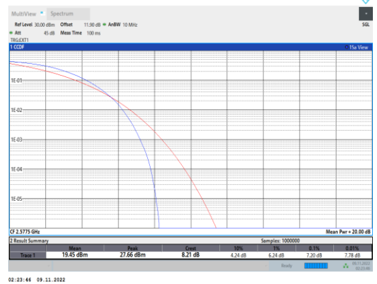
Band38-15MHz-QPSK-37825-75RB#0
