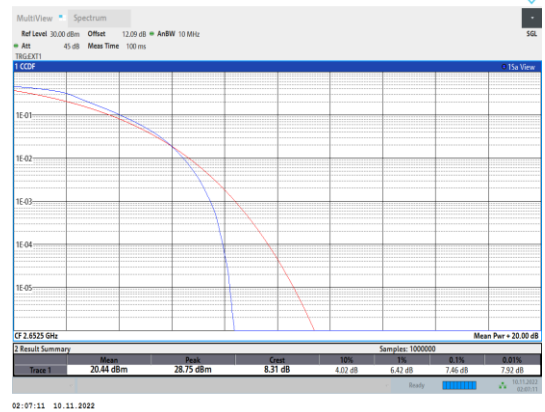
Band41-5MHz-QPSK-41215-25RB#0
