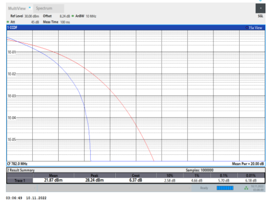
Band13-10MHz-QPSK-23230-50RB#0
