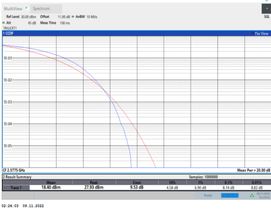
Band38-15MHz-16QAM-37825-75RB#0
