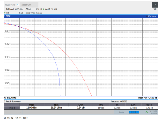
Band26-1.4MHz-16QAM-26740-6RB#0
