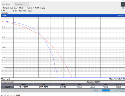
Band38-20MHz-QPSK-38150-100RB#0
