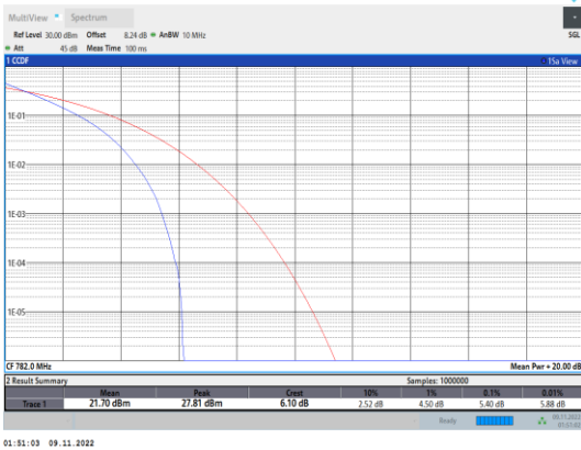
Band13-5MHz-QPSK-23230-25RB#0
