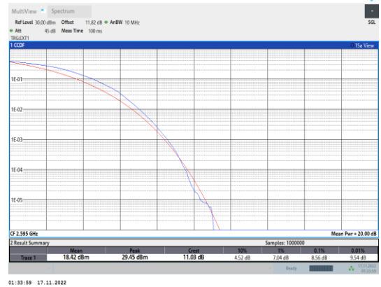
Band38-5MHz-64QAM-38000-25RB#0
