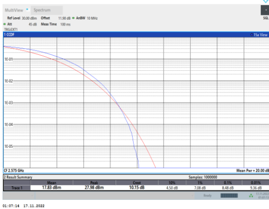
Band38-10MHz-64QAM-37800-50RB#0
