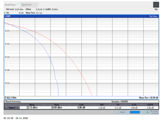
Band26-3MHz-QPSK-26775-15RB#0
