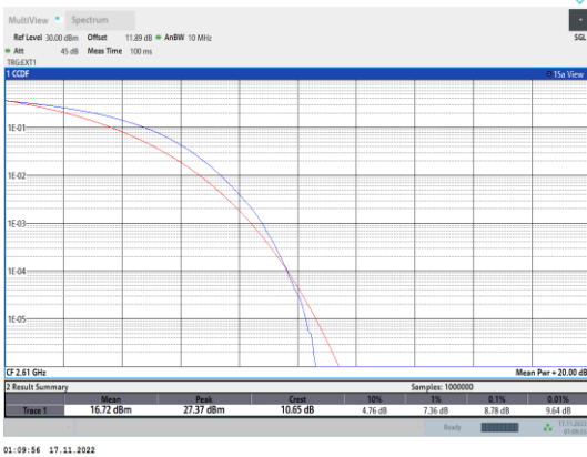
Band38-20MHz-64QAM-38150-100RB#0
