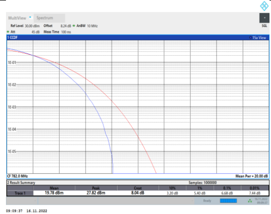
Band13-10MHz-64QAM-23230-50RB#0
