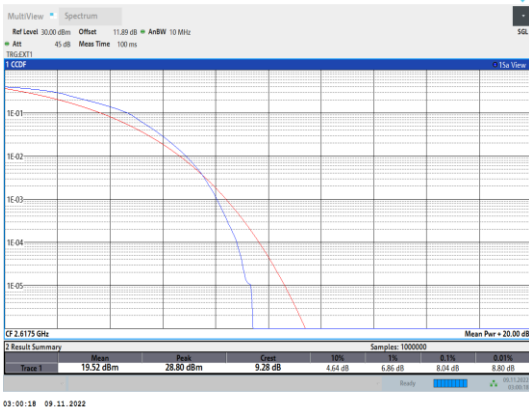
Band38-5MHz-16QAM-38225-25RB#0
