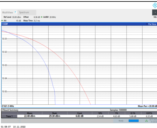
Band26-15MHz-QPSK-26765-75RB#0
