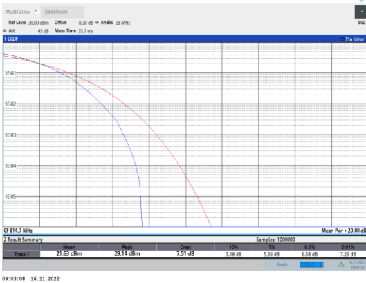
Band26-1.4MHz-64QAM-26697-6RB#0
