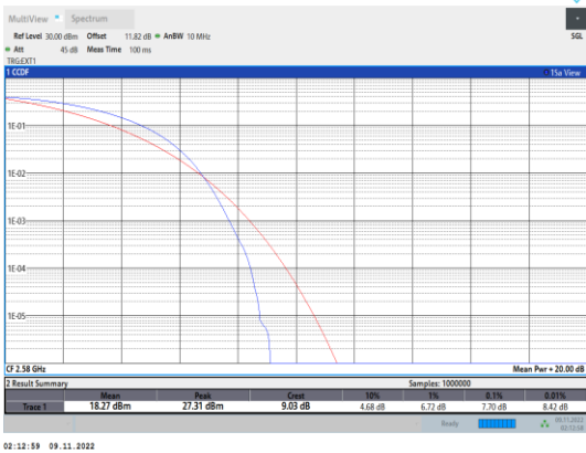
Band38-20MHz-QPSK-37850-100RB#0
