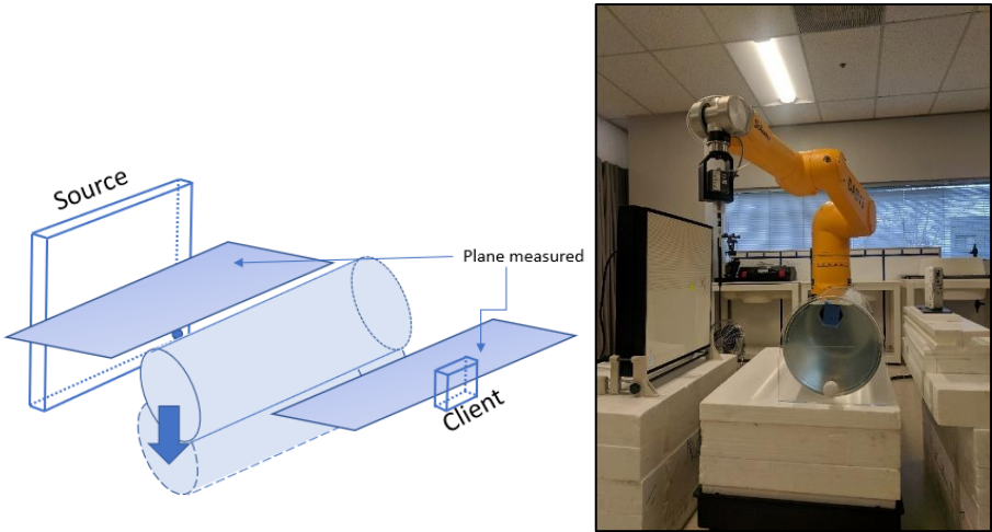
Figure 62 - Test setup - single phantom, transverse orientation (50 cm)
