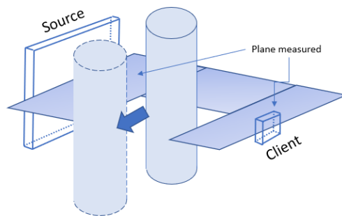
Figure 54 – Test setup – single phantom, vertical orientation (75 cm)
