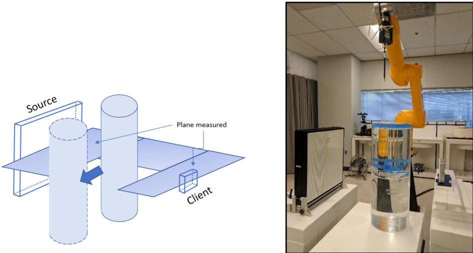
Figure 60 – Test setup – Single phantom, vertical orientation (50 cm)
