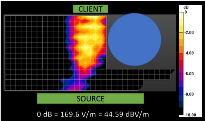
Figure 61. Obstructed E-field scan at 50 cm between Source and Client with 22.5 cm offset– Vertical Phantom
