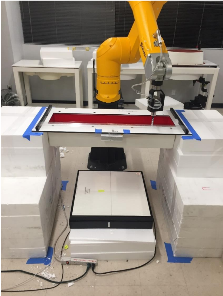
Figure 91 - SAR measurement test setup
