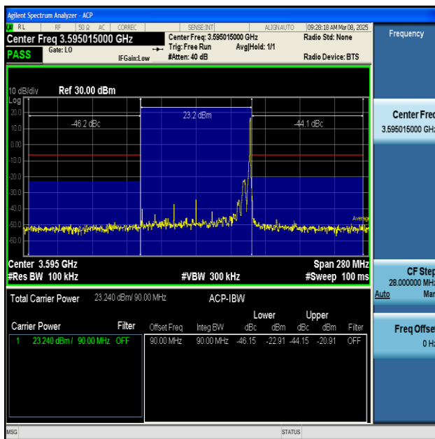
NTNV-n48-PC3-30-90-L-DFT-BPSK-Inner_1RB_Right- PASS
