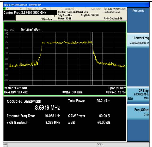
NTVN-n48-PC3-30-10-M-DFT-256QAM-Outer_Full-Ant1-PASS
