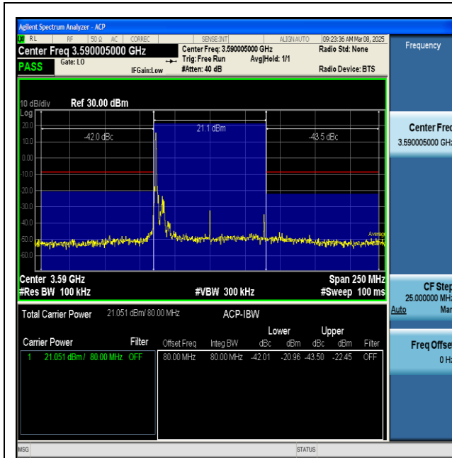
NTVN-n48-PC3-30-80-L-CP-QPSK-Inner_1RB_Left-PASS
