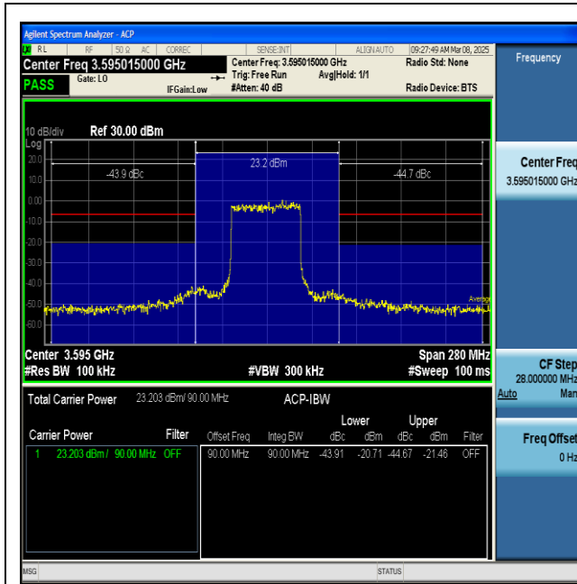
NTNV-n48-PC3-30-90-L-DFT-BPSK-Inner_Full-PASS
