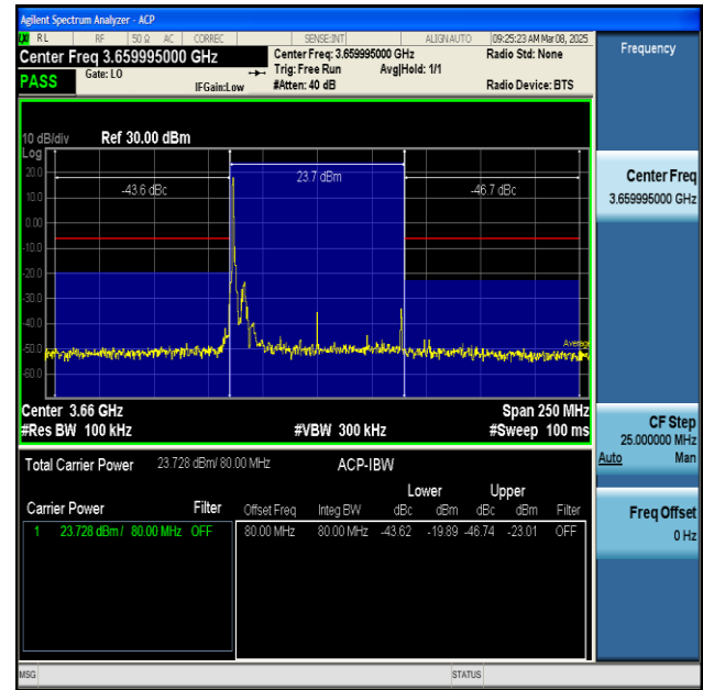
NTNV-n48-PC3-30-80-H-DFT-BPSK-Inner_1RB_Left- PASS
