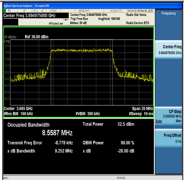
NTNV-n48-PC3-30-10-H-DFT-QPSK-Outer_Full-Ant1- PASS
