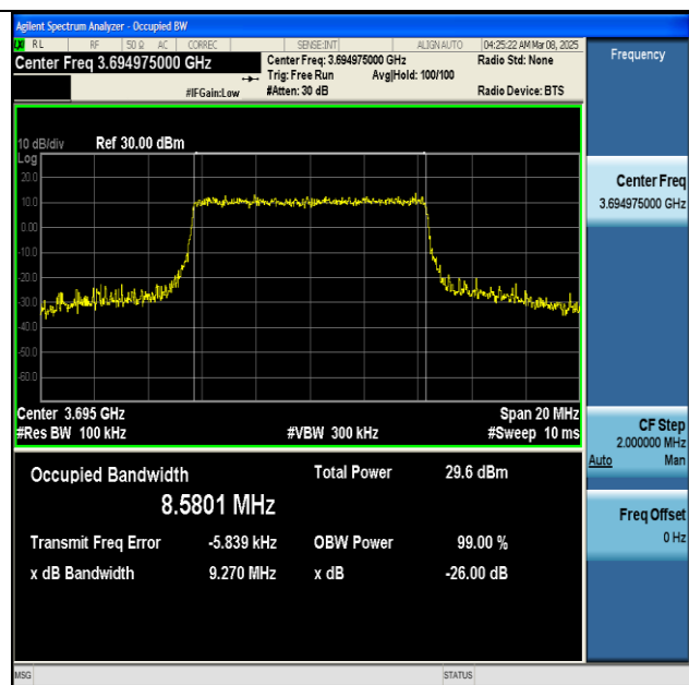
NTNV-n48-PC3-30-10-H-CP-64QAM-Outer_Full-Ant1- PASS
