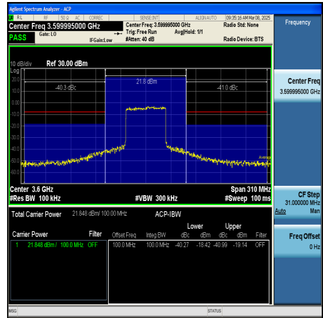
NTNV-n48-PC3-30-100-L-CP-QPSK-Inner_Full-PASS
