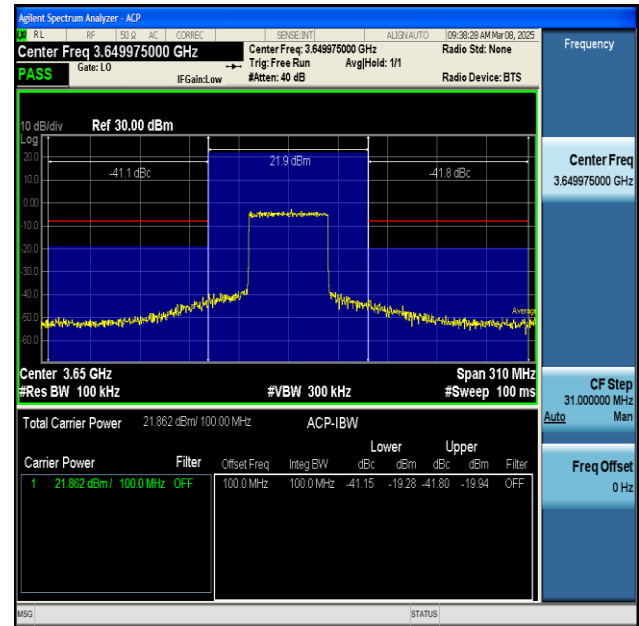
NTNV-n48-PC3-30-100-H-CP-QPSK-Inner_Full-PASS
