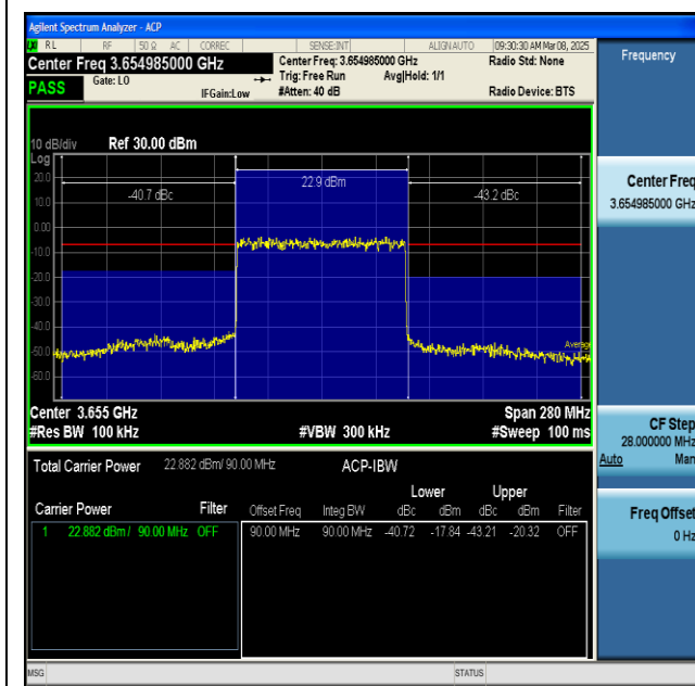
NTNV-n48-PC3-30-90-H-DFT-BPSK-Outter_Full-PASS
