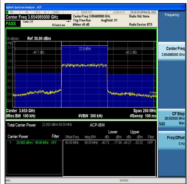
NTNV-n48-PC3-30-90-H-DFT-BPSK-Outter_Full-PASS
