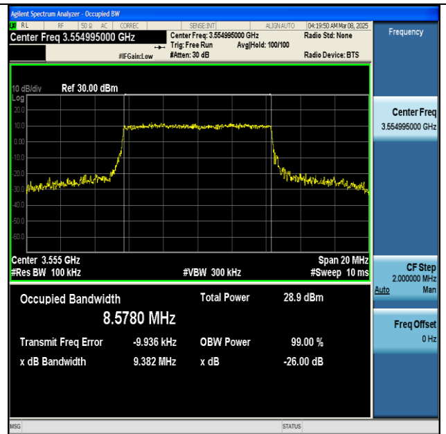
NTNV-n48-PC3-30-10-L-CP-QPSK-Outer_Full-Ant1-PASS
