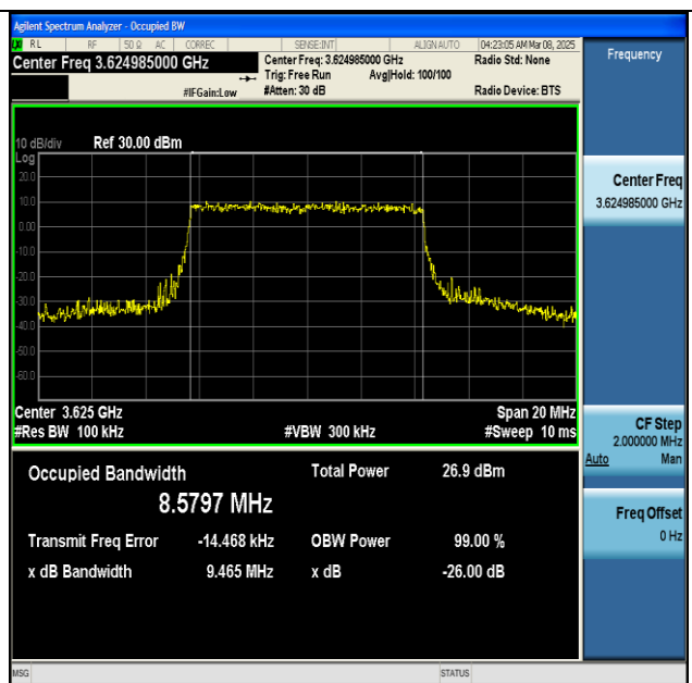
NTNV-n48-PC3-30-10-M-CP-256QAM-Outer_Full-Ant1- PASS
