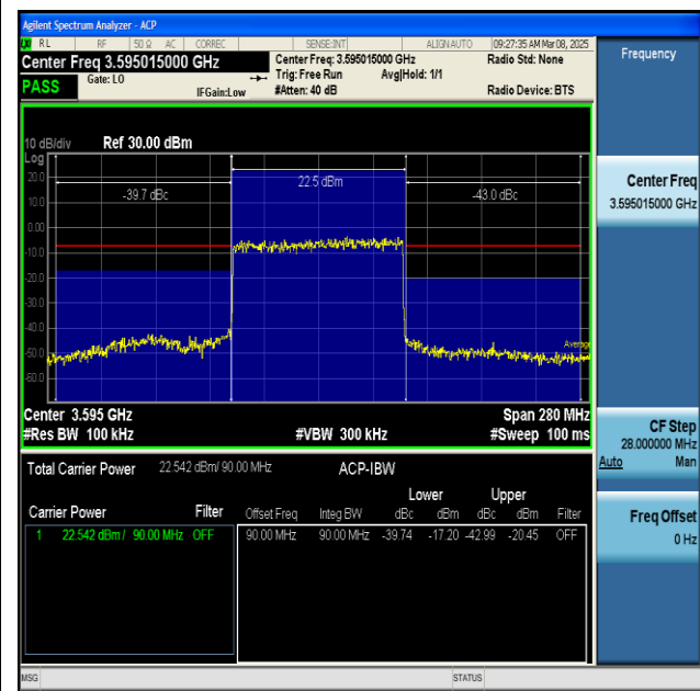
NTNV-n48-PC3-30-90-L-DFT-BPSK-Outer_Full-PASS
