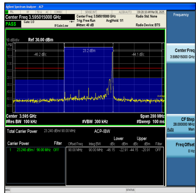
NTNV-n48-PC3-30-90-L-DFT-BPSK-Inner_1RB_Right- PASS
