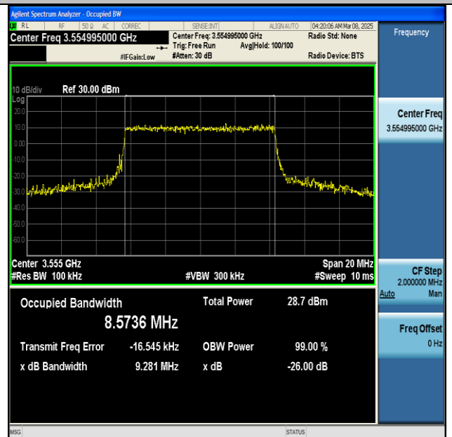
NTNV-n48-PC3-30-10-L-CP-64QAM-Outer_Full-Ant1-PASS
