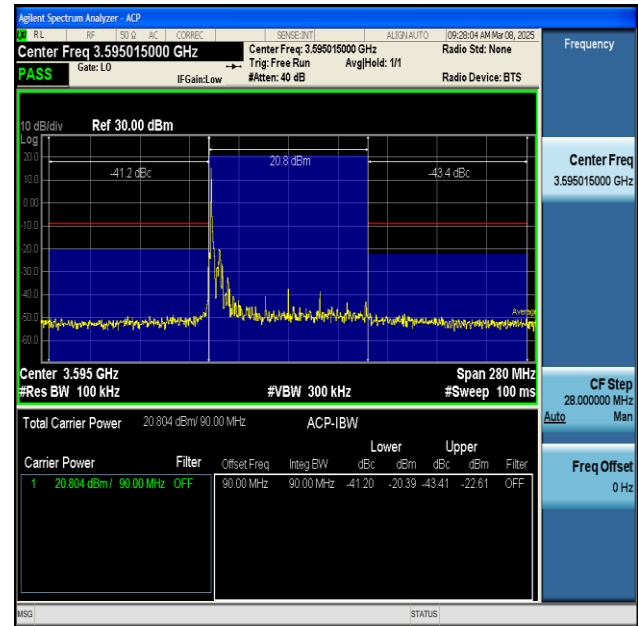
NTNV-n48-PC3-30-90-L-DFT-BPSK-Inner_1RB_Left- PASS
