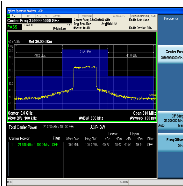
NTNV-n48-PC3-30-100-L-CP-QPSK-Inner_Full-PASS
