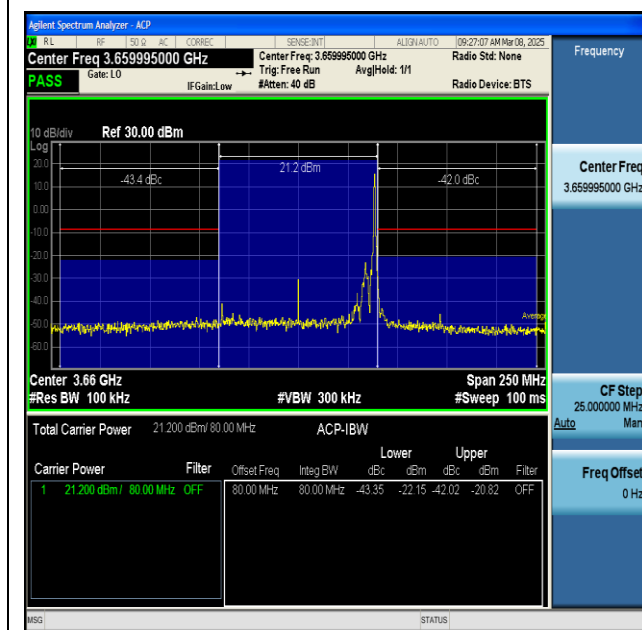
NTNV-n48-PC3-30-80-H-CP-QPSK-Inner_1RB_Right-PASS
