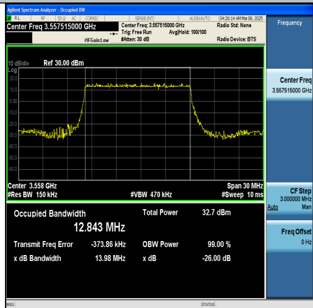
NTNV-n48-PC3-30-15-L-DFT-BPSK-Outer_Full-Ant1- PASS
