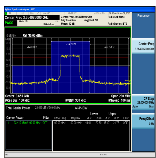
NTNV-n48-PC3-30-90-H-DFT-BPSK-Inner_Full-PASS
