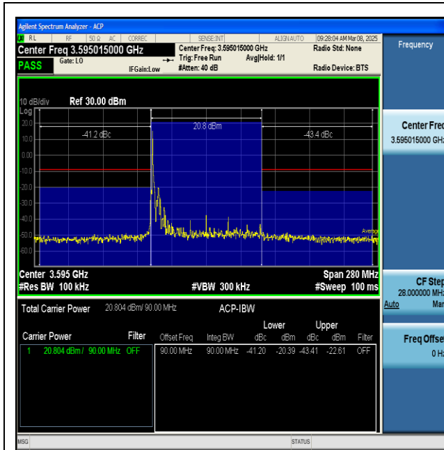
NTNV-n48-PC3-30-90-L-DFT-BPSK-Inner_1RB_Left- PASS
