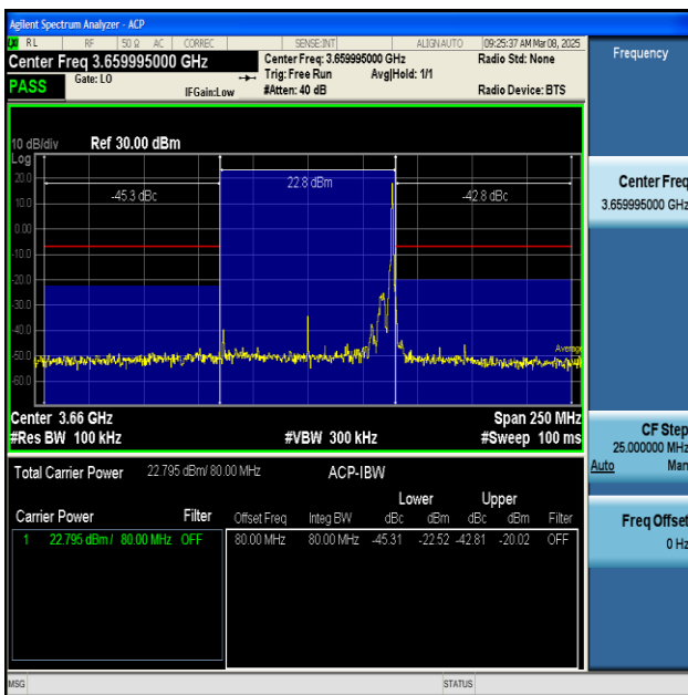
NTNV-n48-PC3-30-80-H-DFT-BPSK-Inner_1RB_Right- PASS
