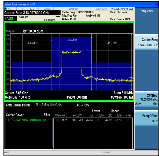
NTNV-n48-PC3-30-100-H-DFT-BPSK-Inner_Full-PASS
