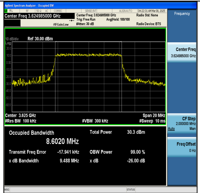
NTVN-n48-PC3-30-10-M-CP-16QAM-Outer_Full-Ant1-PASS
