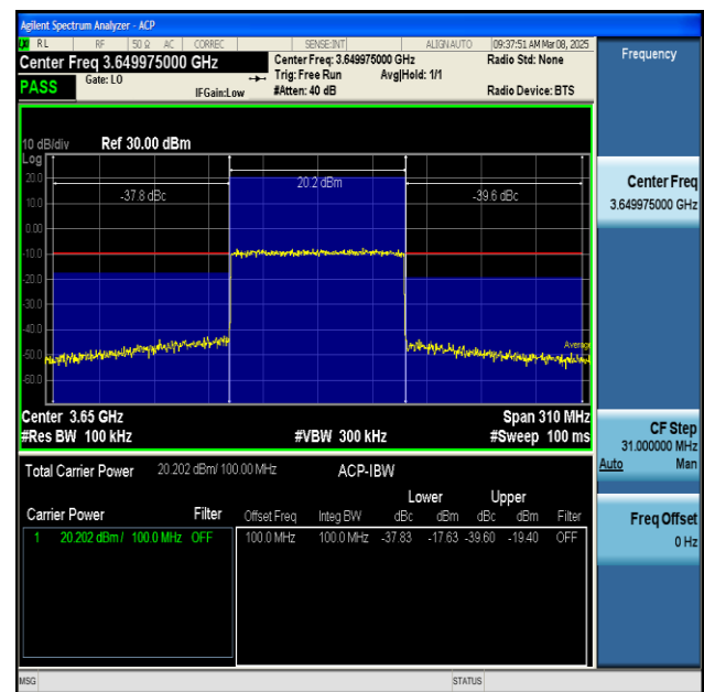
NTNV-n48-PC3-30-100-H-CP-QPSK-Outer_Full-PASS
