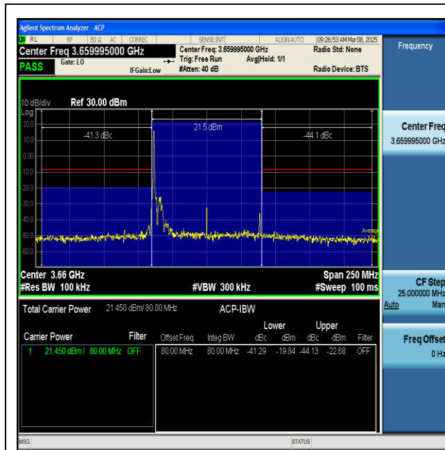
NTNV-n48-PC3-30-80-H-CP-QPSK-Inner_1RB_Left-PASS
