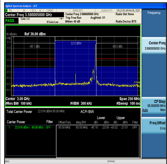
NTVN-n48-PC3-30-80-L-CP-QPSK-Inner_1RB_Right-PASS
