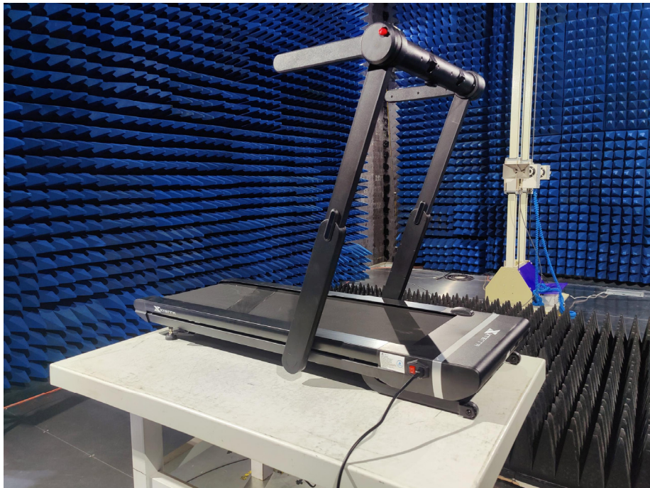
For Above 1GHz Test Site 1# Model: WS300
