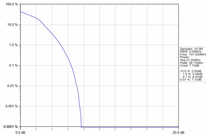
Band12_3MHz_16QAM_MCH_707.5MHz_RB_15_0_NTNV
