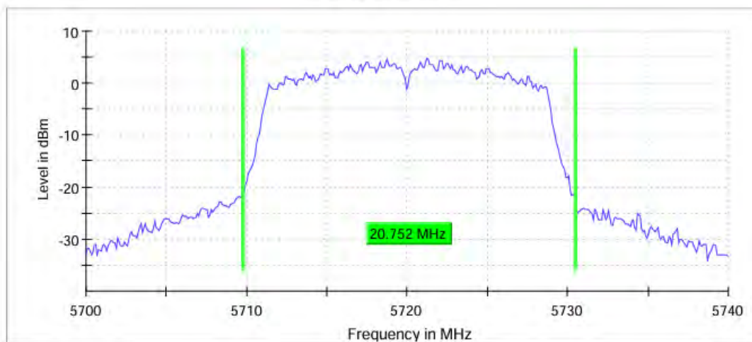
26 dB Bandwidth
