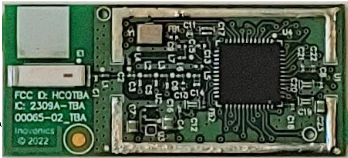
TBA Module – Topside without Can
