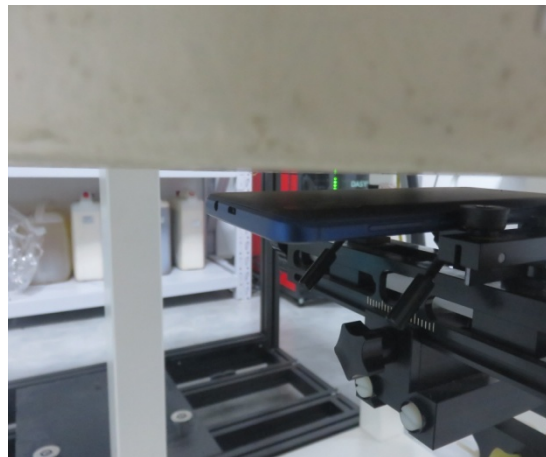
Body-worn Rear Side (10mm)
