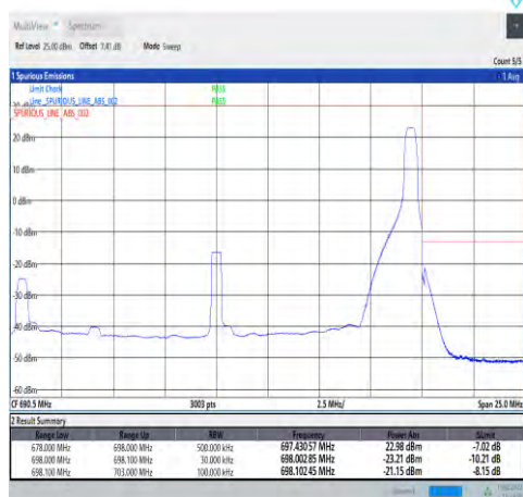
1-N71-PC3-15-20-H-2-DFT-PI2BPSK-Edge_1RB_Right-1@105-Ant1-PASS-see graph
