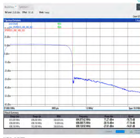
1-N71-PC3-15-5-H-6-CP-QPSK-Outer_Full-2 5@0-Ant1-PASS-see graph
