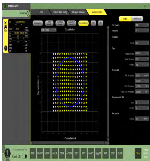
1-N71-15-20-M-5-DFT-256QAM-Outer_Full-100@0-Ant1-see graph-PASS
