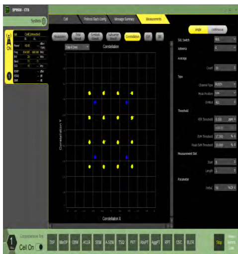
1-N71-15-20-M-7-CP-16QAM-Outer_Full-106@0-Ant1-see graph-PASS
