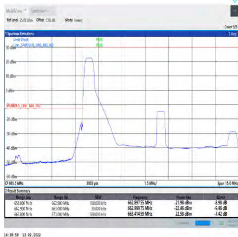
1-N71-PC3-15-10-L-1-DFT-PI2BPSK-Edge_1 RB_Left-1@0-Ant1-PASS-see graph
