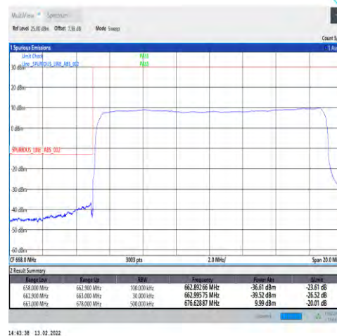
1-N71-PC3-15-15-L-3-DFT-PI2BPSK-Outer_ Full-75@0-Ant1-PASS-see graph
