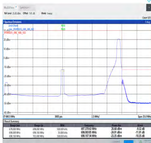
1-N71-PC3-15-20-H-5-CP-QPSK-Edge_1RB_Right-1@105-Ant1-PASS-see graph
