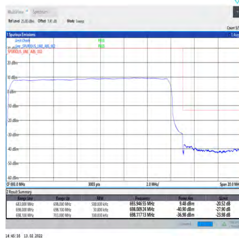
1-N71-PC3-15-15-H-3-DFT-PI2BPSK-Outer_Full-75@0-Ant1-PASS-see graph
