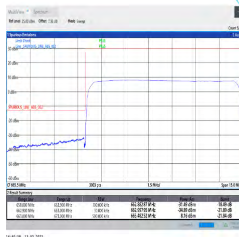
1-N71-PC3-15-10-L-6-CP-QPSK-Outer_Full- 52@0-Ant1-PASS-see graph
