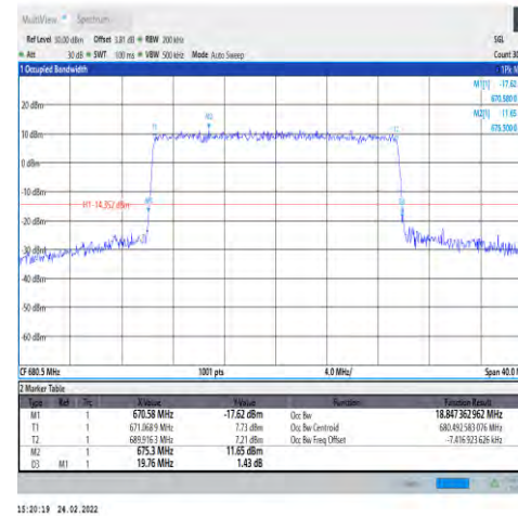
1-N71-PC3-15-20-M-8-CP-64QAM-Outer_Ful I-106@0-Ant1-18.847-19.760-≤20-PASS
