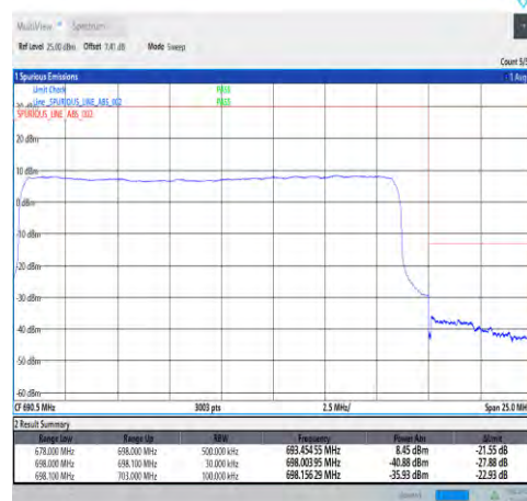
1-N71-PC3-15-20-H-3-DFT-PI2BPSK-Outer_Full-100@0-Ant1-PASS-see graph
