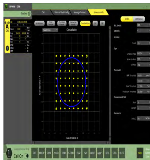
1-N71-15-20-M-4-DFT-64QAM-Outer_Full-100@0-Ant1-see graph-PASS
