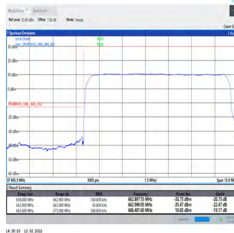
1-N71-PC3-15-10-L-3-DFT-PI2BPSK-Outer_ Full-50@0-Ant1-PASS-see graph
