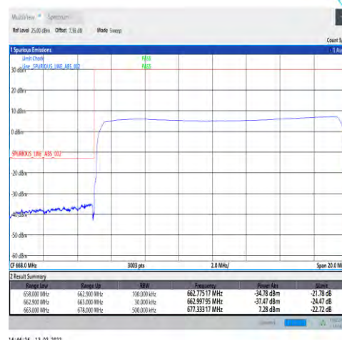
1-N71-PC3-15-15-L-6-CP-QPSK-Outer_Full- 79@0-Ant1-PASS-see graph
