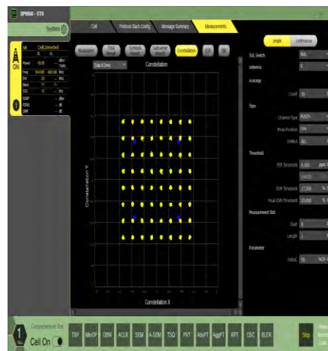
1-N71-15-20-M-8-CP-64QAM-Outer_Full-106@0-Ant1-see graph-PASS
