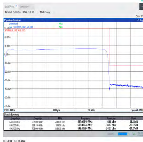
1-N71-PC3-15-15-H-6-CP-QPSK-Outer_Full-79@0-Ant1-PASS-see graph
