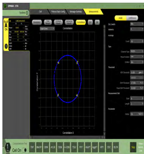
1-N71-15-20-M-1-DFT-PI2BPSK-Outer_Full-100@0-Ant1-see graph-PASS
