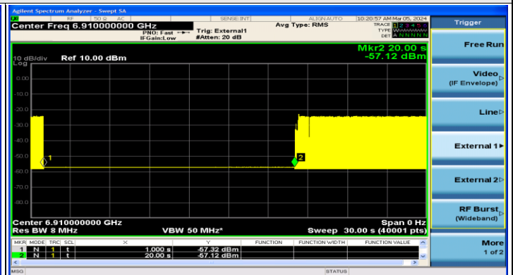
802.11ax (HE160) Full RU / CH207(Low Edge)
