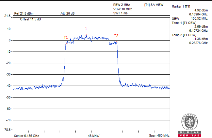
802.11ax (HE160) Full RU / Chain 0 : CH 47
