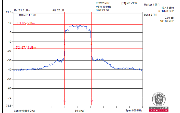
802.11ax (HE160) Full RU / Chain 1 : CH 143
