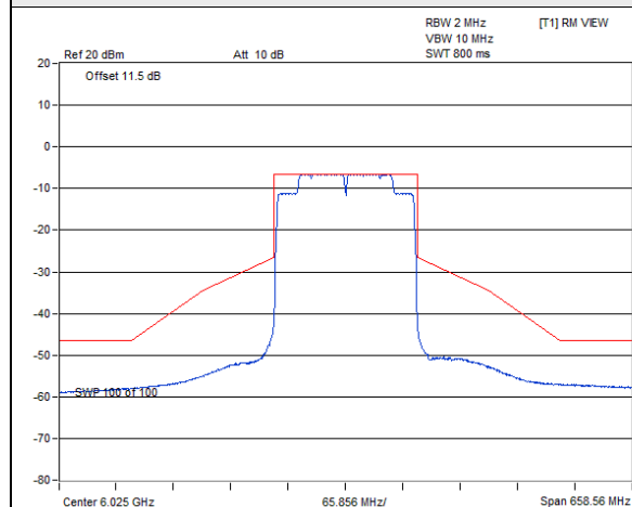
802.11ax (HE160) Full RU / Chain 0 : CH 15
