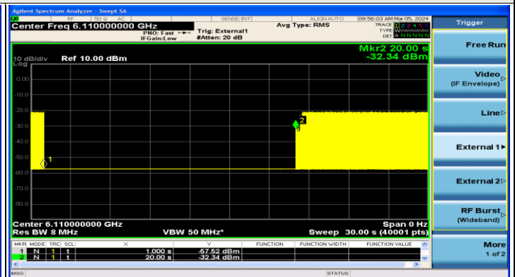
802.11ax (HE160) Full RU / CH47(Low Edge)
