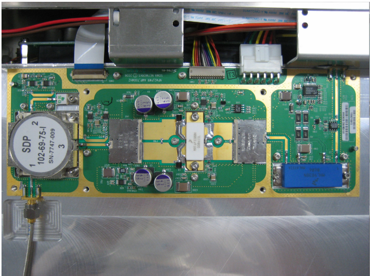
Power Amplifier(close up)
