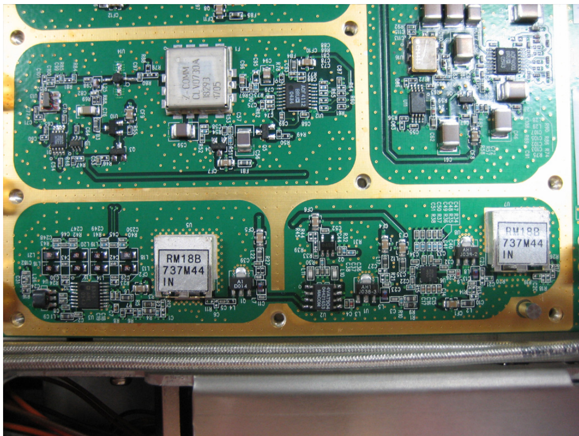
Up Down Converter(close up : Tx part)
