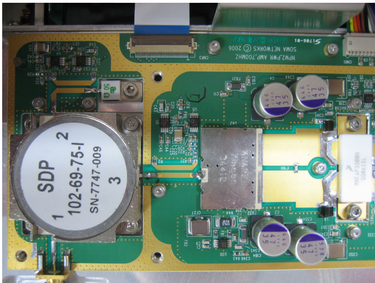
Power Amplifier(close up: Output part)
