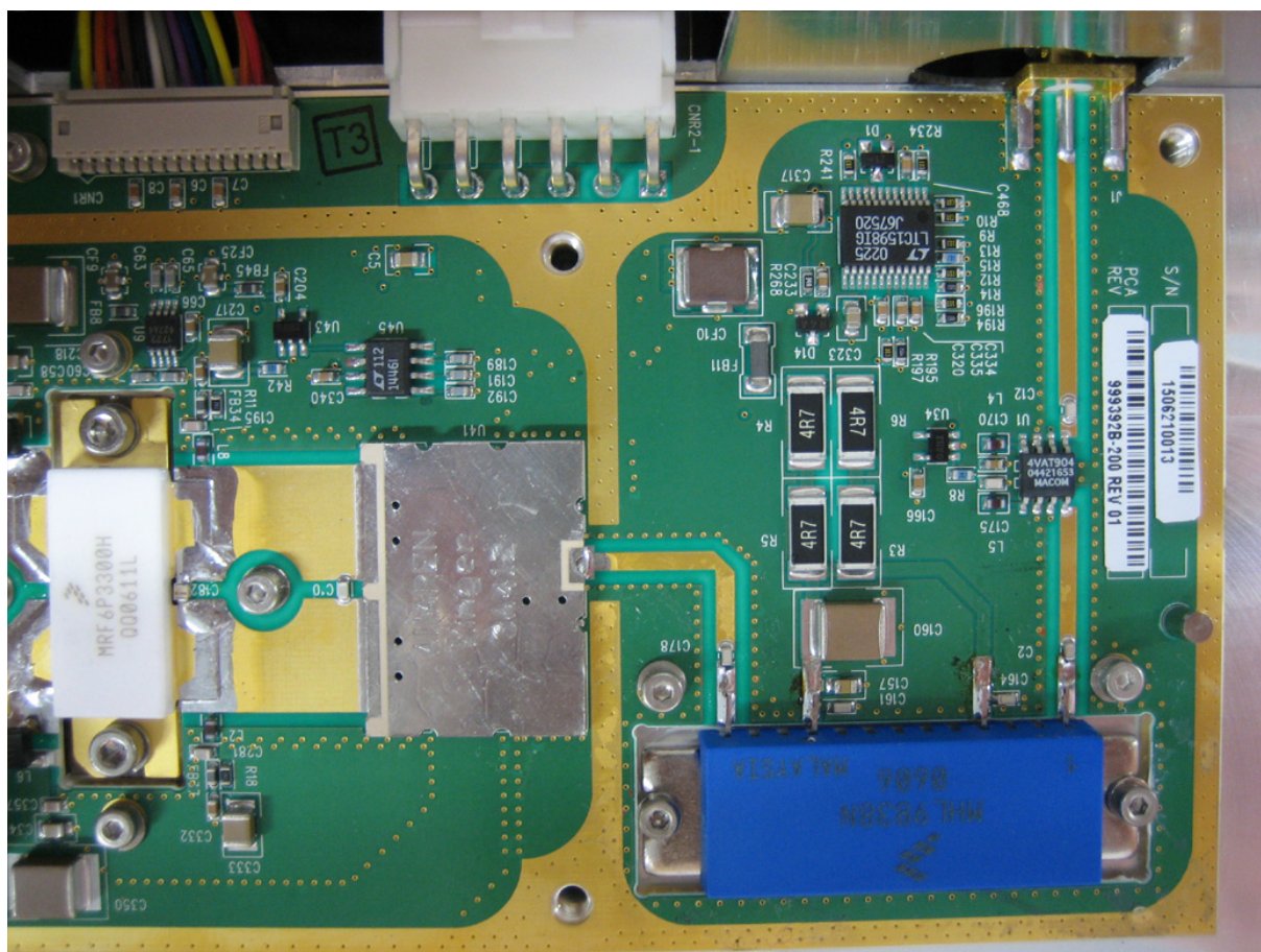
Power Amplifier(close up: Input part)
