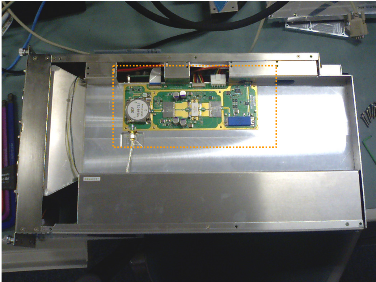
Power Amplifier(overall view)
