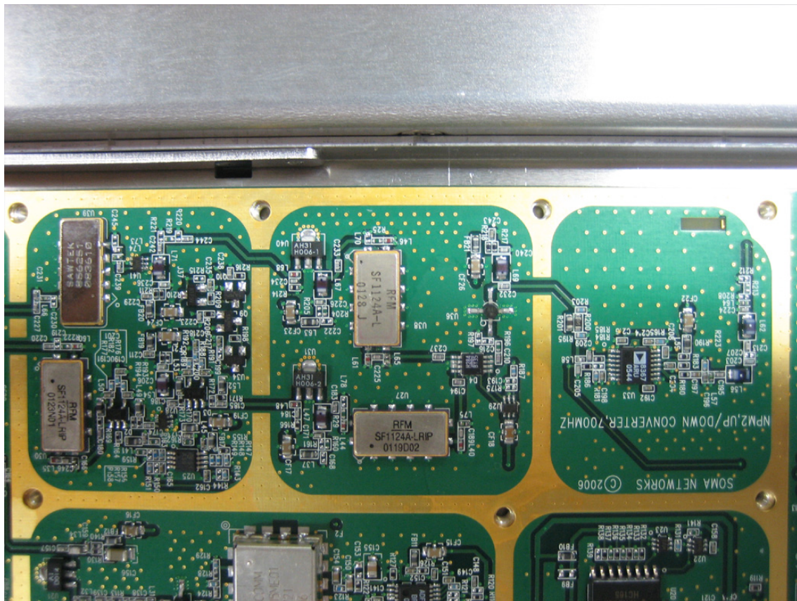
Up Down Converter(close up : Rx part)
