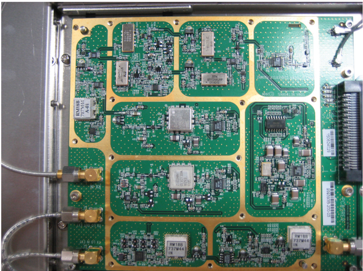
Up Down Converter (close up)
