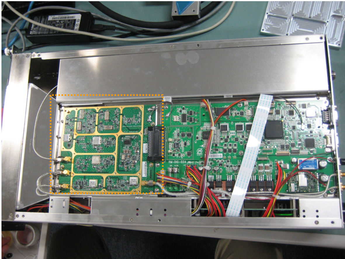
Up Down Converter with Digital Board (overall view)
