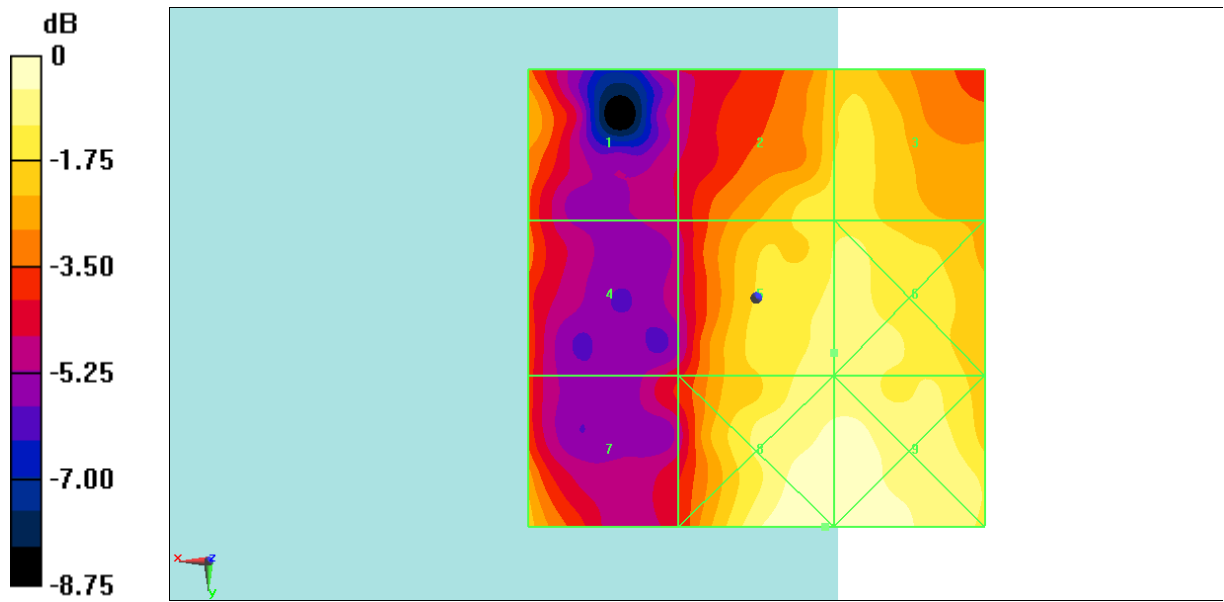
Fig B.44 HAC RF E-Field LTE Band41 Power Class 3 64QAM CH40185
