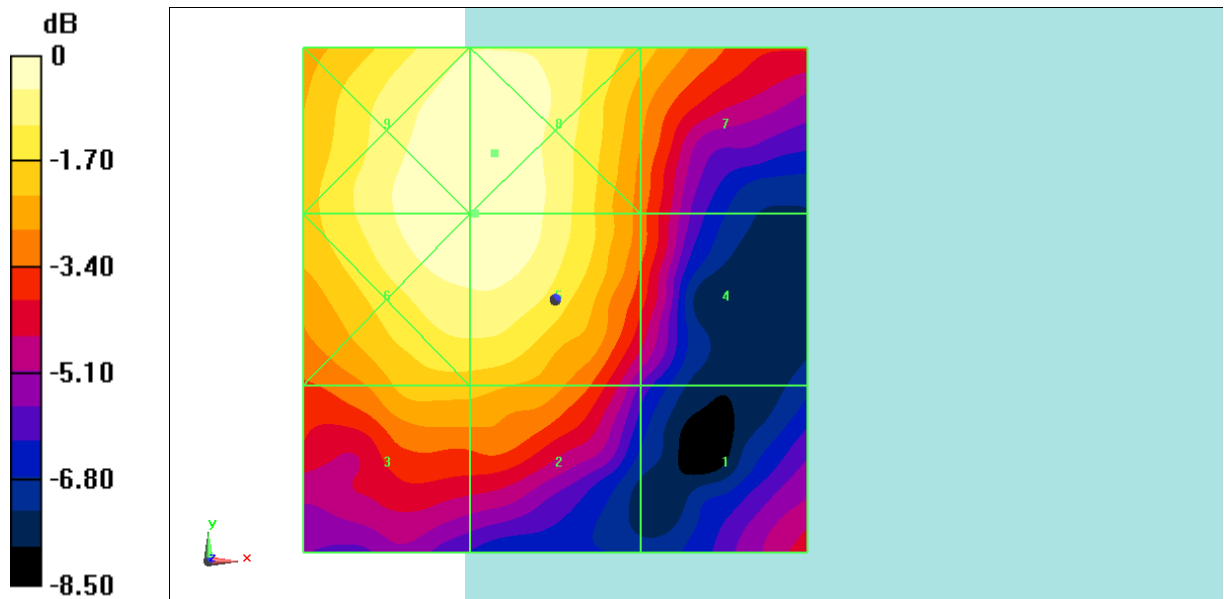
Fig B.35 HAC RF E-Field LTE Band41 Power Class 3 QPSK CH39750
