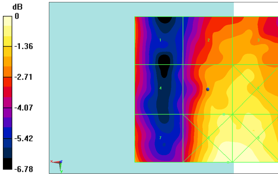
Fig B.43 HAC RF E-Field LTE Band41 Power Class 3 64QAM CH40620
