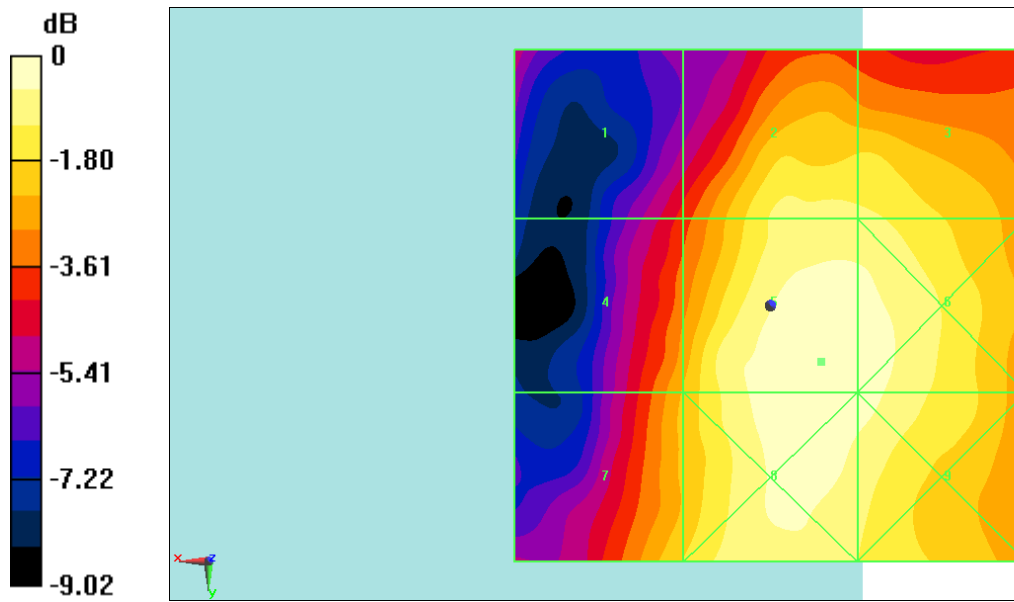
Fig B.45 HAC RF E-Field LTE Band41 Power Class 3 64QAM CH39750
