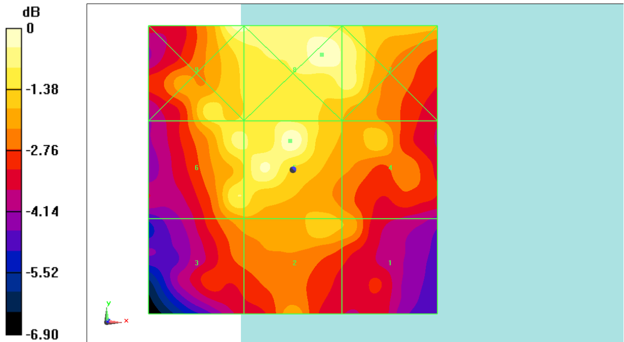
Fig B.8 HAC RF E-Field CDMA BC0 Middle
