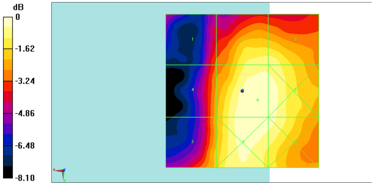
Fig B.40 HAC RF E-Field LTE Band41 Power Class 3 16QAM CH39750
