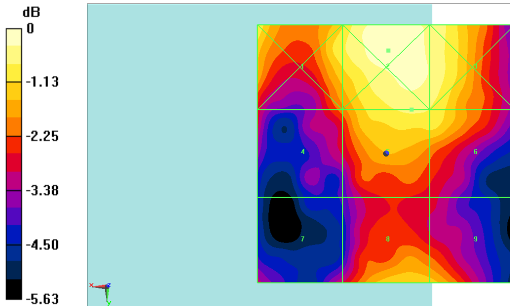
Fig B.26 HAC RF E-Field LTE Band41 Power Class 2 64QAM CH41490
