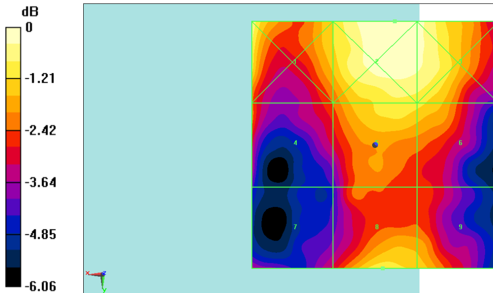
Fig B.30 HAC RF E-Field LTE Band41 Power Class 2 64QAM CH39750
