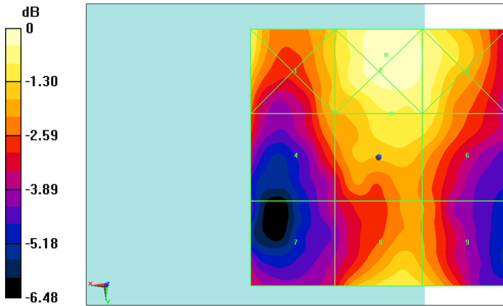
Fig B.29 HAC RF E-Field LTE Band41 Power Class 2 64QAM CH40185
