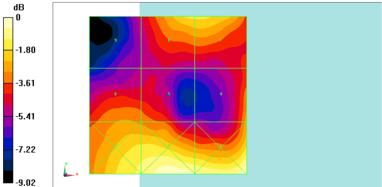
Fig B.31 HAC RF E-Field LTE Band41 Power Class 3 QPSK CH41490
