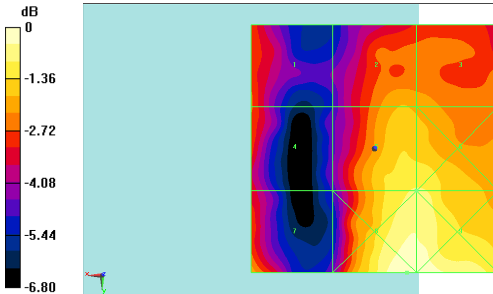
Fig B.42 HAC RF E-Field LTE Band41 Power Class 3 64QAM CH41055
