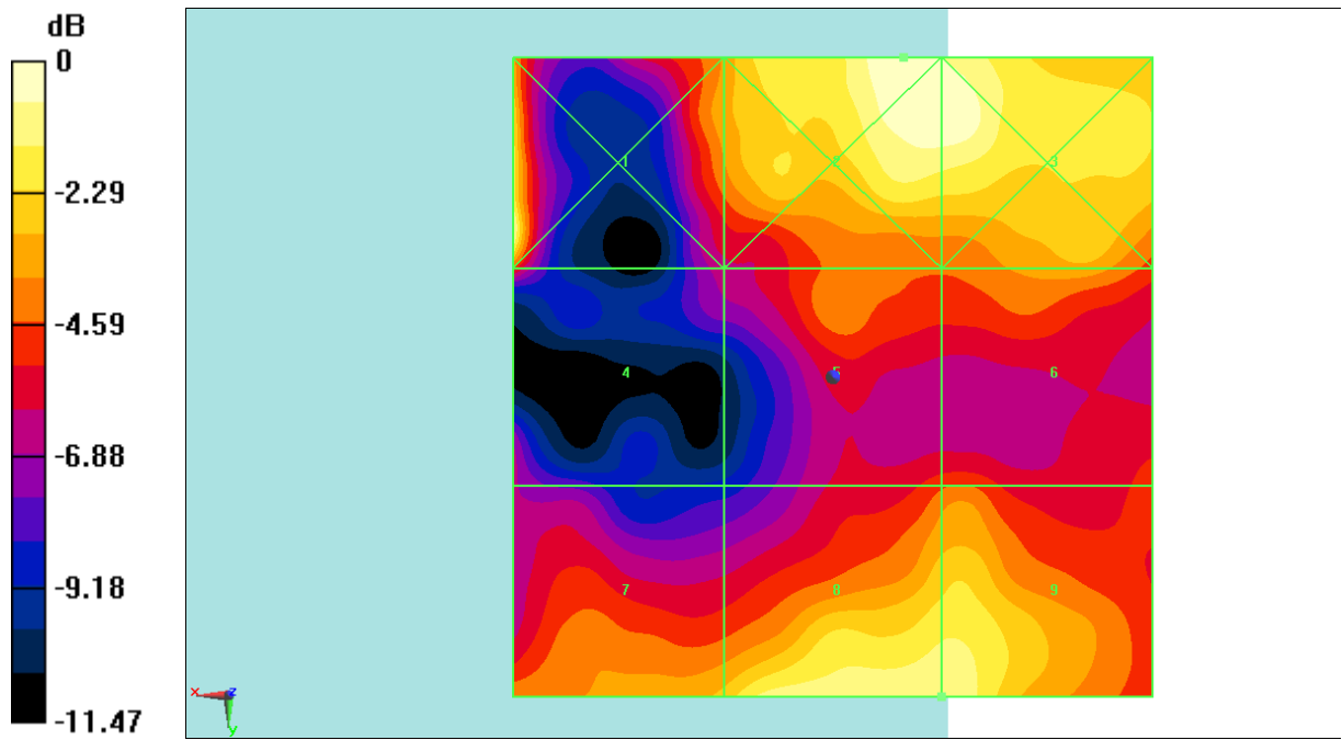
Fig B.10 HAC RF E-Field CDMA BC1 High
