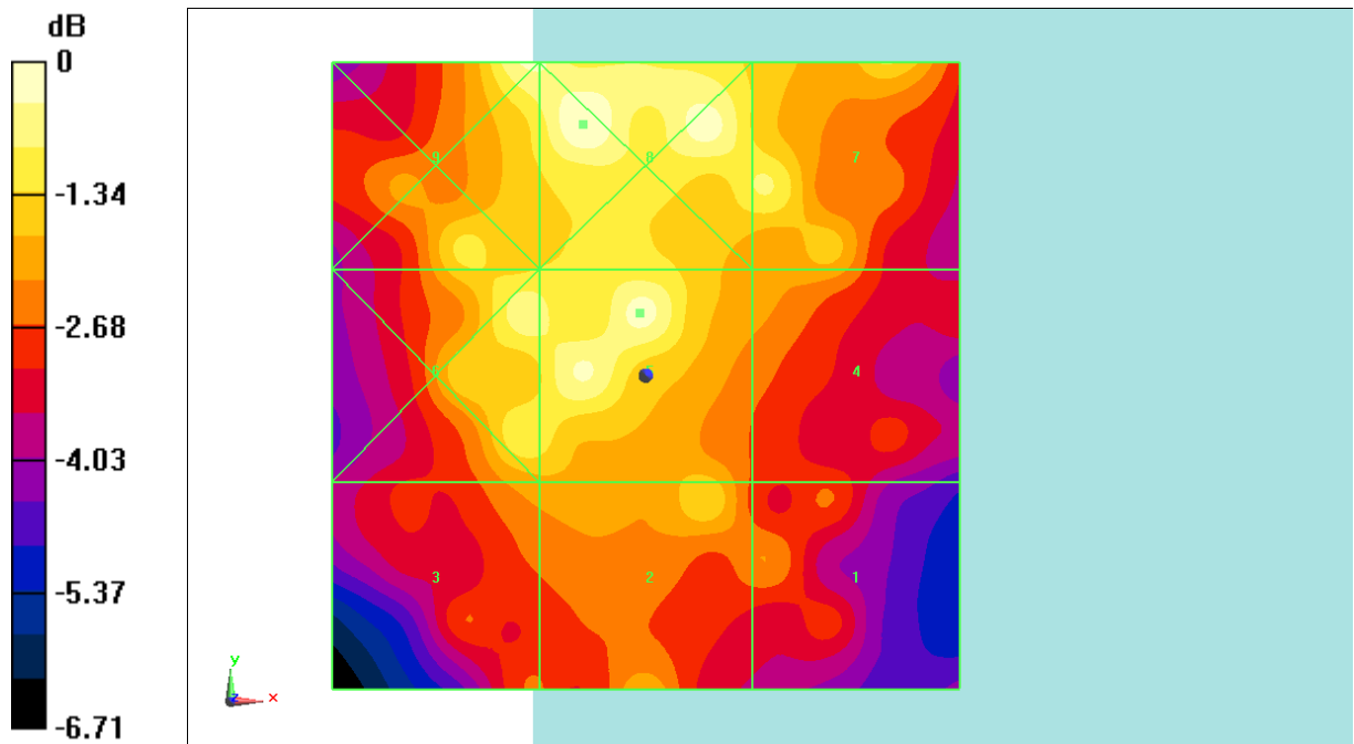
Fig B.7 HAC RF E-Field CDMA BC0 High
