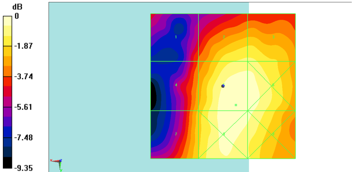
Fig B.39 HAC RF E-Field LTE Band41 Power Class 3 16QAM CH40185
