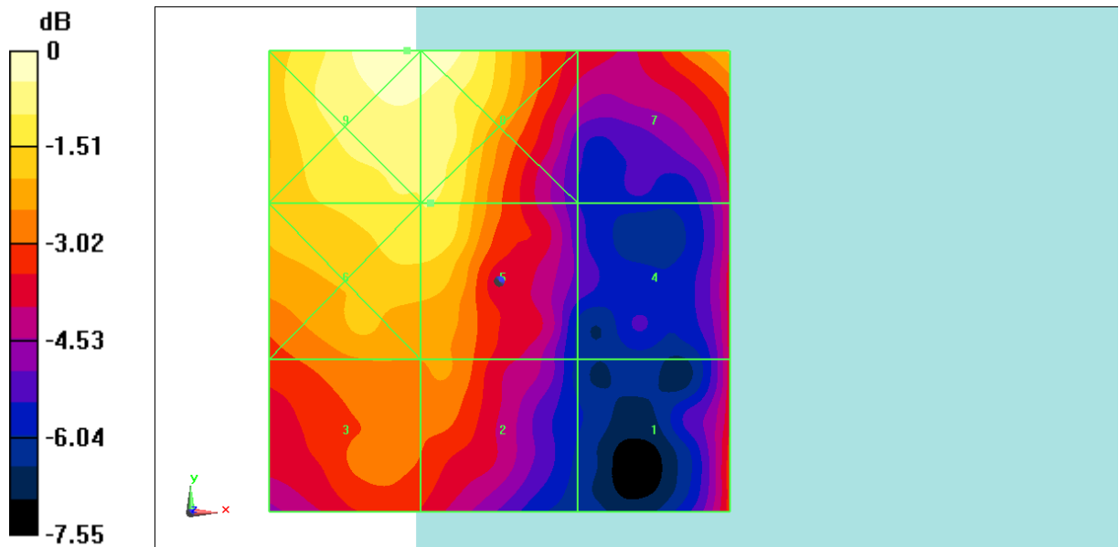
Fig B.34 HAC RF E-Field LTE Band41 Power Class 3 QPSK CH40185
