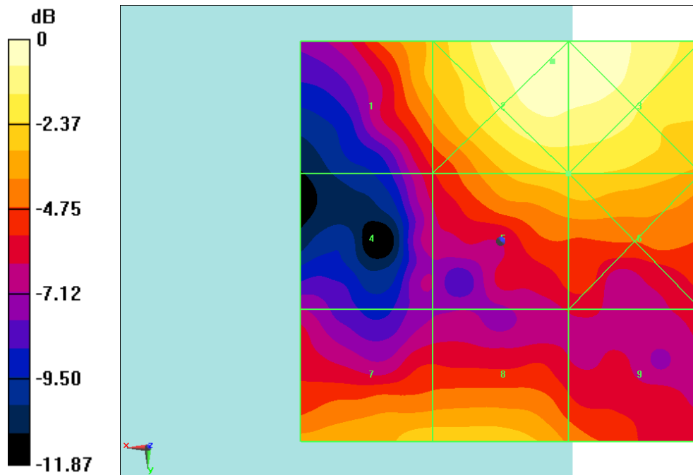
Fig B.12 HAC RF E-Field CDMA BC1 Low
