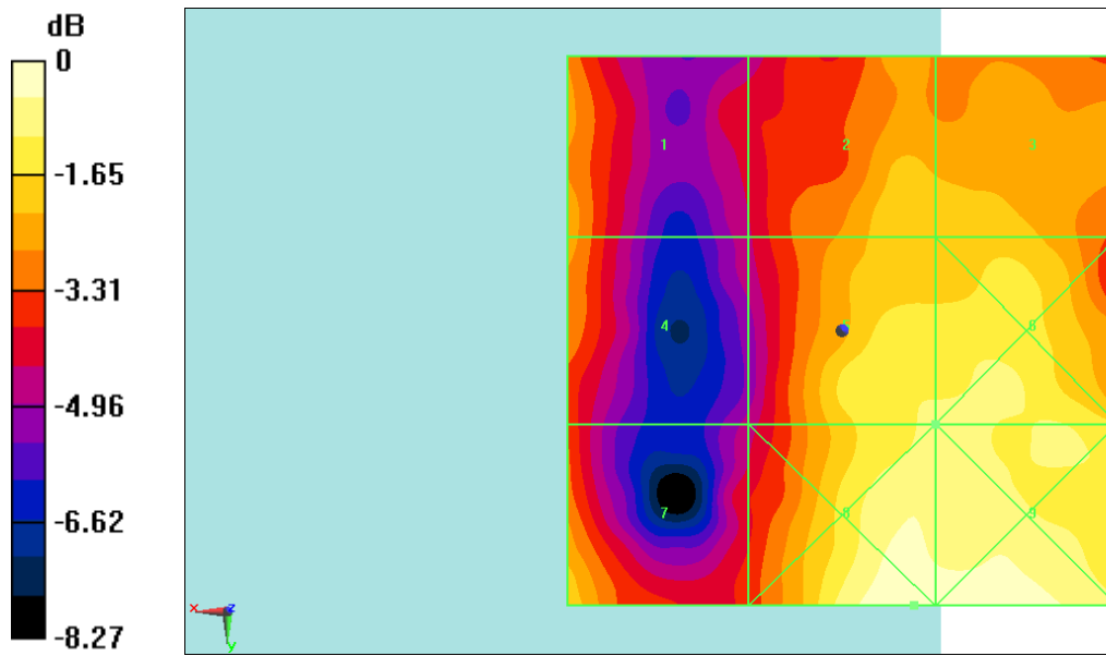
Fig B.41 HAC RF E-Field LTE Band41 Power Class 3 64QAM CH41490
