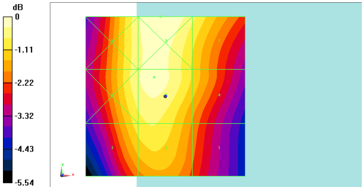
Fig B.2 HAC RF E-Field GSM 850 Middle
