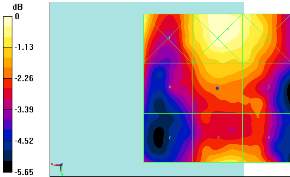
Fig B.27 HAC RF E-Field LTE Band41 Power Class 2 64QAM CH41055
