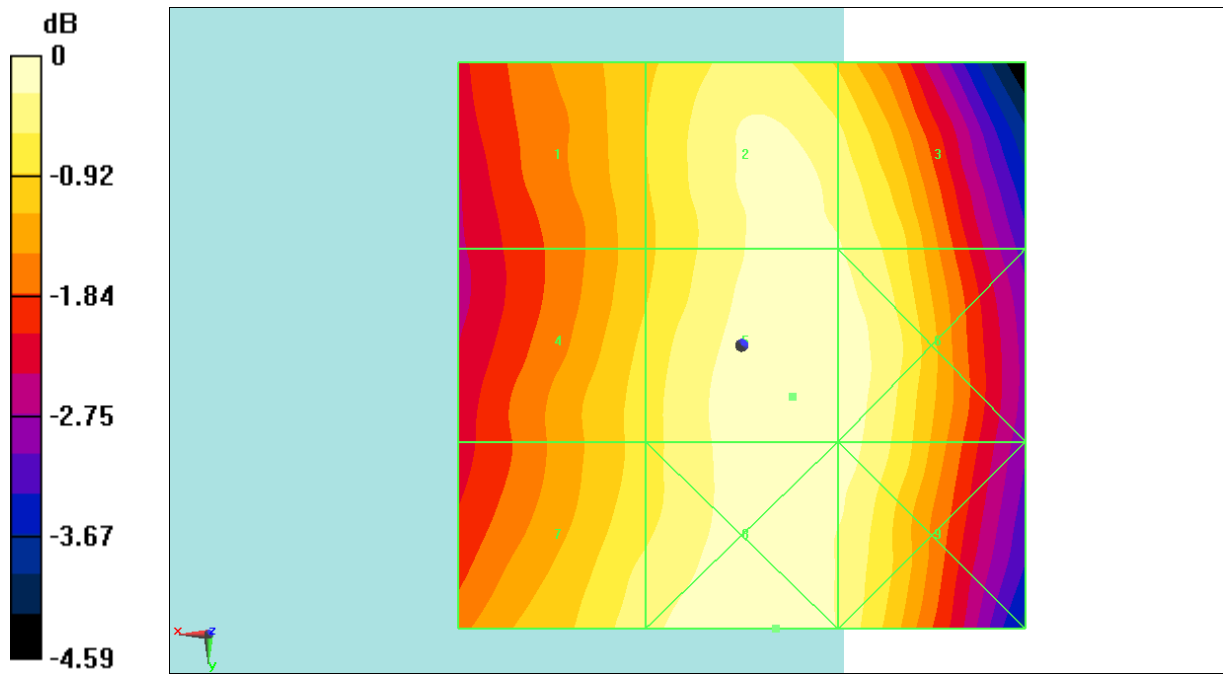
Fig B.14 HAC RF E-Field CDMA BC10 Middle
