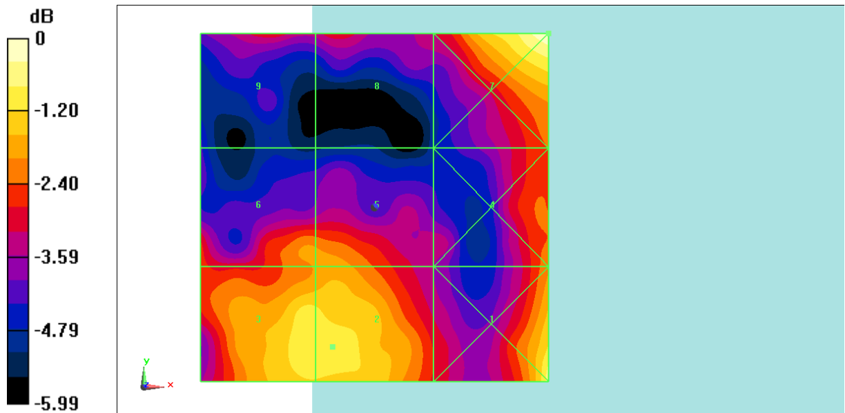
Fig B.33 HAC RF E-Field LTE Band41 Power Class 3 QPSK CH40620
