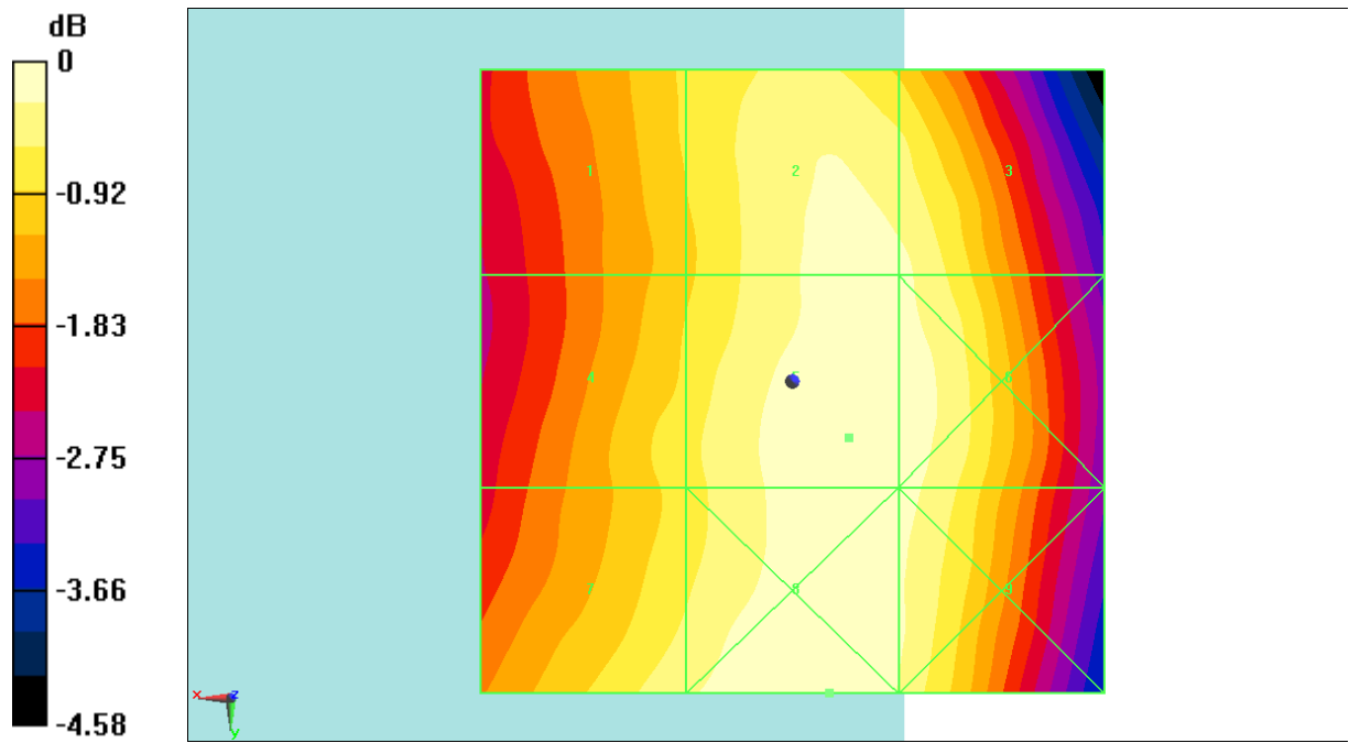
Fig B.13 HAC RF E-Field CDMA BC10 High
