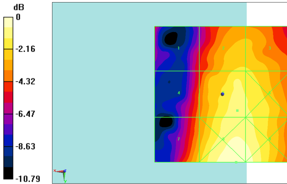
Fig B.16 HAC RF E-Field LTE Band41 Power Class 2 QPSK CH41490
