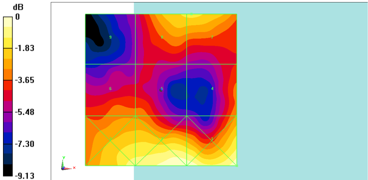
Fig B.32 HAC RF E-Field LTE Band41 Power Class 3 QPSK CH41055
