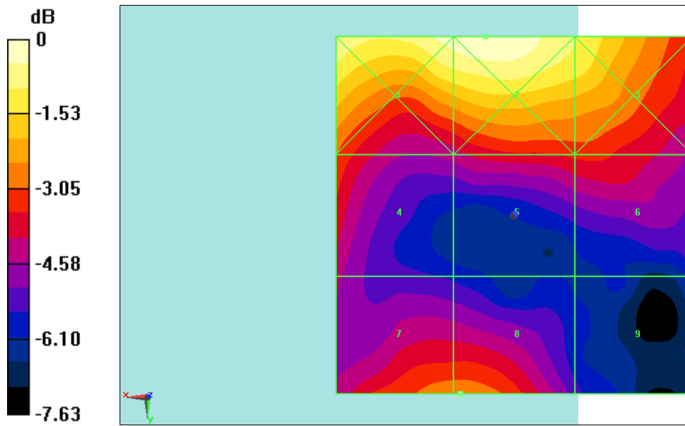
Fig B.19 HAC RF E-Field LTE Band41 Power Class 2 QPSK CH40185
