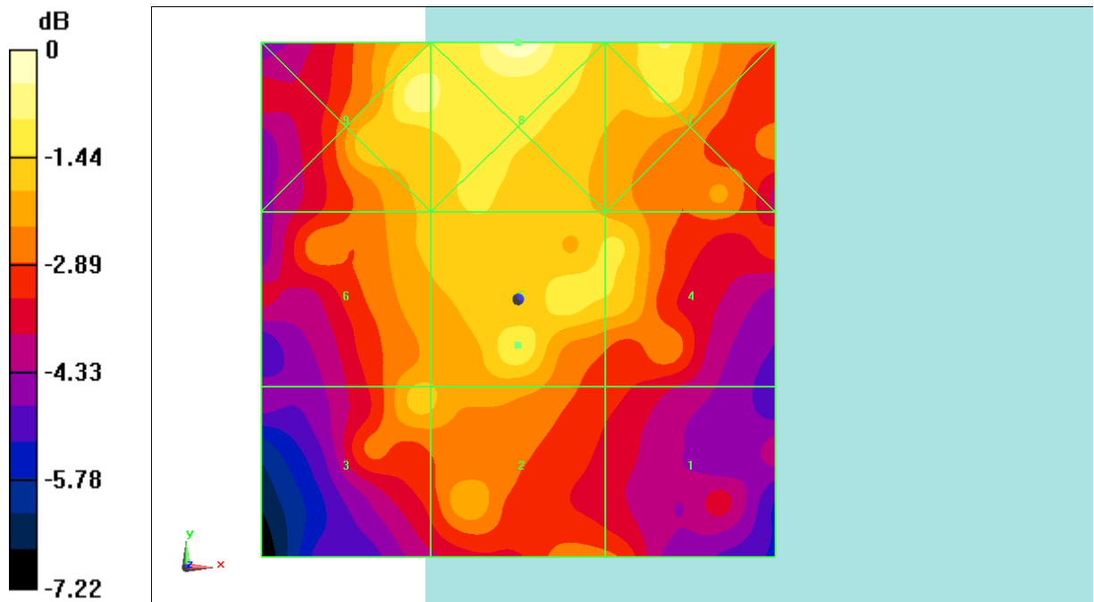
Fig B.9 HAC RF E-Field CDMA BC0 Low
