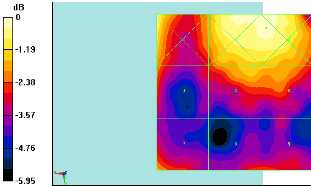
Fig B.37 HAC RF E-Field LTE Band41 Power Class 3 16QAM CH41055
