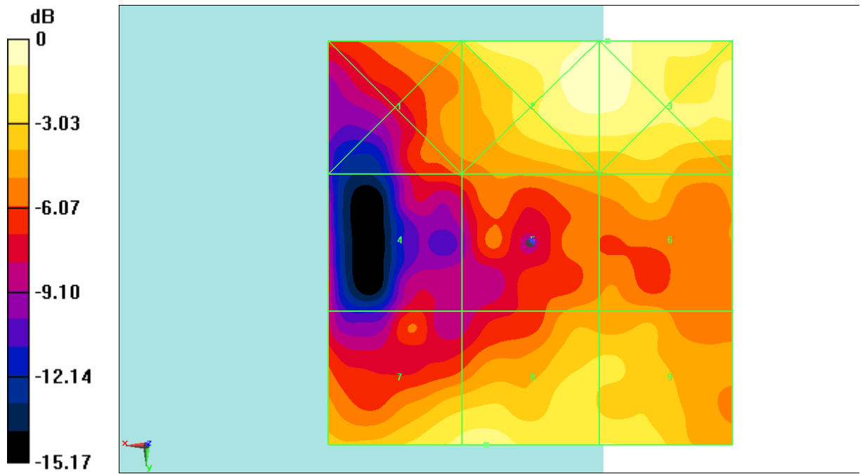
Fig B.11 HAC RF E-Field CDMA BC1 Middle
