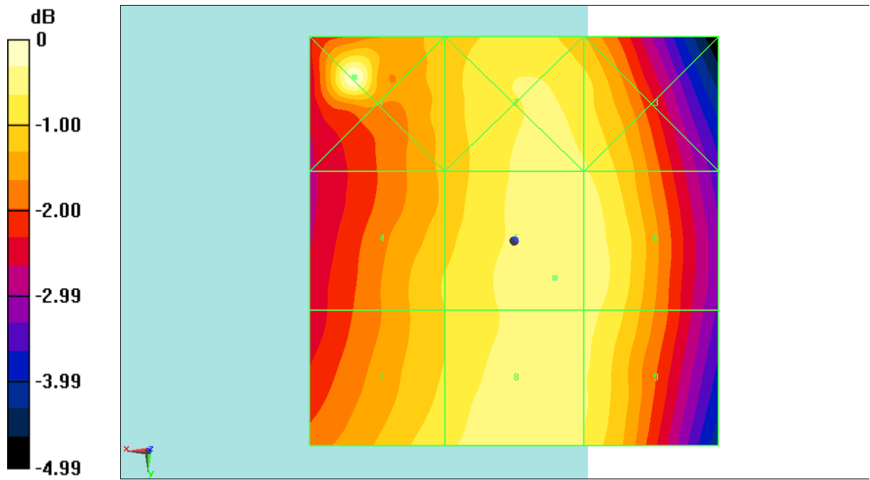
Fig B.15 HAC RF E-Field CDMA BC10 Low
