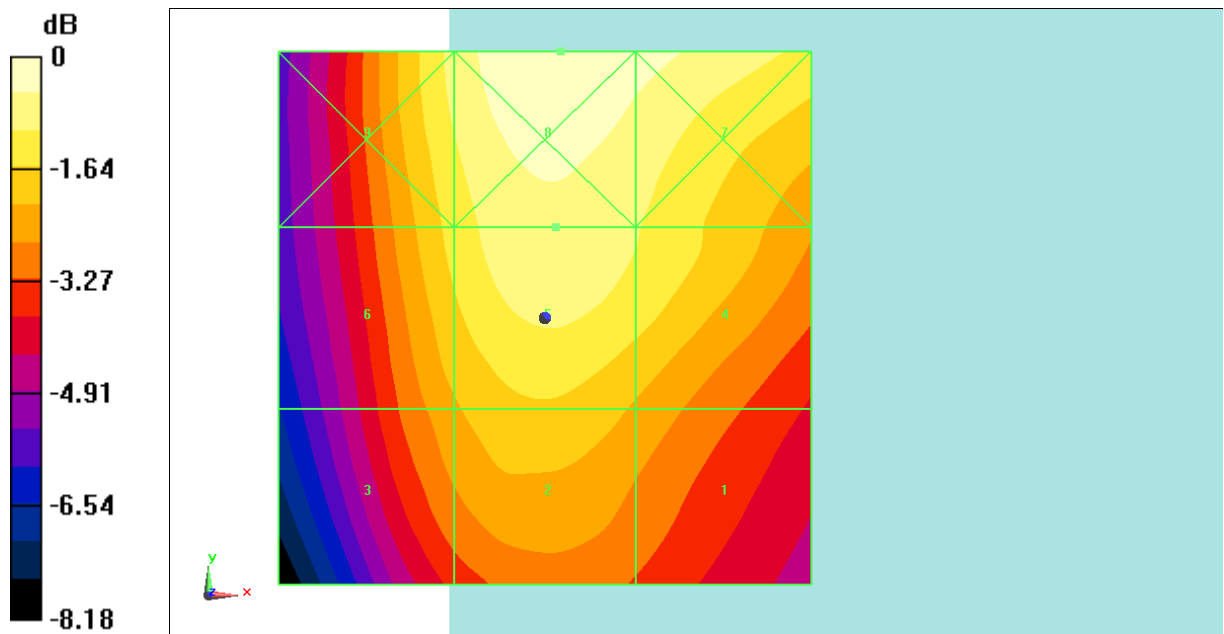
Fig B.1 HAC RF E-Field GSM 850 High
