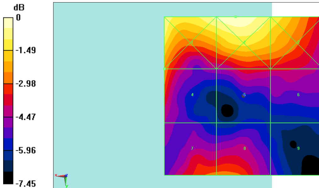
Fig B.23 HAC RF E-Field LTE Band41 Power Class 2 16QAM CH40620
