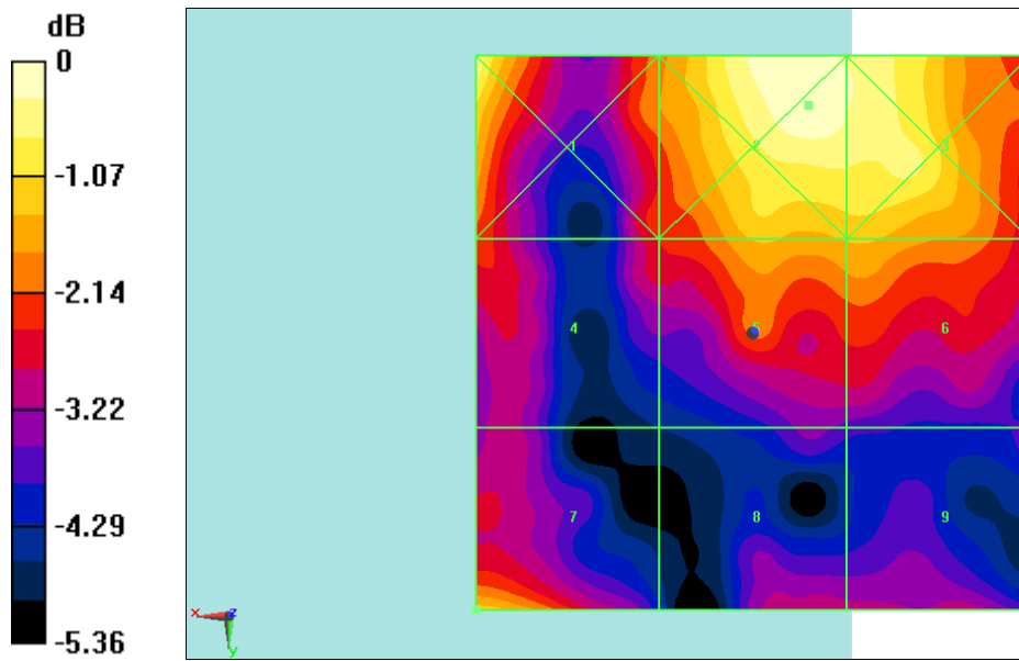
Fig B.36 HAC RF E-Field LTE Band41 Power Class 3 16QAM CH41490
