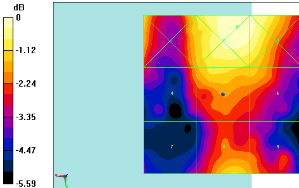
Fig B.28 HAC RF E-Field LTE Band41 Power Class 2 64QAM CH40620
