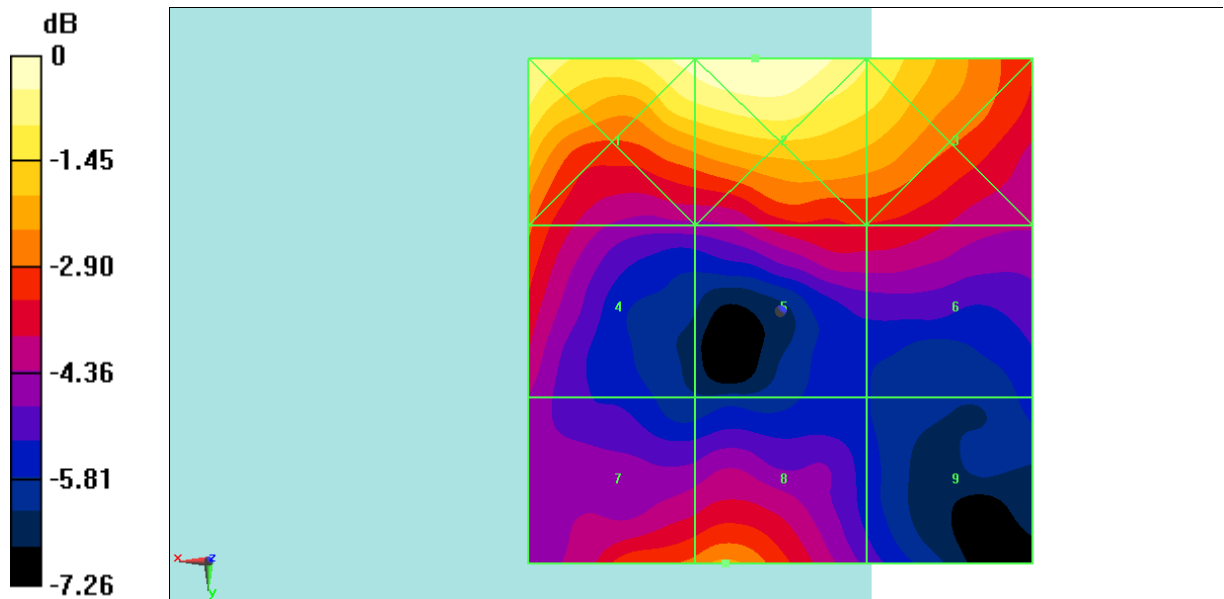
Fig B.24 HAC RF E-Field LTE Band41 Power Class 2 16QAM CH40185
