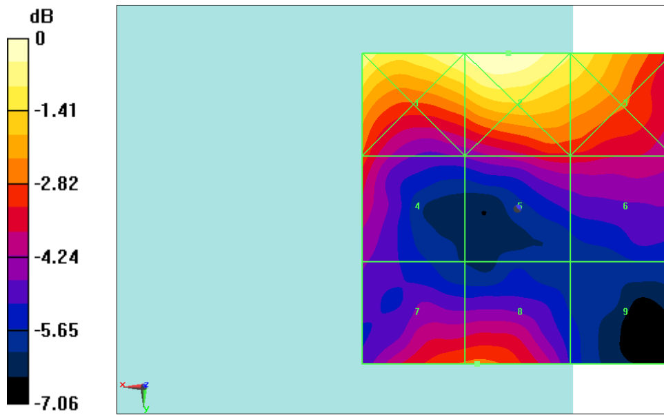
Fig B.17 HAC RF E-Field LTE Band41 Power Class 2 QPSK CH41055
