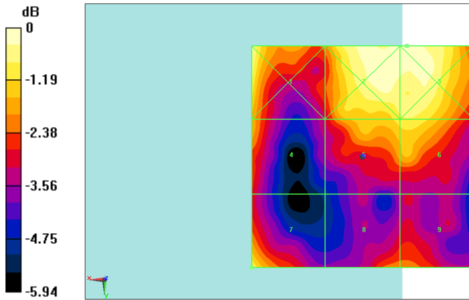
Fig B.38 HAC RF E-Field LTE Band41 Power Class 3 16QAM CH40620
